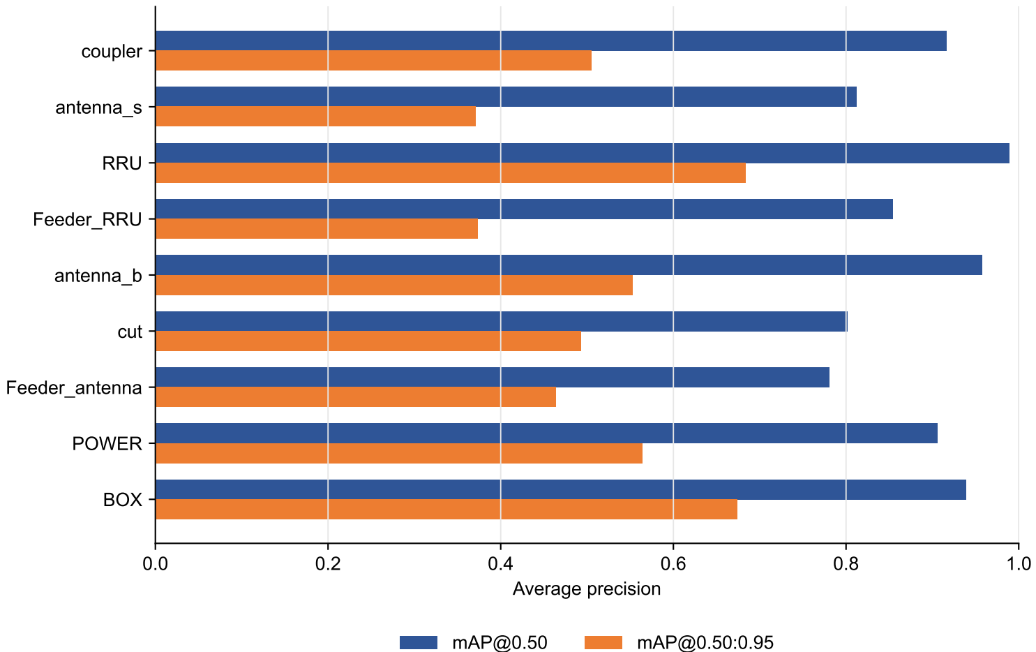
Per-class performance of the proposed fusion on the independent test set
