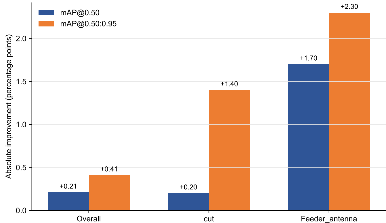
Contribution of the weak-class specialist on the development validation set
