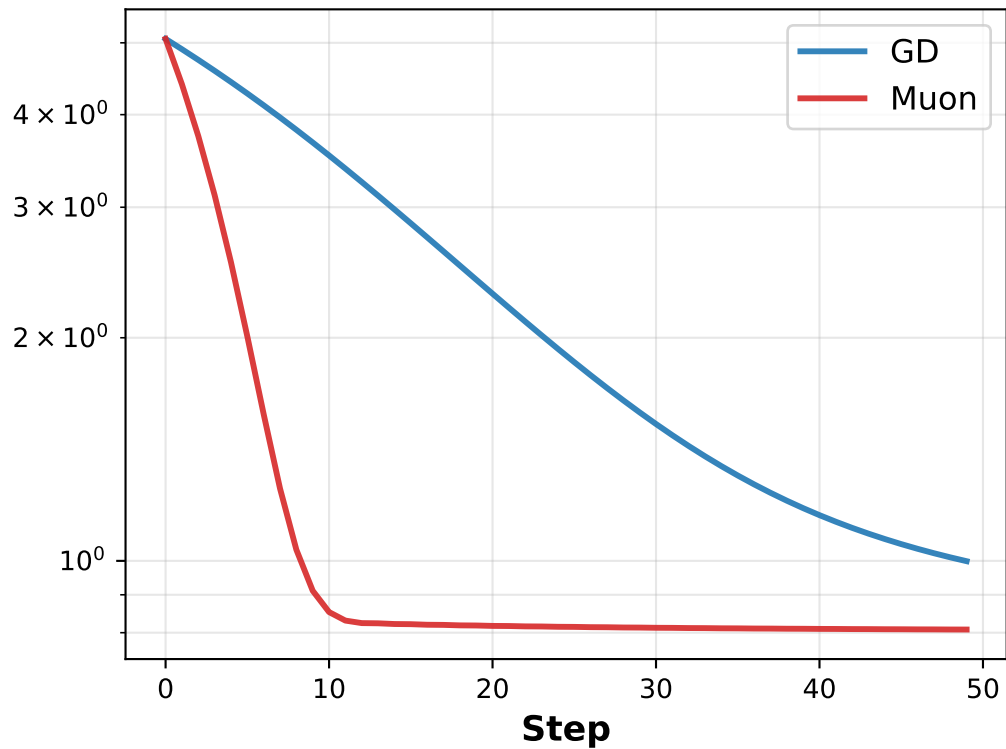
Loss (Random Init)
