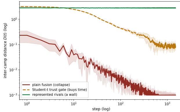
Fig. 4: Same setups, same evidence—only the representation differs (two camps, full contact, theory-laden streams; inter-camp distance D(t) , mean \pm s.d., 5 seeds, log-log). Plain fusion collapses (the theorem); the Student- t gate decays (time, bought and spent); represented rivals hold (a wall). Each architecture runs its own best memory setting (Appendix C).
