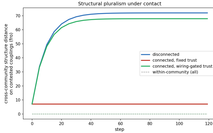
Fig. 2: The paper’s two results in one experiment (a structurally underdetermined world; cross-community distance on the contested couplings, mean \pm s.d., 5 seeds; dashed: within-community, \sim 0 throughout). Apart (blue): two crisply different wirings. Connected, default fusion (red): the pluralism never forms—10% of the disconnected divergence, the homogeneity effect (Result 1). Connected, wiring-reading trust (green, §3.5): 94% survives full contact (Result 2).
