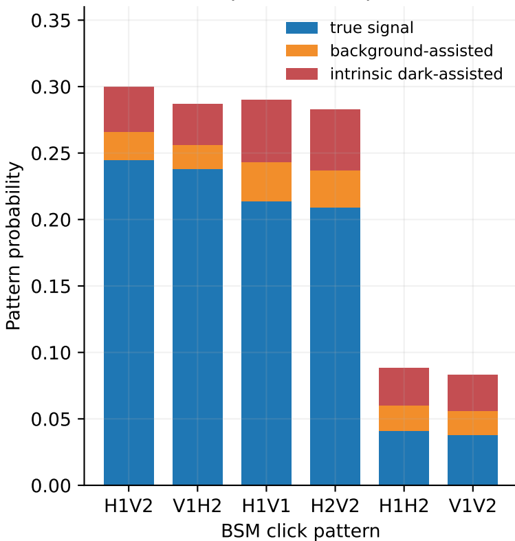
Herald-pattern composition
