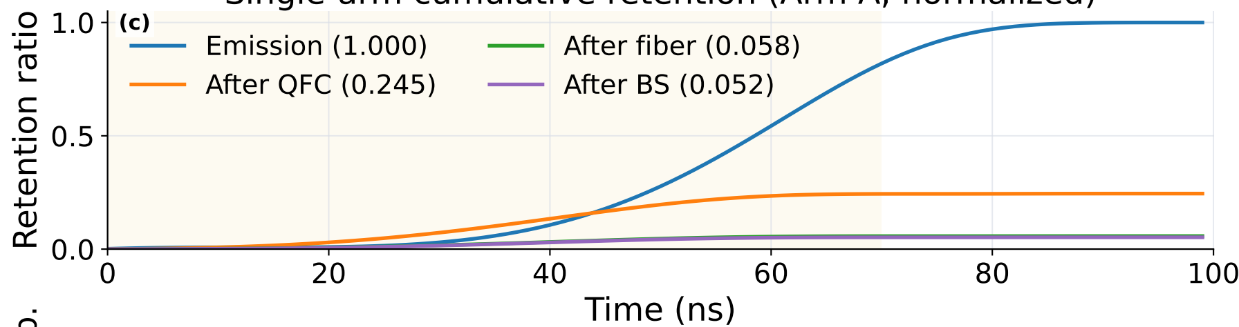
Stage-wise total photon probability
