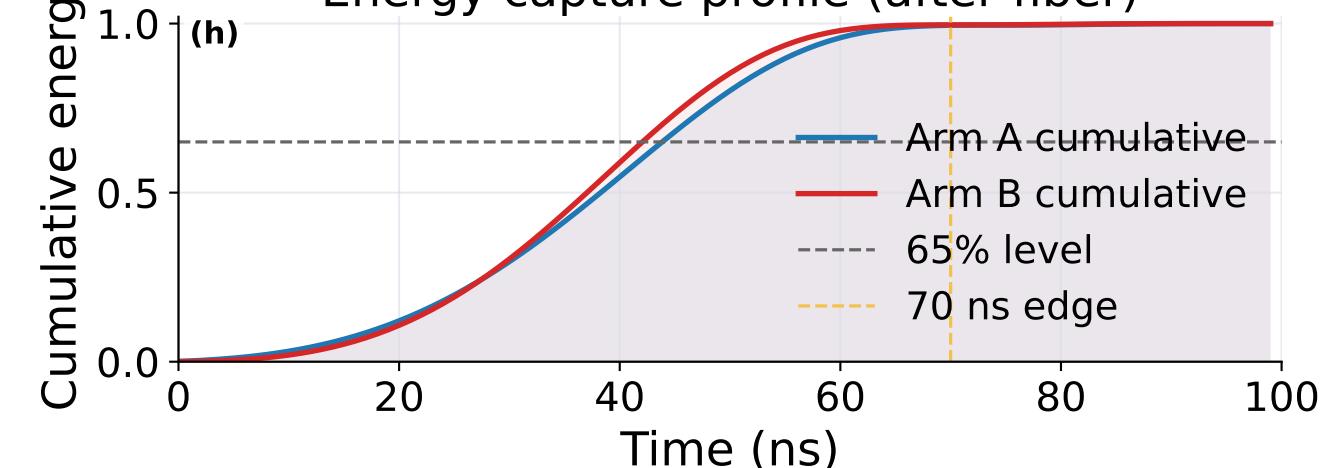
Energy capture profile (after fiber)
