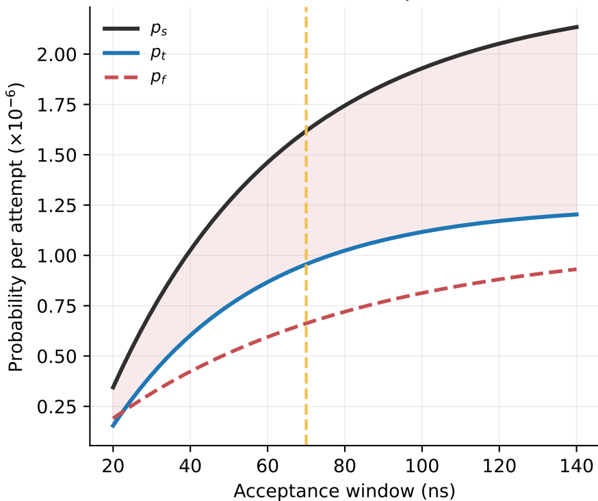
Herald-rate decomposition
