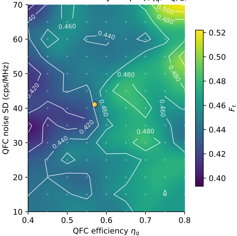
(a) Conditional fidelity map F_t(\eta_q, \sigma_{\text{QFC}})
