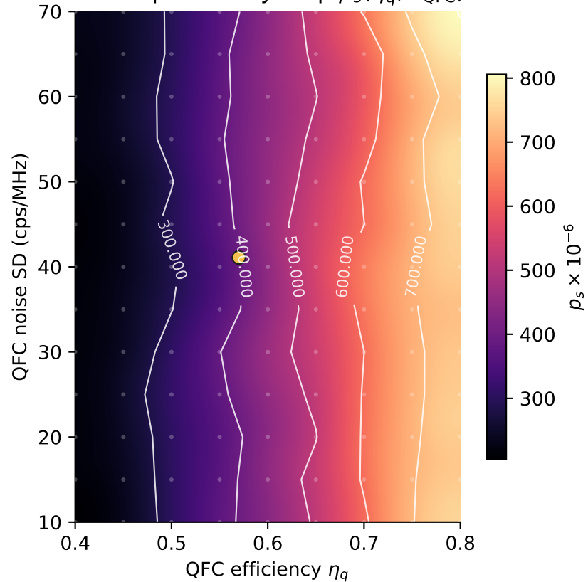
(b) Herald probability map p_s(\eta_q, \sigma_{\text{QFC}})
