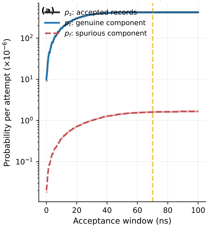
Rate decomposition versus acceptance window
