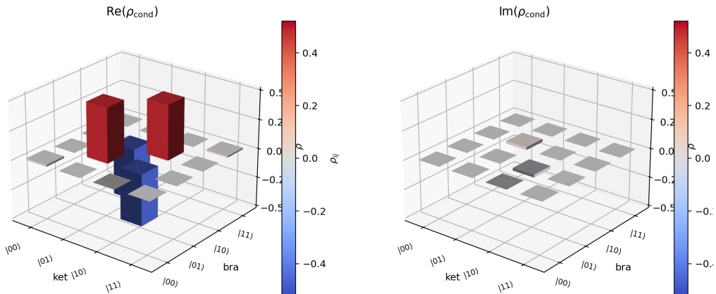
Heralded Bell-state density matrix (3D bars)
