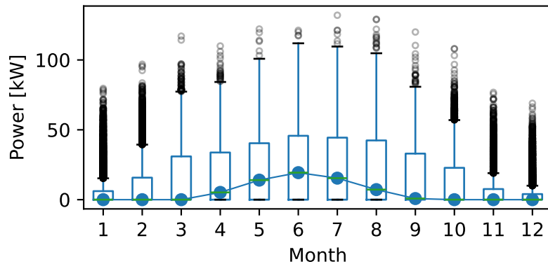
Power PV distribution by month
