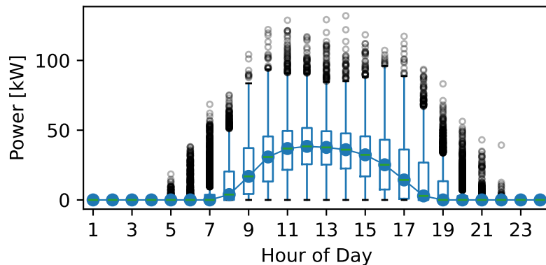
Power PV distribution by the hour of the day
