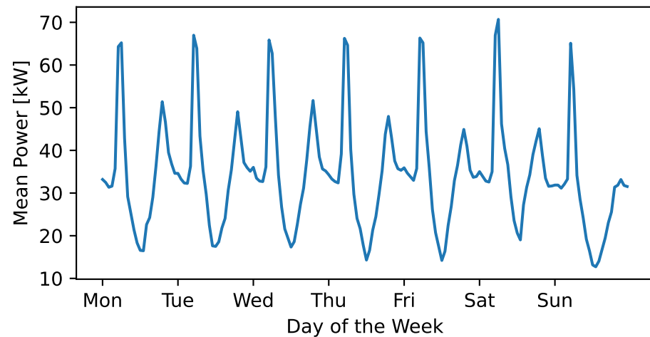
Mean Total power during week
