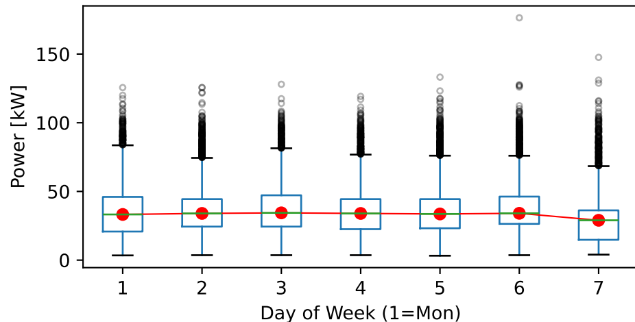
Mean Total power during week
