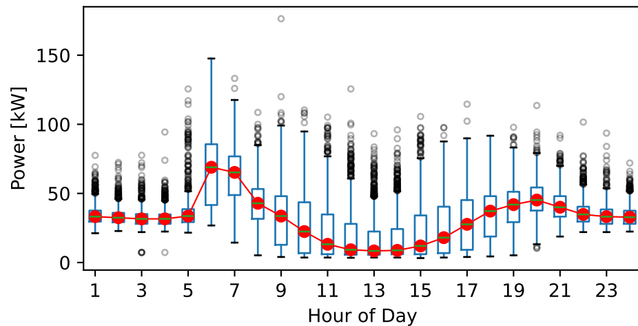
Power Total distribution by hour
