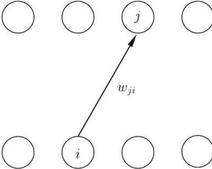
Fig. 9.19 Designation of the neurons and weights for the application of the backpropagation rule
