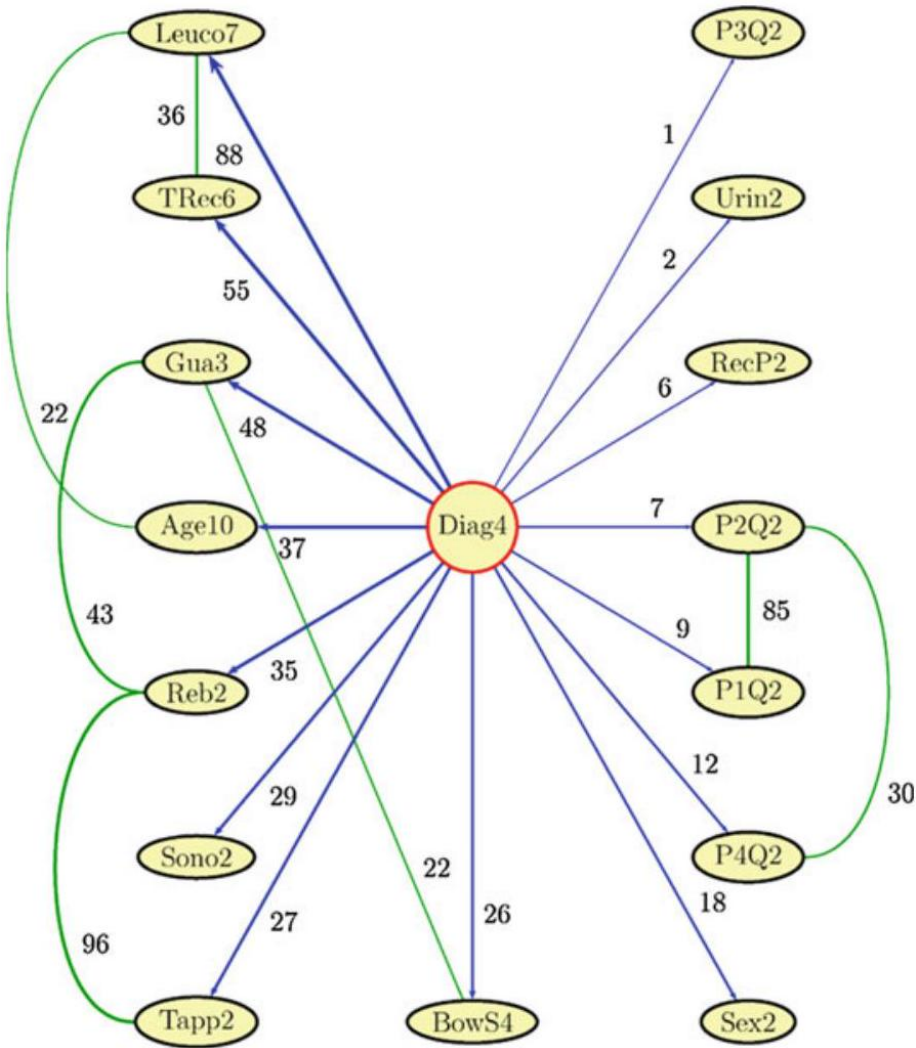
Fig. 7.8 Dependency graph computed from the database
