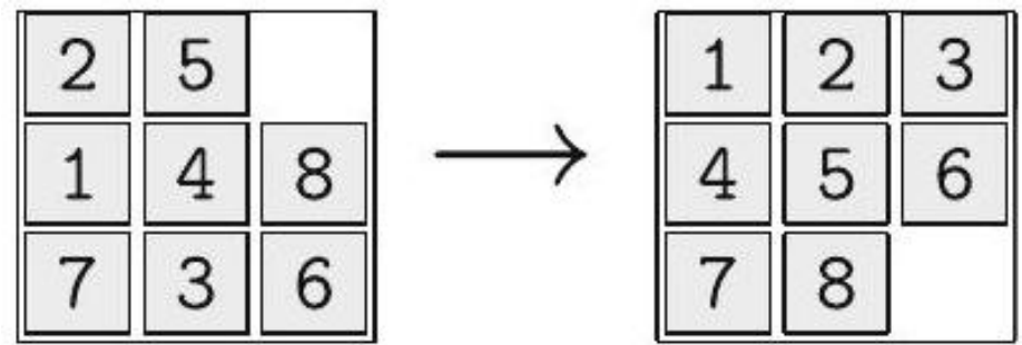
Fig. 6.2 Possible starting and goal states of the 8-puzzle
