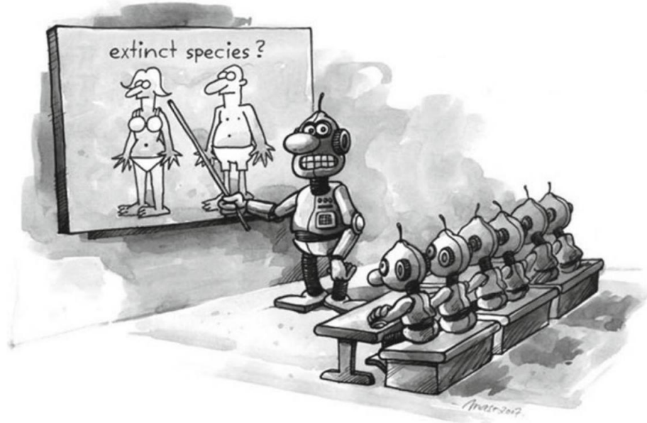
Fig. 8.1 Supervised learning ...
