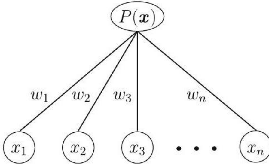
Fig. 8.9 Graphical representation of a perceptron as a two-layer neural network
