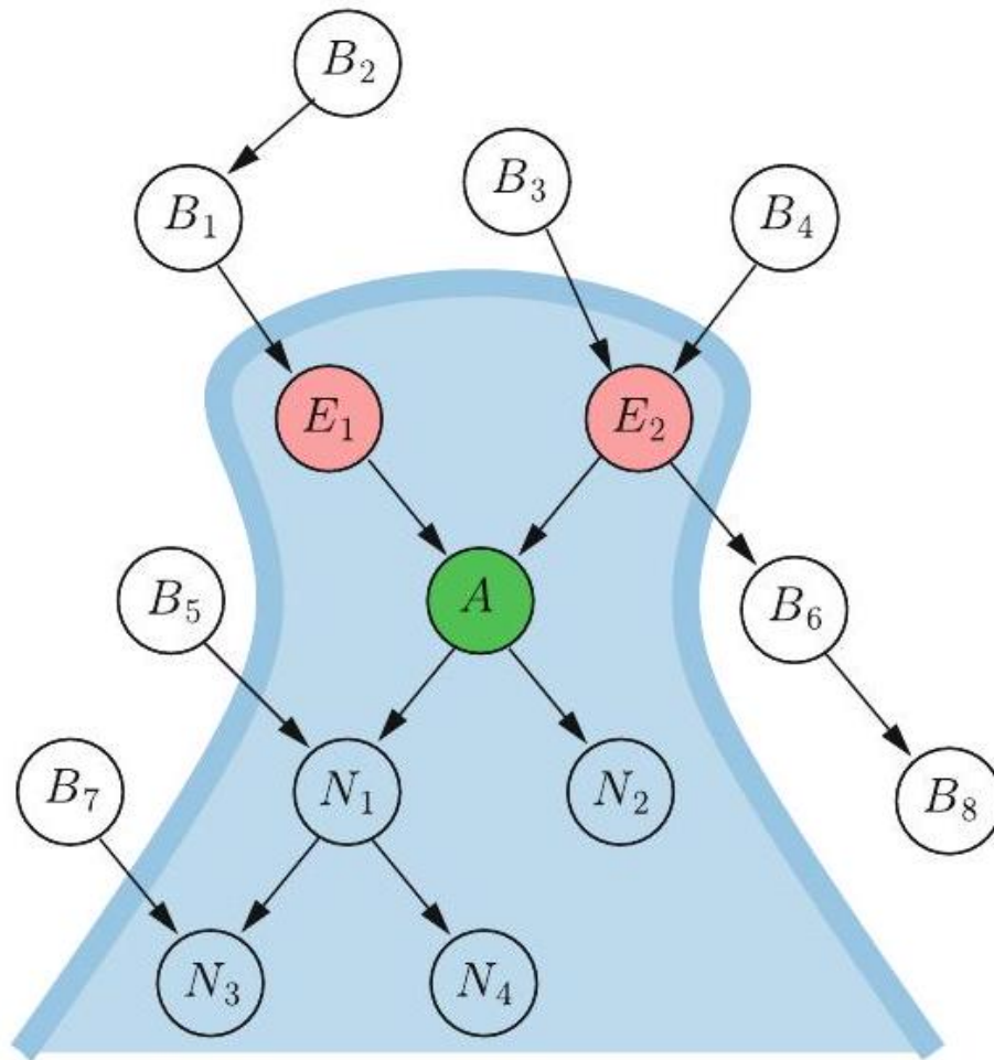
Fig. 7.17 Example of conditional independence in a Bayesian network. If the parent nodes E_1 and E_2 are given, then all non-successor nodes B_1, \dots, B_8 are independent of A
