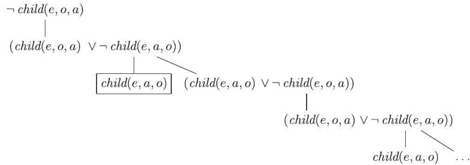
Fig. 5.2 PROLOG search tree for child(eve, oscar, anne)
