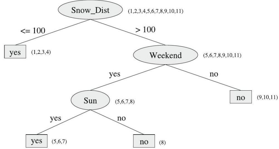
Fig. 8.23 Decision tree for the skiing classification problem. In the lists to the right of the nodes, the numbers of the corresponding training data are given. Notice that of the leaf nodes sunny = yes only two of the three examples are classified correctly
