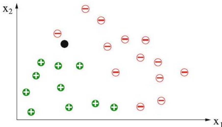
Fig. 8.13 In this example with negative and positive training examples, the nearest neighbor method groups the new point marked in black into the negative class
