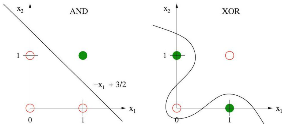
Fig. 8.8 The boolean function AND is linearly separable, but XOR is not ( \odot \triangleq true, \circ \triangleq false)
