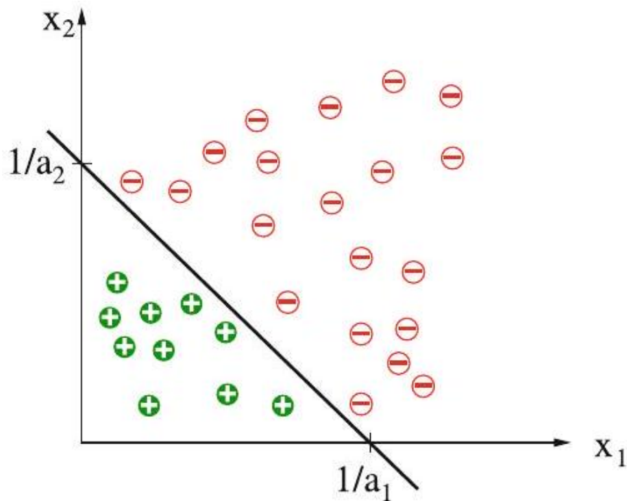
Fig. 8.7 A linearly separable two dimensional data set. The equation for the dividing straight line is a_1x_1 + a_2x_2 = 1
