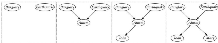
Fig. 7.15 Stepwise construction of the alarm network considering causality
