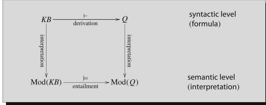
Fig. 2.1 Syntactic derivation and semantic entailment. \text{Mod}(X) represents the set of models of a formula X
