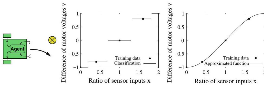
Fig. 8.18 The learning agent, which is supposed to avoid light (left), represented as a classifier (middle), and as an approximation (right)
