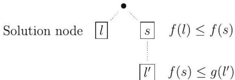
Fig. 6.17 The first solution node l found by A^* never has a higher cost than another arbitrary node l'
