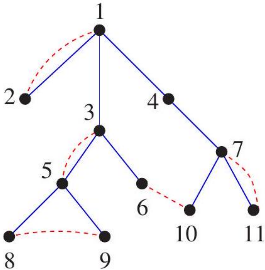
Figure 12.4: A depth-first traversal of a spanning tree, with the shortcut tour (left). The same DFS tree with a minimum weight matching between odd degree vertices, creating an Eulerian graph for the Christofides heuristic (right).
