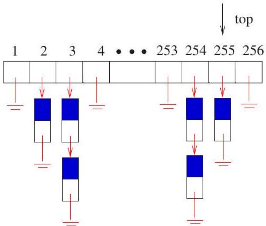
Figure 3.8: A bounded-height priority queue for triangle strips.
