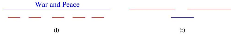
Figure 1.6: Bad instances for the (l) earliest job first and (r) shortest job first heuristics. The optimal solutions are in red.
