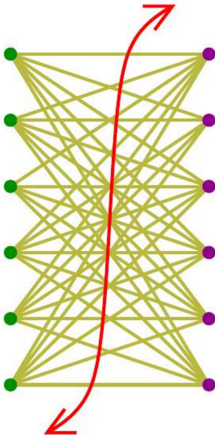
Figure 19.1: The maximum cut of a bipartite graph cuts all the edges.
