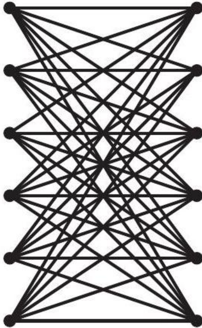
Figure 19.1: The maximum cut of a bipartite graph cuts all the edges.
