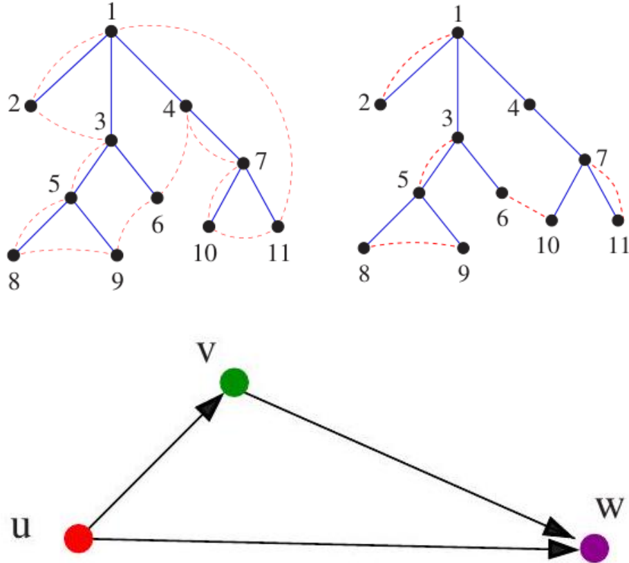
Figure 12.3: The triangle inequality , that d(u, w) \leq d(u, v) + d(v, w) , holds for distances defined between geometric points.
