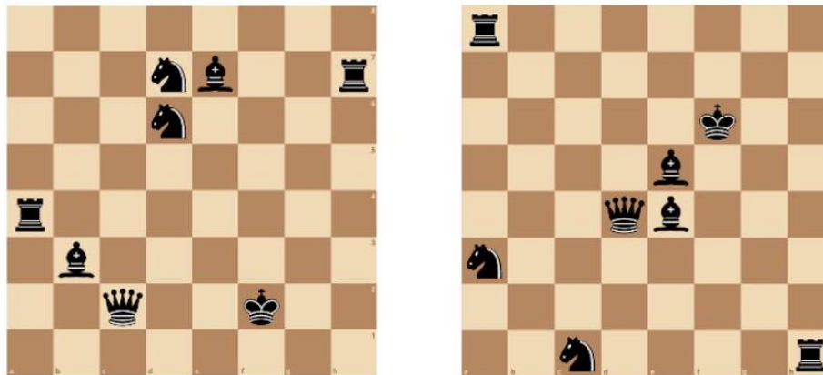
Figure 9.5: Configurations covering 63 but not 64 squares.
