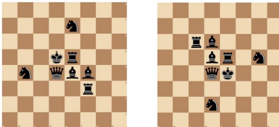
Figure 9.7: Weakly covering 64 squares.
