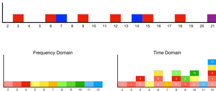
Figure 12.15: Transforming the integers from the frequency to the time domain computes the number of factors for each integer.
