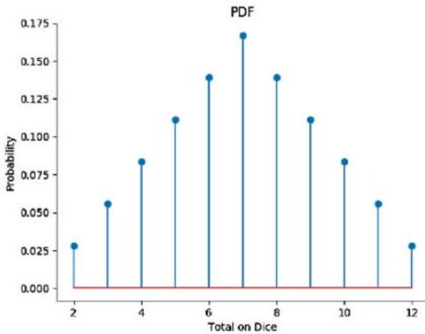
Figure 6.2: The probability density function (pdf) of the sum of two dice contains exactly the same information as the cumulative density function (cdf), but looks very different.
