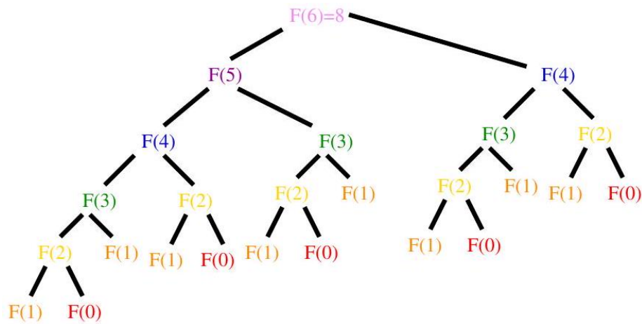
Figure 10.1: The recursion tree for computing Fibonacci numbers.
