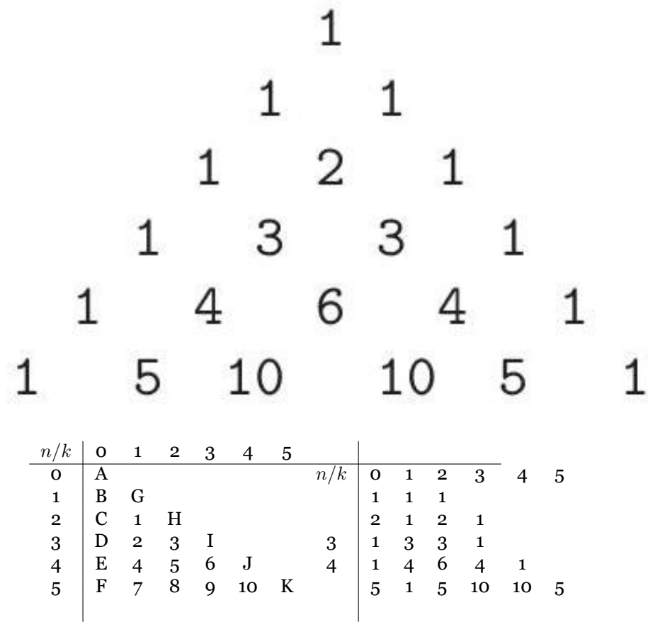
Figure 10.3: Evaluation order for binomial_coefficient at M[5,4] (left). The initialization conditions are labeled A – K and recurrence evaluations labeled 1 – 10. The matrix contents after evaluation are shown on the right.
