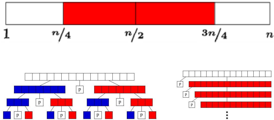
Figure 4.6: The best-case (left) and worst-case (right) recursion trees for quicksort. The left partition is in blue and the right partition in red.
