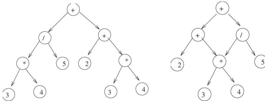
Figure 7.17: Expression 2 + 3 * 4 + (3 * 4) / 5 as a tree and a DAG
