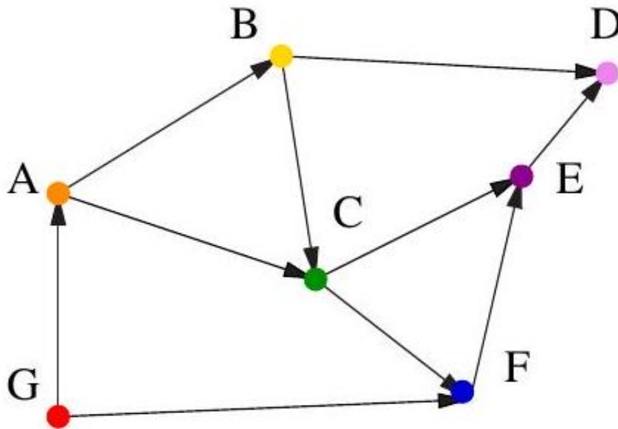
Figure 7.15: A DAG with only one topological sort ( G, A, B, C, F, E, D )
