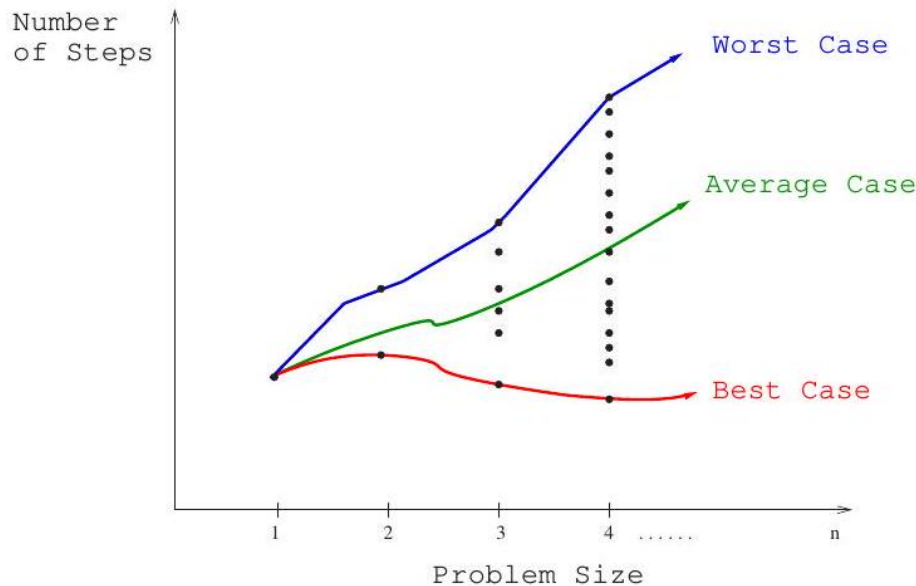
Figure 2.1: Best-case, worst-case, and average-case complexity.
