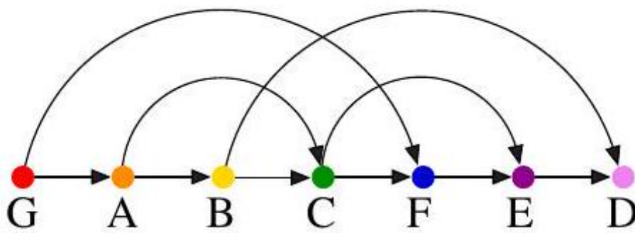
Figure 7.15: A DAG with only one topological sort ( G, A, B, C, F, E, D )
