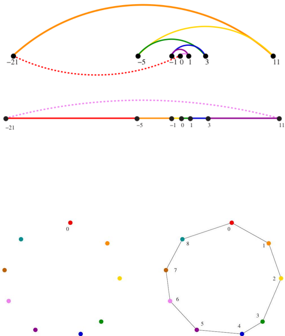
Figure 1.2: A good instance for the nearest-neighbor heuristic. The rainbow coloring (red to violet) reflects the order of incorporation.
