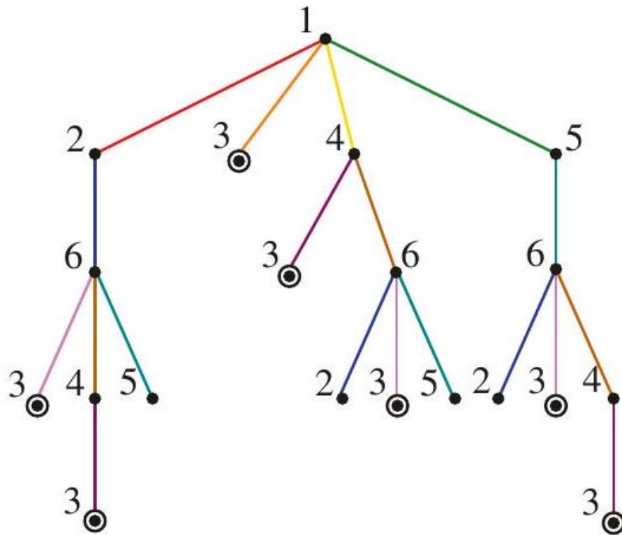
Figure 9.2: Search tree (right) enumerating all simple s - t paths in the given graph (left). The color of a search tree edge reflects the color of the corresponding graph edge.
