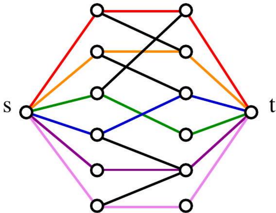
Figure 8.10: Bipartite graph with a maximum matching (left). The corresponding network flow instance highlighting the maximum s-t flow (right).
