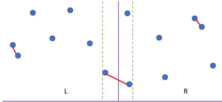
Figure 5.4: The closest pair of points in two dimensions either lie to the left of center, to the right, or in a thin strip straddling the center.
