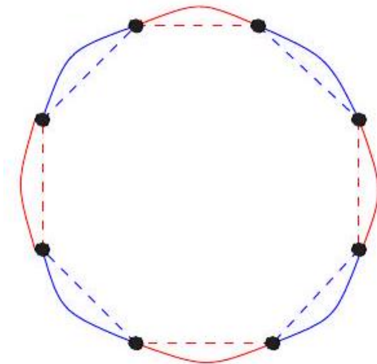
Figure 12.5: Any TSP tour in a graph with an even number of vertices that observes the triangle inequality can be partitioned into red and blue matchings, one of which must be at most half the cost of the tour.
