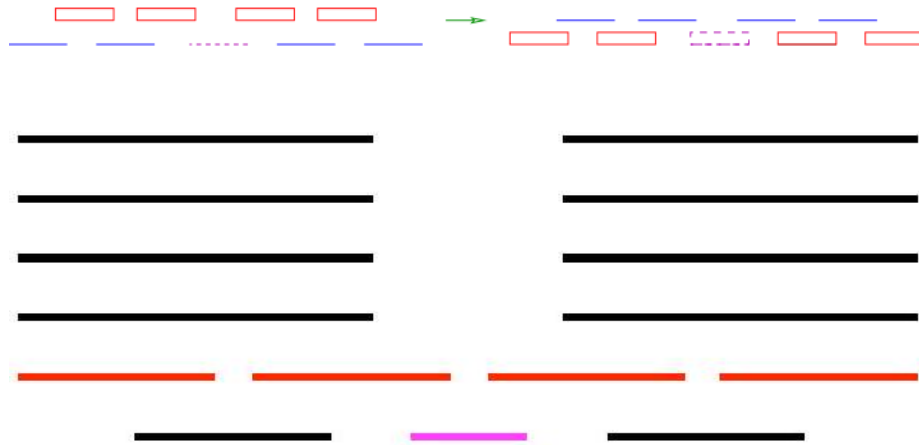
Figure 1.7: Counter-example to the greedy heuristic for movie star scheduling. Picking the pink interval, which intersects the fewest others, blocks us from the optimal solution (the four red intervals).
