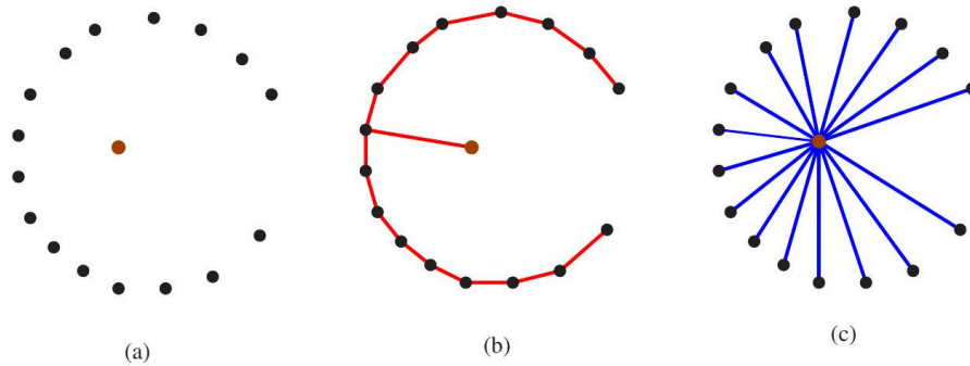
Figure 8.1: (a) The distances between points define a complete weighted graph, (b) its minimum spanning tree , and (c) the shortest path from center tree.
