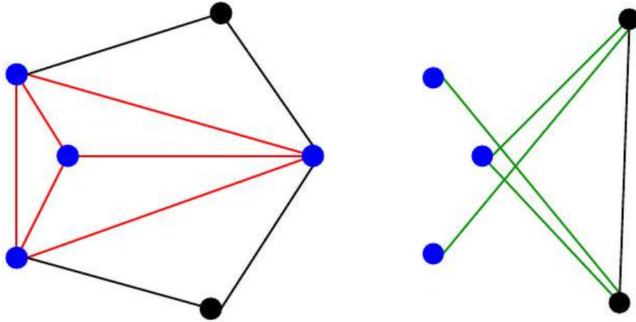
Figure 11.6: A small graph with a four-vertex clique (left), with the corresponding independent set in black forming a two-vertex clique in the graph's complement (right).
