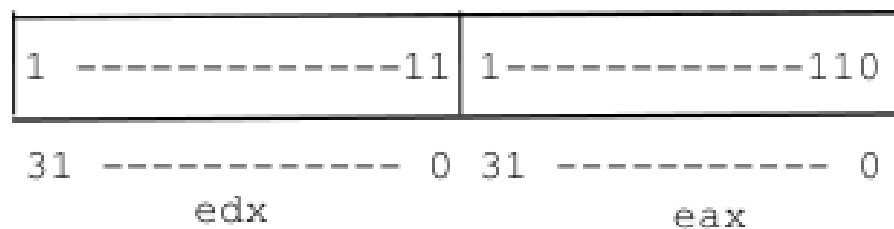
Fig. 3.2 The edx:eax registers after execution of the imul instruction
