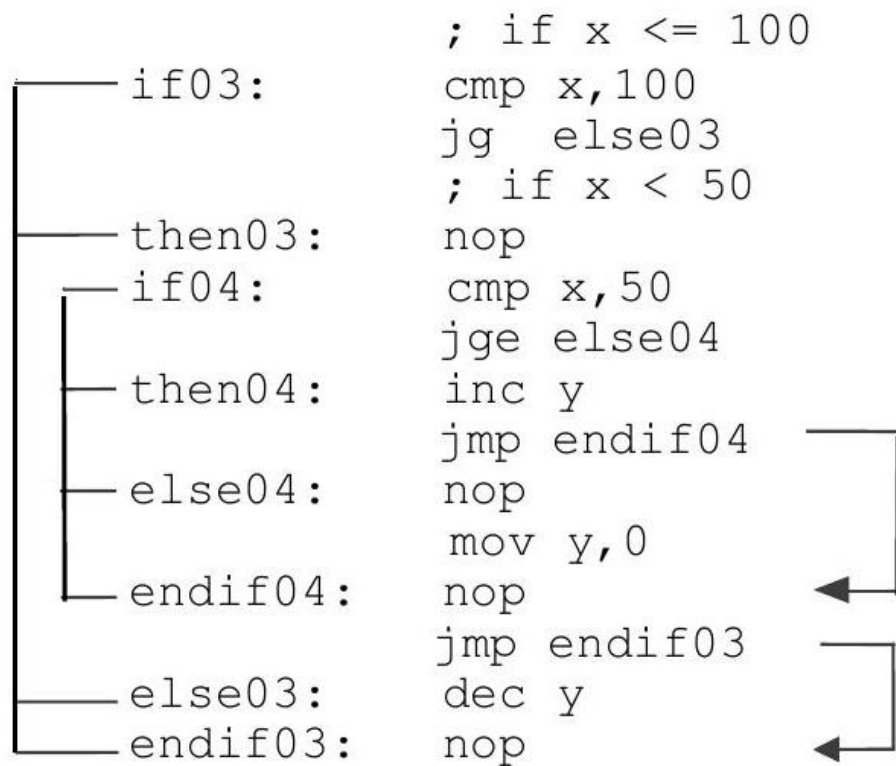
Fig. 4.2 If-then-if structure with double jump
