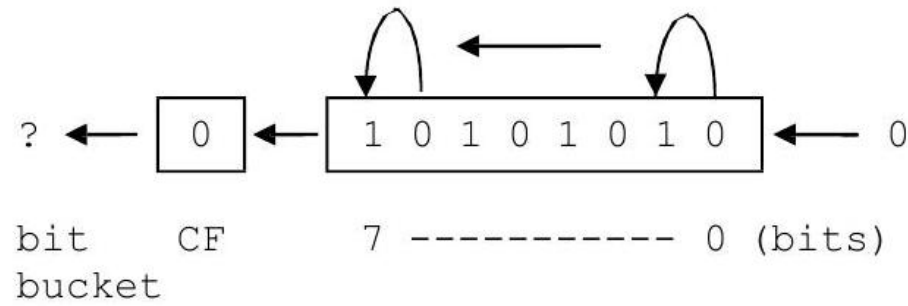
Fig. 6.4 Results in al register after sal instruction
