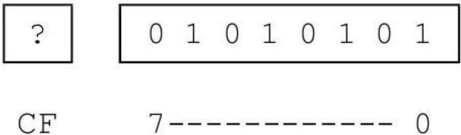
Fig. 6.6 Initial contents of al Register
