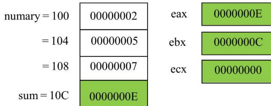
Fig. 8.4 Using ebx for array processing
