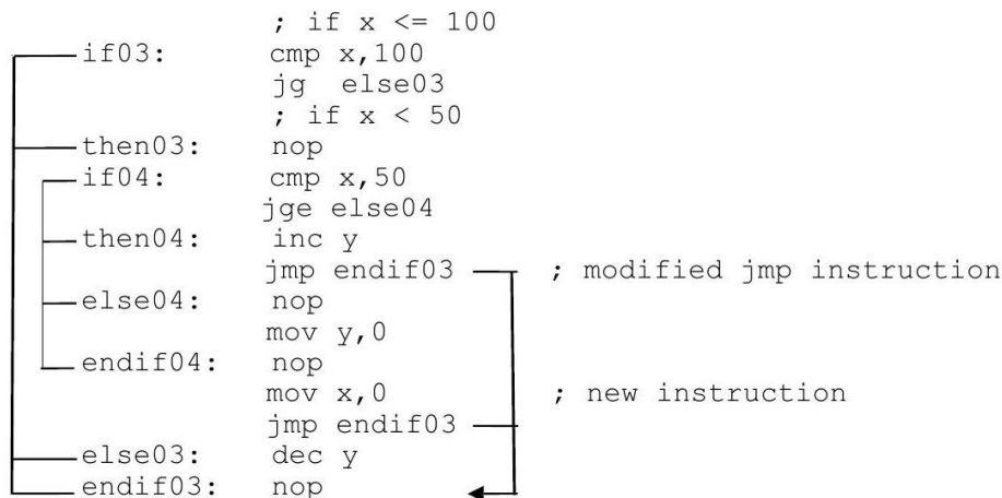
Fig. 4.3 If-then-if structure with inadvisable jump
