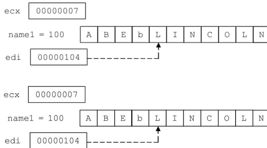
Fig. 9.2 Using repne scasb
