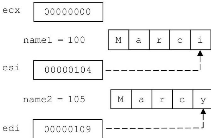
Fig.9.9 Using repe cmpsb and backing up one character
