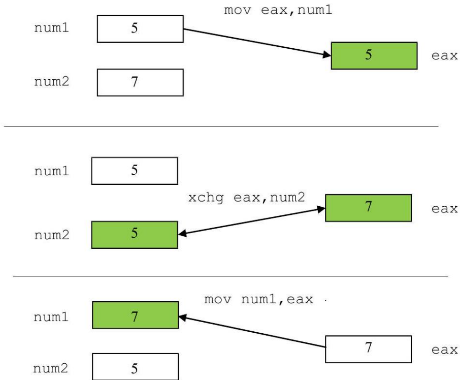
Fig. 6.10 Swapping using the xchg instruction
