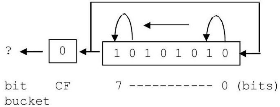
Fig. 6.6 Initial contents of al Register
