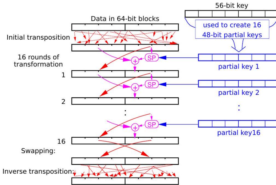
Fig. 4.8 Operation of the Digital Encryption Standard (DES)
