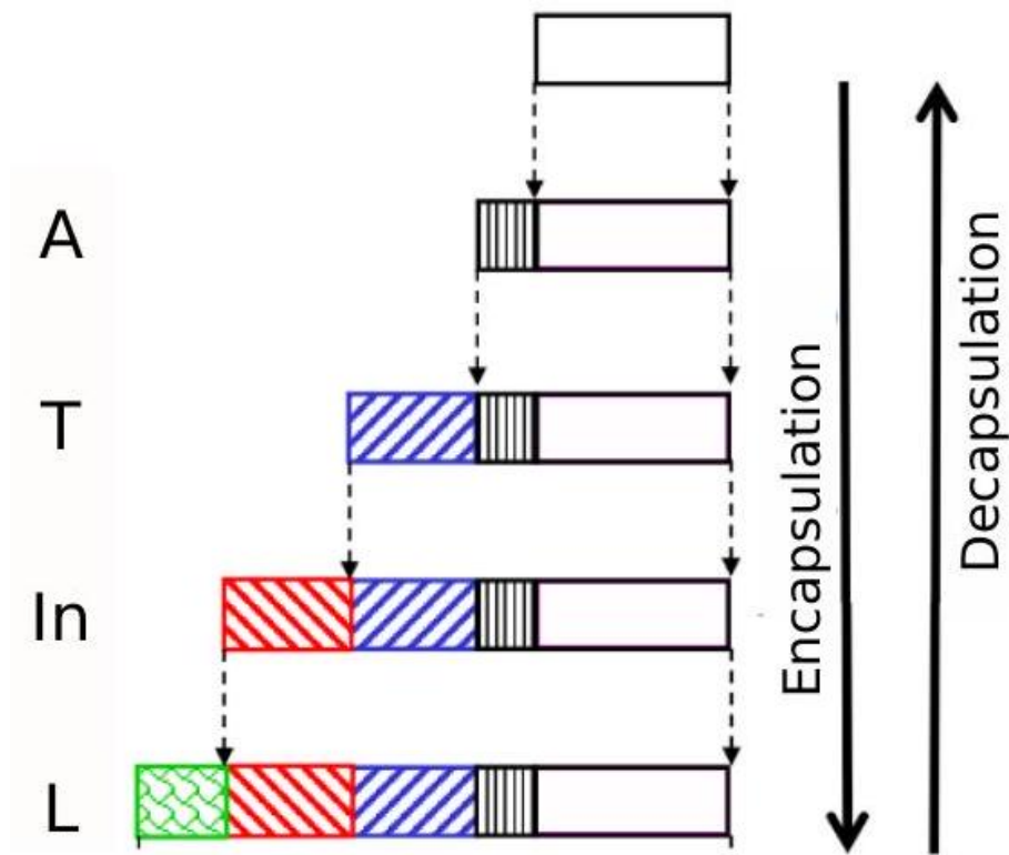
Fig. 8.1 Embedding of PDUs in a layered architecture
