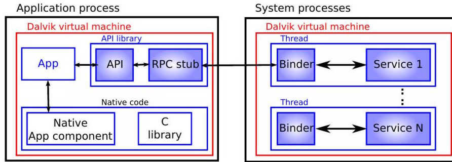
Fig. 9.21 Software architecture in Android (after citefelt2011android)
