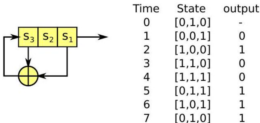
Fig. 4.14 Structure and operation of a simple LFSR
