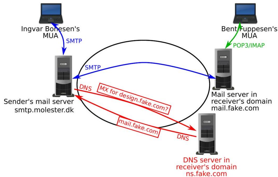
Fig. 7.3 Mail relaying in the Internet
