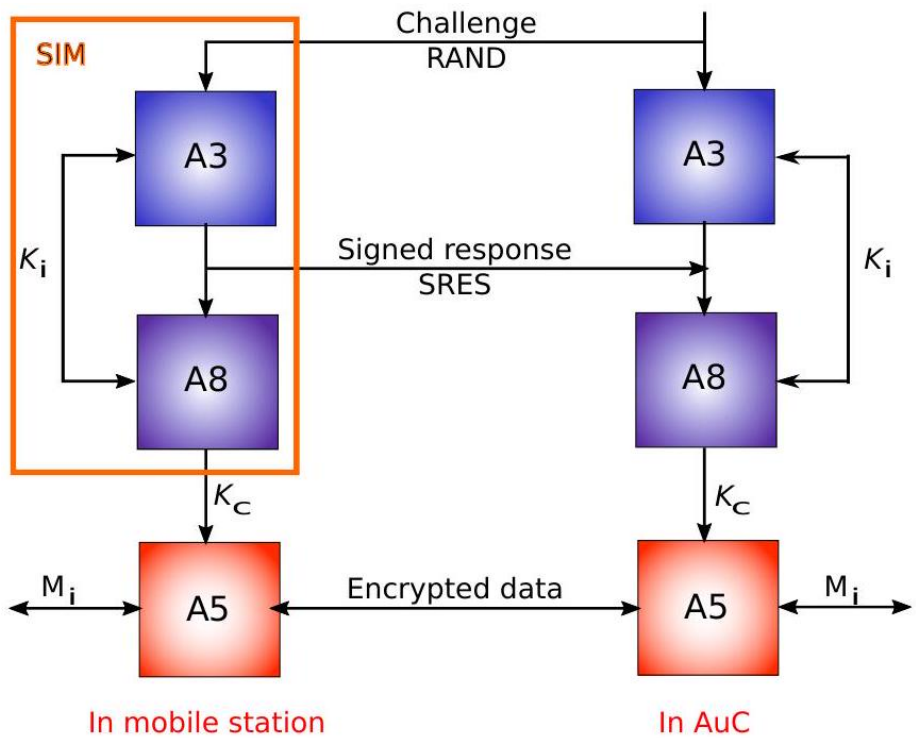
Fig. 8.26 Cryptographic functions in GSM
