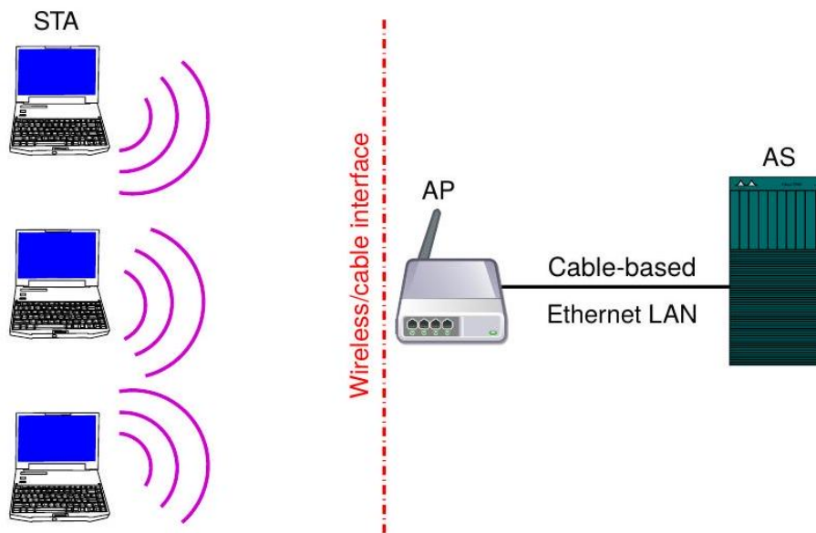
Fig. 8.25 Authentication with the use of 802.1X
