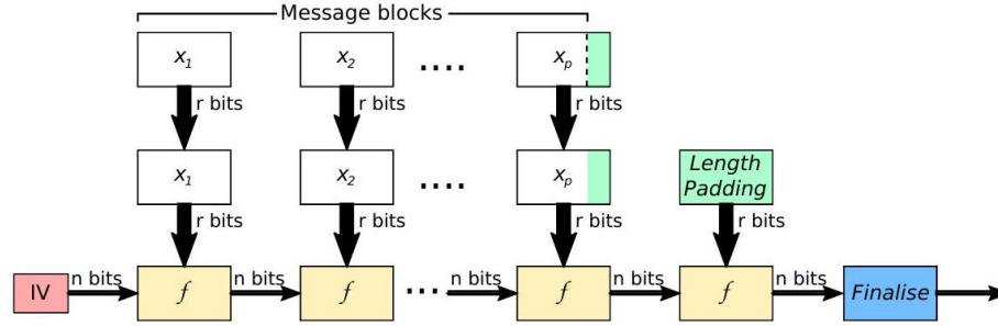
Fig. 5.3 Principle of operation of a cryptographic hash function based on the Merkle-Damgaard construction
