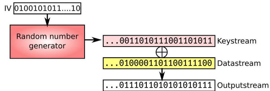
Fig. 4.13 Operation of a stream cipher.
