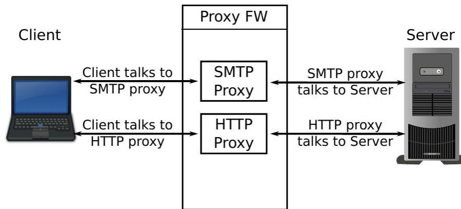
Fig. 8.19 An application proxy firewall
