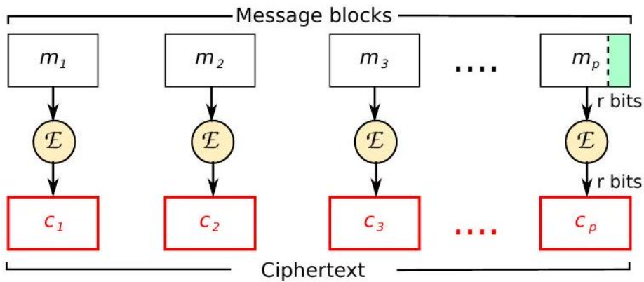
Fig. 4.9 Operation of DES in ECB mode
