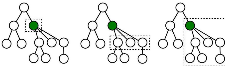
Fig. 10.10 Scope in LDAP searches. The filled circle is the chosen base object. From left to right : base, one and sub.
