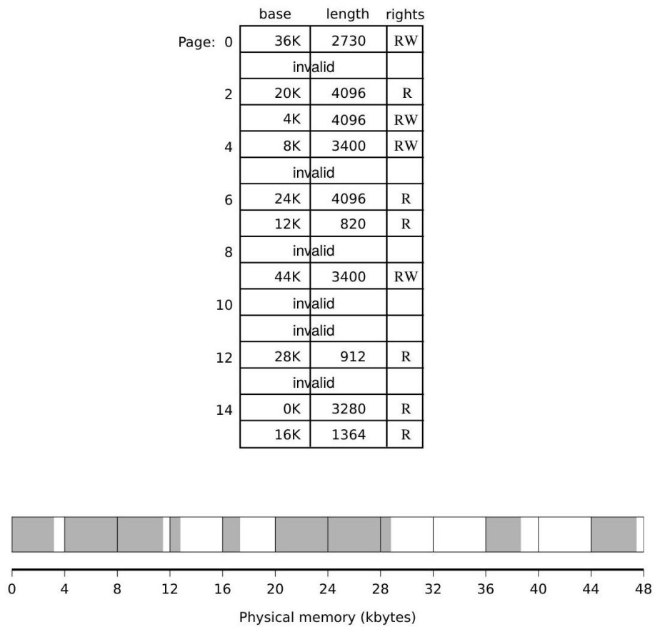
Fig. 9.19 A page table and the allocation of space in the memory which it corresponds to
