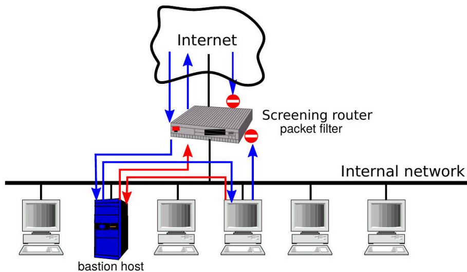
Fig. 8.22 A screened host setup
