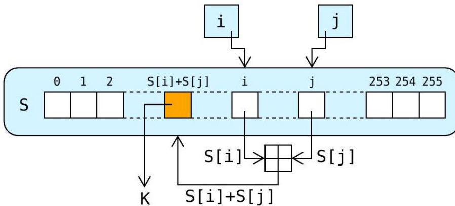
Fig. 4.16 The lookup step in RC4's keystream generator. (Diagram : Wikimedia Commons I)
