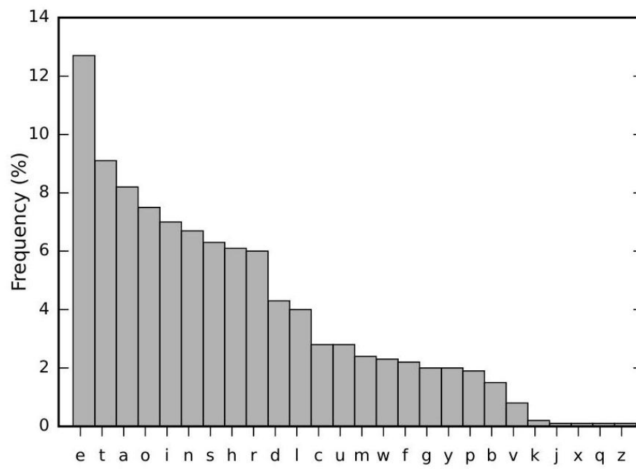
Fig. 4.3 Relative frequencies for the use of letters from the English alphabet in English texts. (Data source : citelewand2000cryptological)
