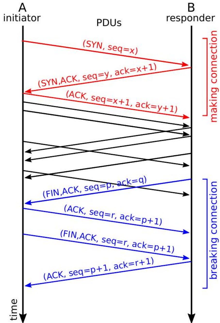
Fig. 6.11 Exchange of PDUs via a TCP connection Only the relevant components in each PDU are shown.
