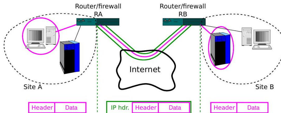
Fig. 8.10 Site-to-site tunneling
