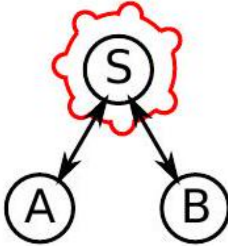
Fig. 5.10 Authentication via a trustworthy and wellprotected authentication server
