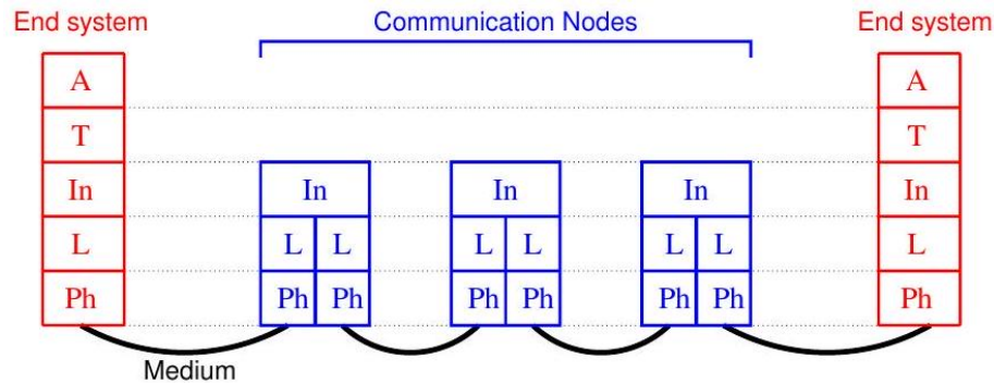
Fig. 6.12 End systems and communication nodes
