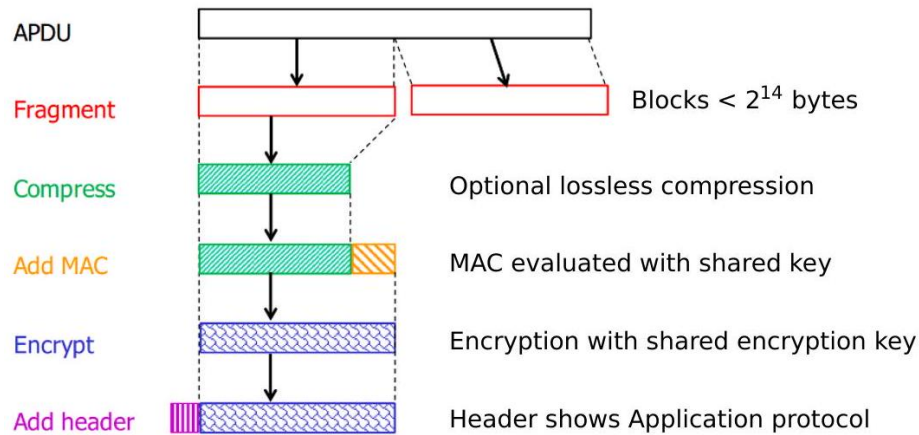
Fig. 8.15 Treatment of APDUs in SSL/TLS's Record protocol
