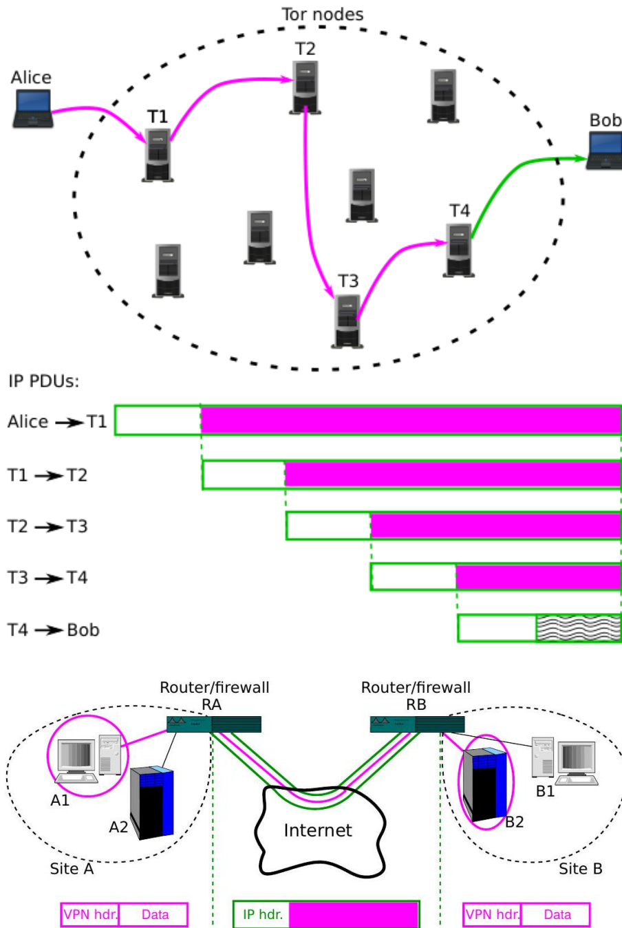
Fig. 8.11 Secure site-to-site tunneling in a VPN
