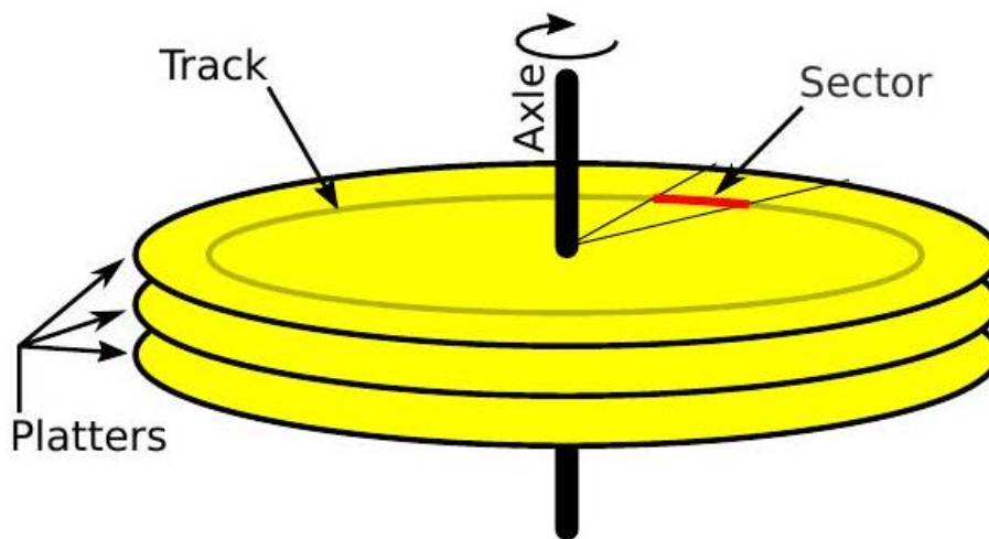
Fig. A. 3 A classical HDD. Left : Schematic structure.
