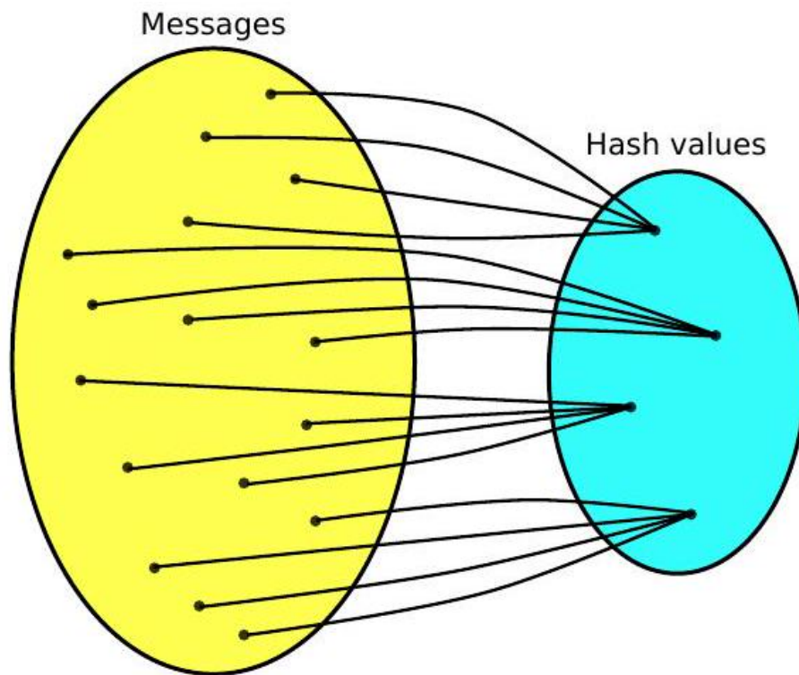
Fig. 5.2 Principle of a cryptographic hash function A potentially large set of messages is mapped onto a much smaller set of possible hash values. The curved lines indicate which hash value will be evaluated for each individual message.
