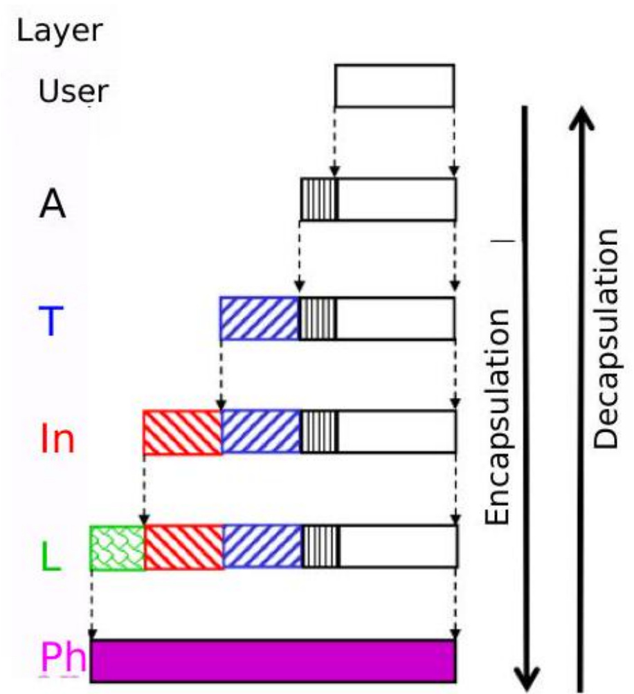
Fig. 8.6 Securing the Physical layer
