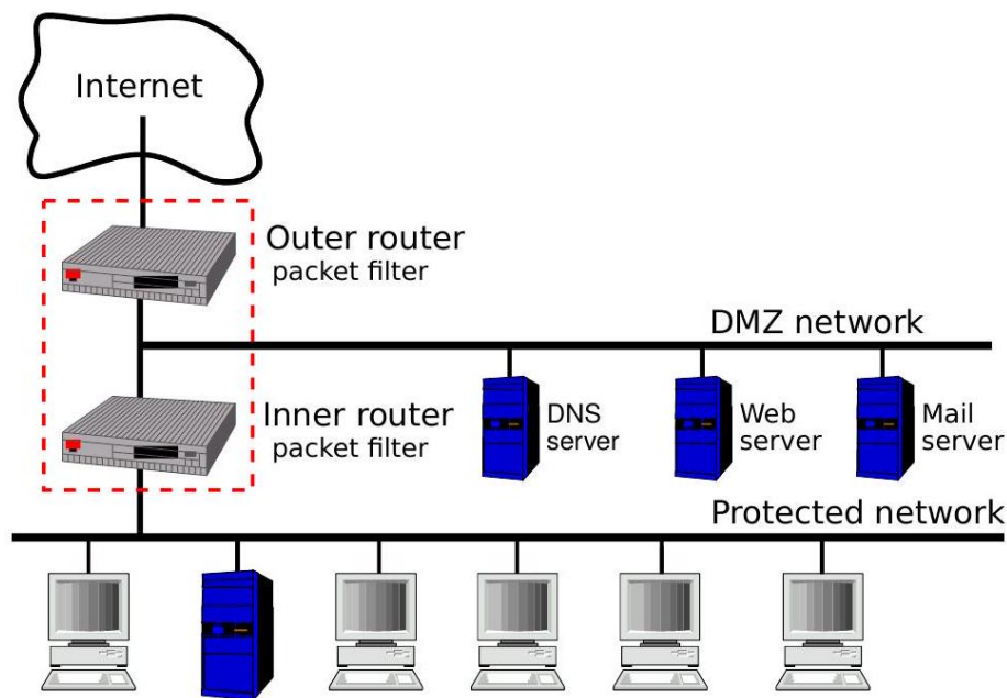
Fig. 8.23 A screened subnet setup with DMZ
