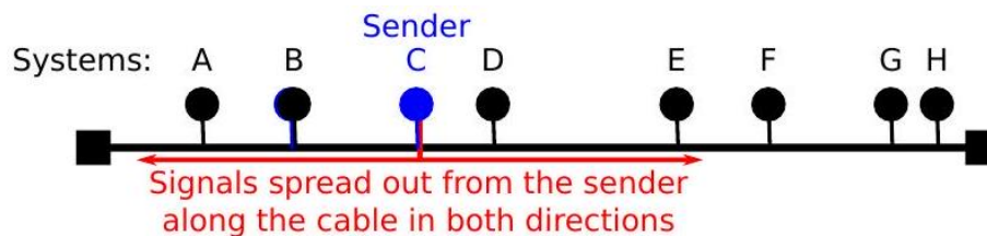
Fig. 6.15 Communication in Ethernet
