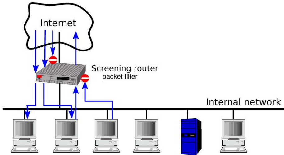
Fig. 8.20 A screening router setup
