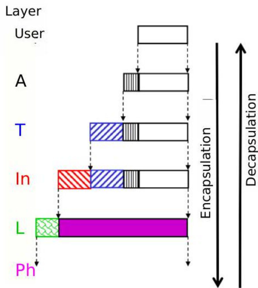
Fig. 8.5 Encryption in the Link layer
