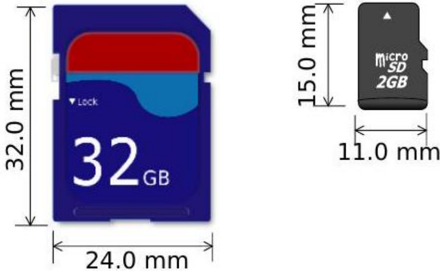
Fig. A. 5 Standard formats for Standard (left) and Micro (right) SD memory cards
