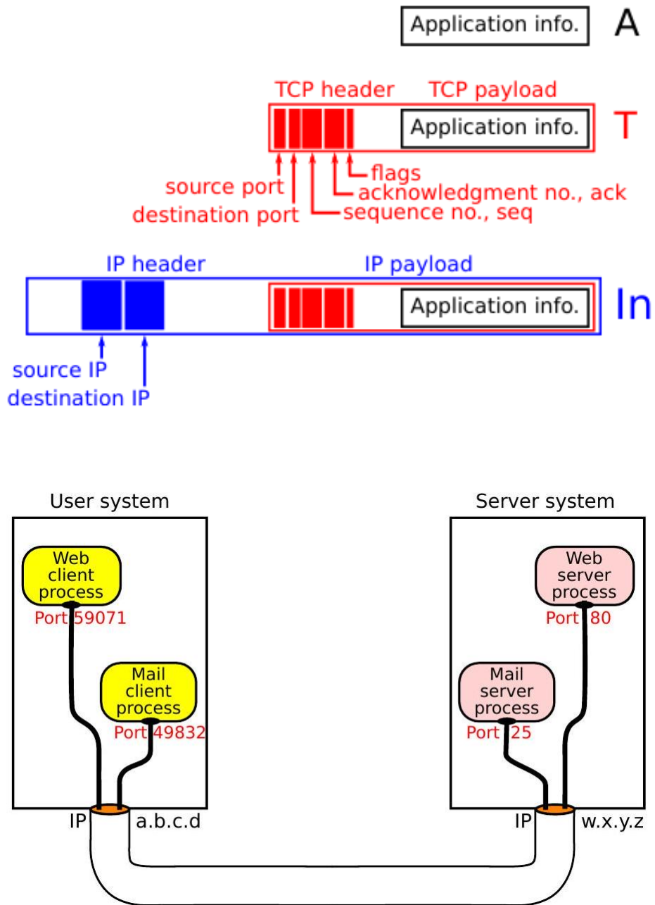
Fig. 6.9 Ports for use by TCP and UDP
