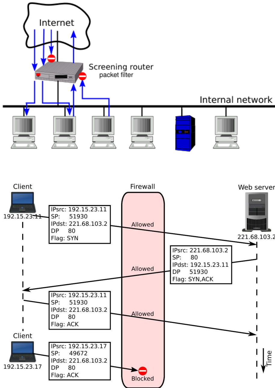
Fig. 8.18 An SPI firewall
