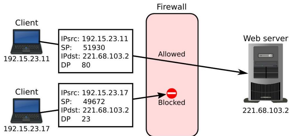
Fig. 8.17 A PF firewall
