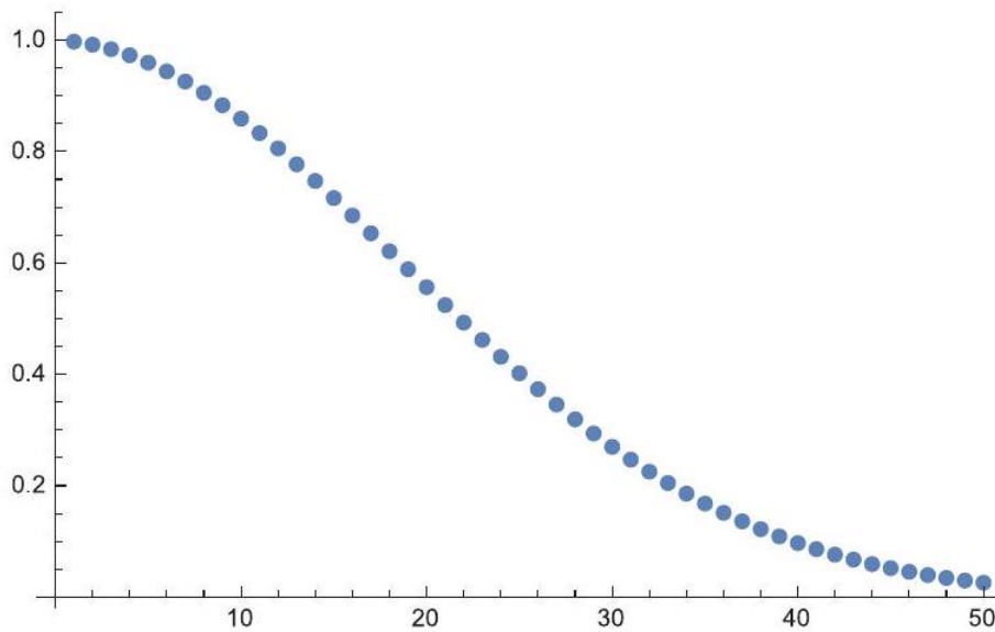
Figure 4.44: The probability of no collisions in a hash table decreases rapidly with n , the number of keys to hash. Here the hash table size is m = 365 .
