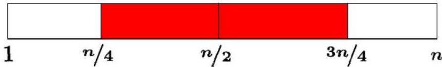
Figure 4.30: Half the time, a randomly chosen pivot is close to the median element.
