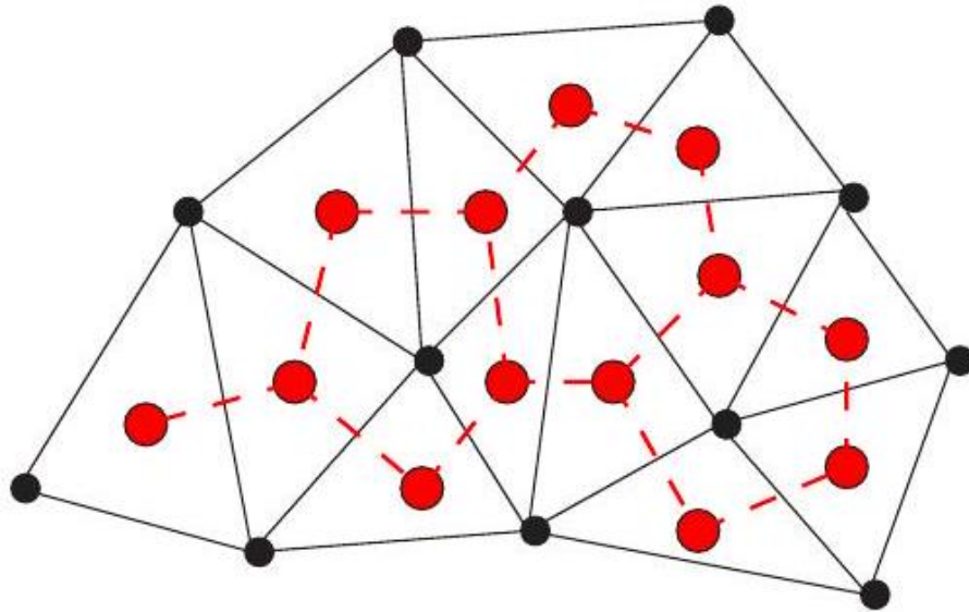
Figure 4.52: The dual graph (dashed lines) of a triangulation
