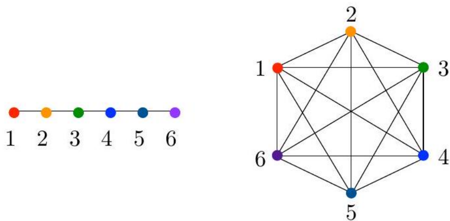
Figure 4.41: How long does a random walk take to visit all n nodes of a path (left) or a complete graph (right)?
