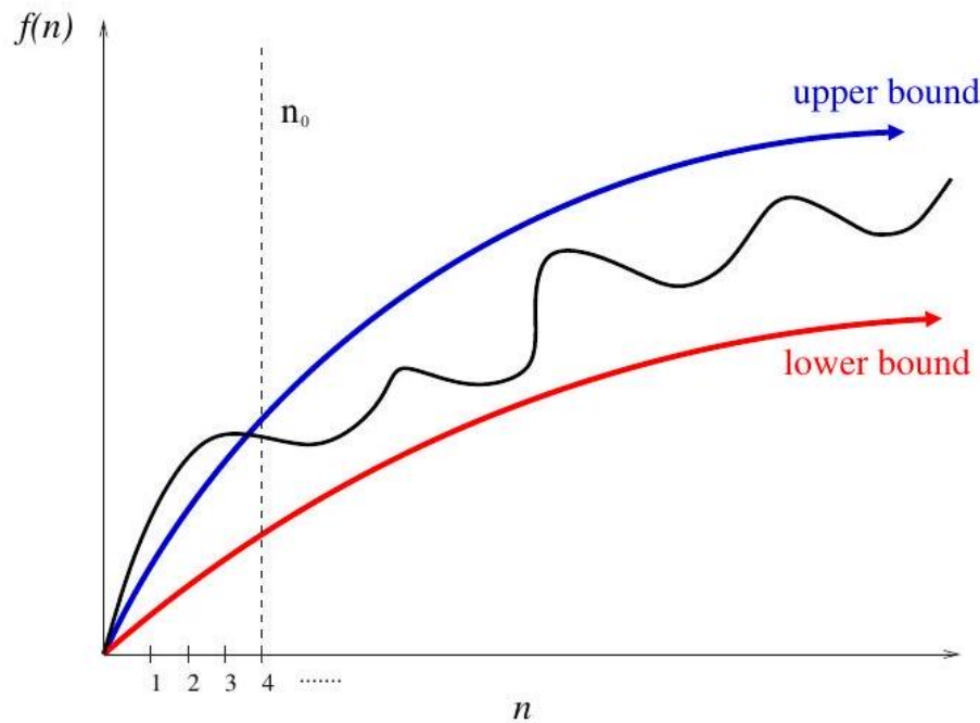
Figure 4.10: Upper and lower bounds valid for n > n_0 smooth out the behavior of complex functions.
