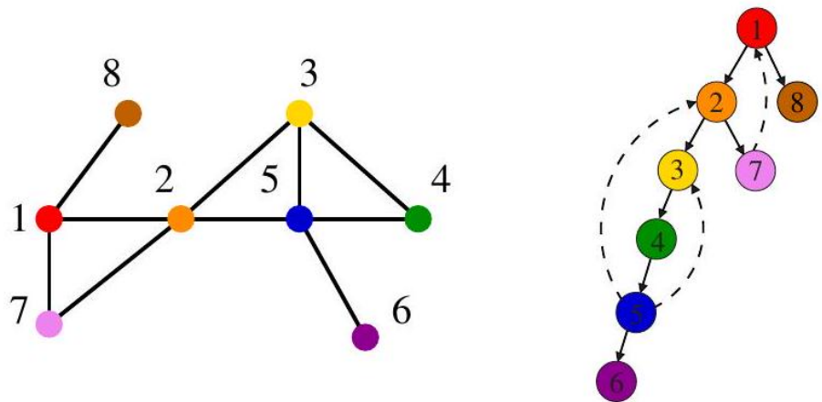
Figure 4.54: An undirected graph and its depth-first search tree. Dashed lines, which are not part of the tree, indicate back edges.
