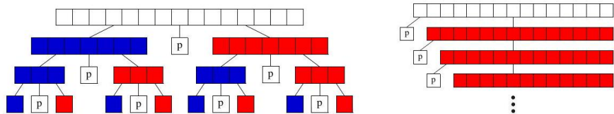
Figure 4.29: The best-case (left) and worst-case (right) recursion trees for quicksort. The left partition is in blue and the right partition in red.
