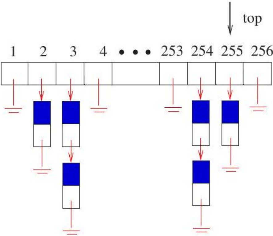
Figure 4.21: A bounded-height priority queue for triangle strips.
