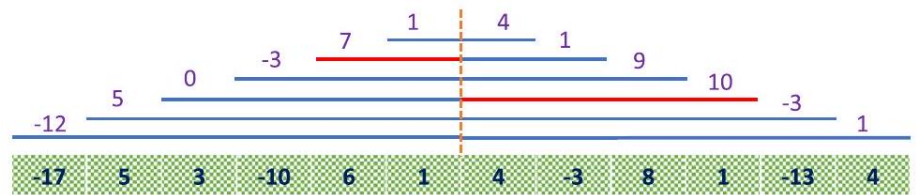
Figure 4.35: The largest subrange sum is either entirely to the left of center or entirely to the right, or (like here) the sum of the largest center-bordering ranges on left and right.
