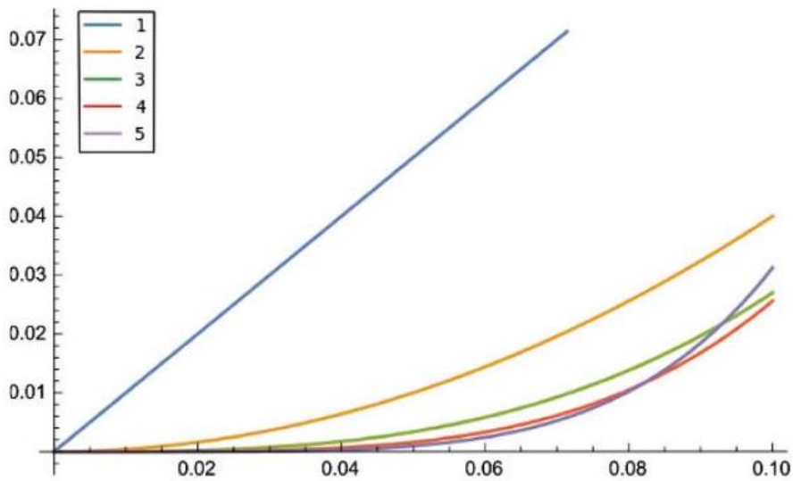
Figure 4.43: Bloom filter error probability as a function of load ( m/n ) for k from 1 to 5. By selecting the right k for the given load, we can dramatically reduce false positive error rate with no increase in table space.
