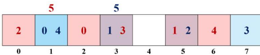
Figure 4.42: Hashing the integers 0, 1, 2, 3, and 4 into an n = 8 bit Bloom filter, using hash functions h_1(x) = 2x + 1 (blue) and h_2(x) = 3x + 2 (red). Searching for x = 5 would yield a false positive, since the two corresponding bits have been set by other elements.
