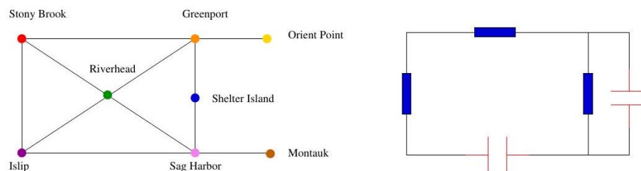
Figure 4.46: Modeling road networks and electrical circuits as graphs.
