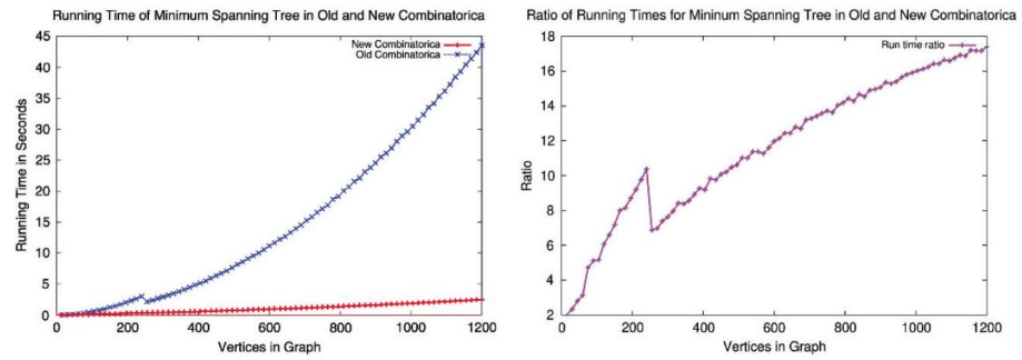
Figure 4.51: absolute running times (left), and the ratio of these times (right).
