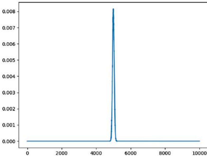
Figure 4.40: The probability distribution of getting h heads in n = 10,000 tosses of a fair coin is tightly centered around the mean, n/2 = 5,000 .
