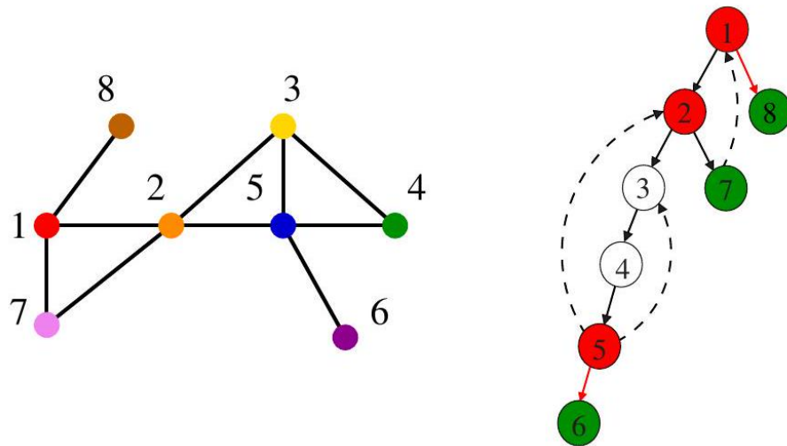
Figure 4.56: DFS tree of a graph containing three articulation vertices (namely 1, 2, and 5). Back edges keep vertices 3 and 4 from being cut-nodes, while green vertices 6, 7, and 8 escape by being leaves of the DFS tree. Red edges (1, 8) and (5, 6) are bridges whose deletion disconnect the graph.
