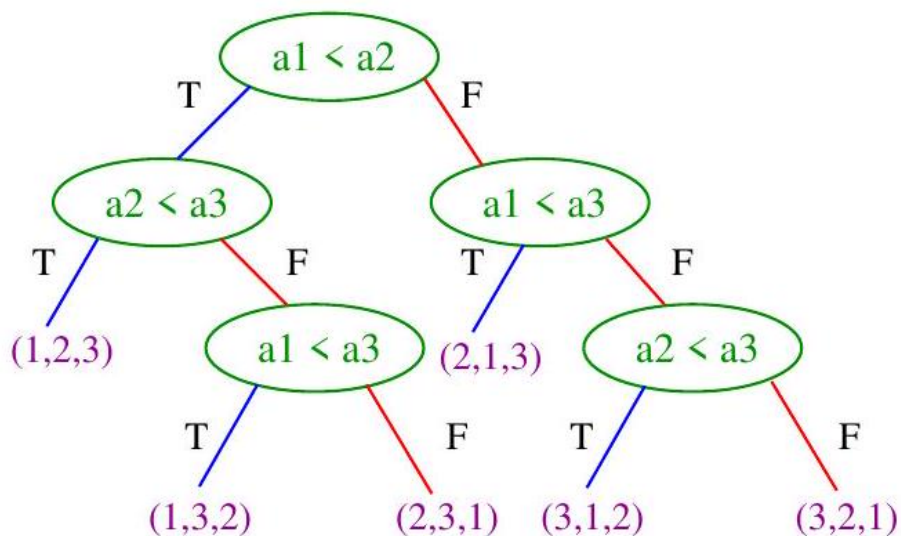
Figure 4.32: Interpreting insertion sort of input array a as a decision tree. Each leaf represents a given input permutation, while the root-to-leaf path describes the sequence of comparisons the algorithm does to sort it.
