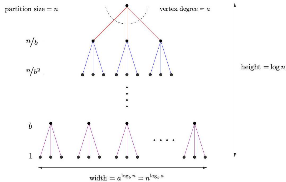
Figure 4.34: The recursion tree resulting from decomposing each problem of size n into a problems of size n/b
