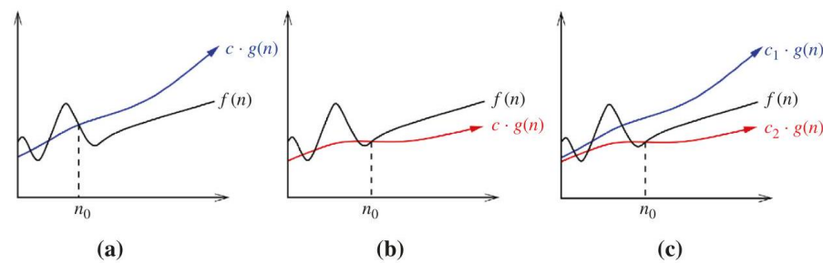
Figure 4.11: Upper and lower bounds valid for n > n_0 smooth out the behavior of complex functions.
