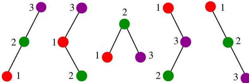
Figure 4.16: The five distinct binary search trees on three nodes. All nodes in the left (resp. right) subtree of node x have keys < x (resp. > x ).
