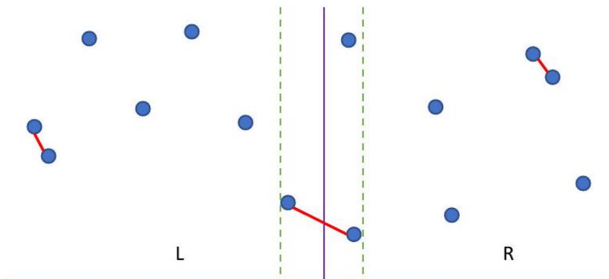
Figure 4.36: The closest pair of points in two dimensions either lie to the left of center, to the right, or in a thin strip straddling the center.
