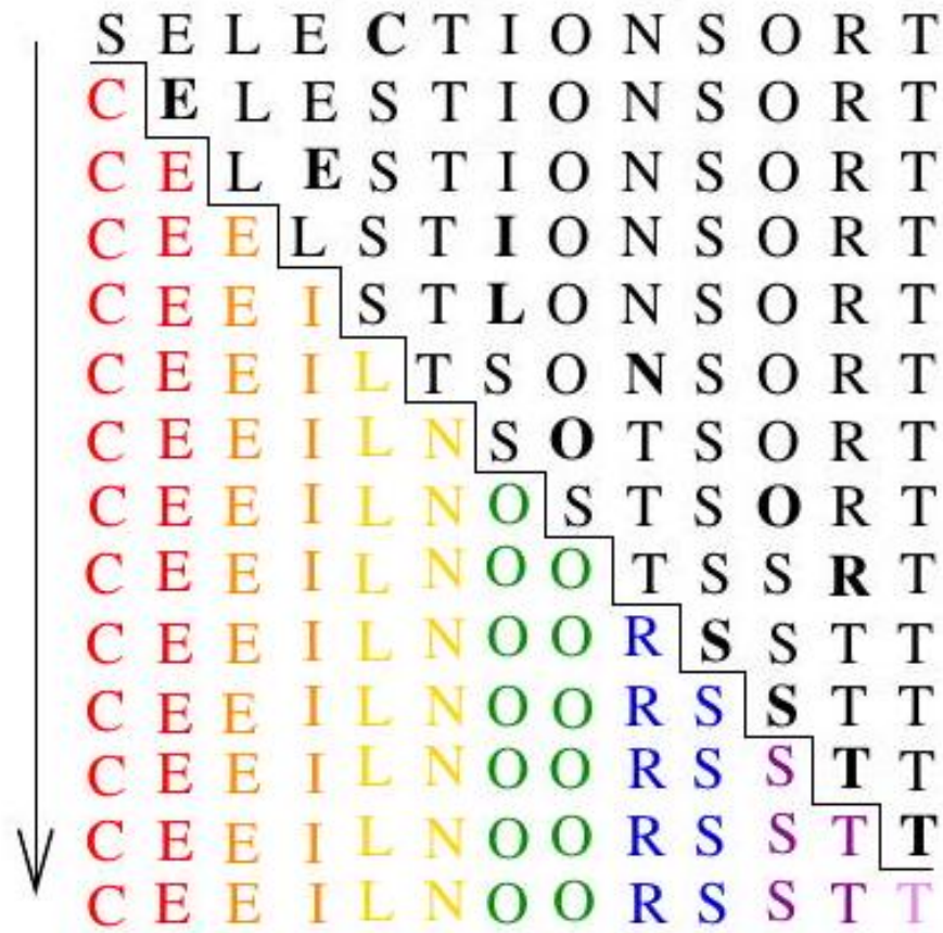
Figure 4.12: Animation of selection sort in action.
