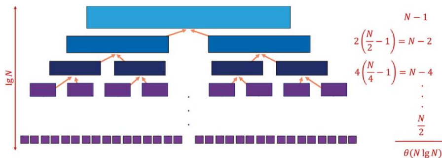
Figure 4.27: The recursion tree for mergesort. The tree has height \lceil \log_2 n \rceil , and the cost of the merging operations on each level are \Theta(n) , yielding an \Theta(n \log n) time algorithm.
