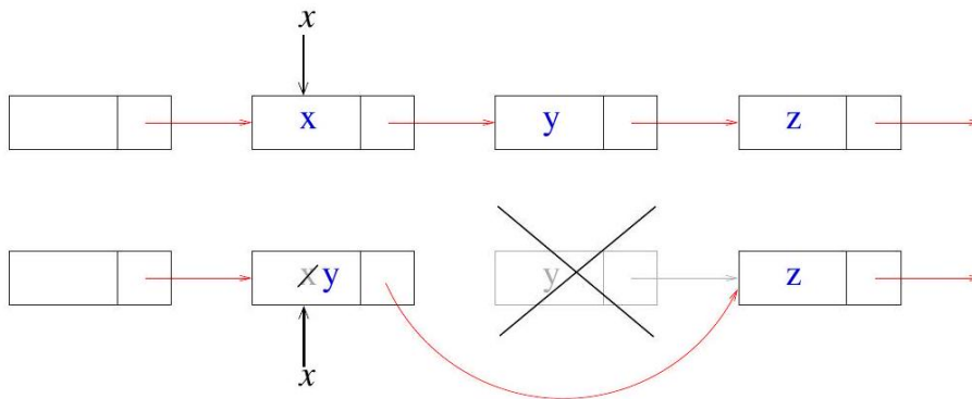
Figure 4.15: By overwriting the contents of a node-to-delete, and deleting its original successor, we can delete a node without access to its list predecessor.
