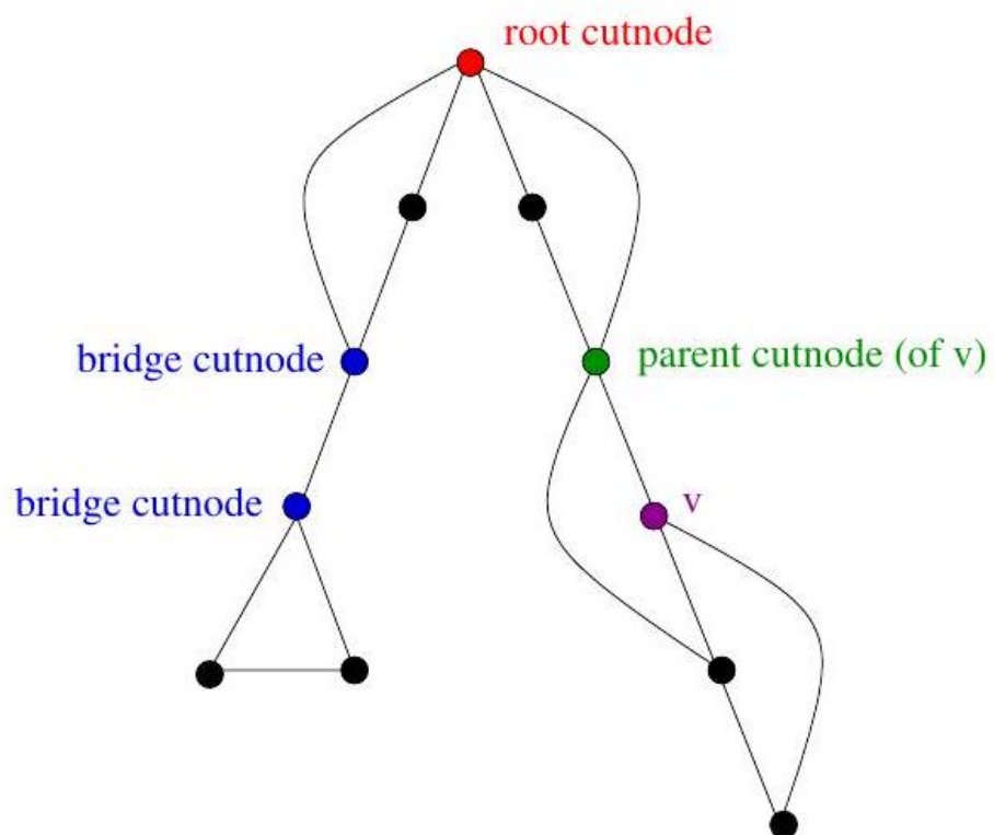
Figure 4.57: root, bridge, and parent cut-nodes.
