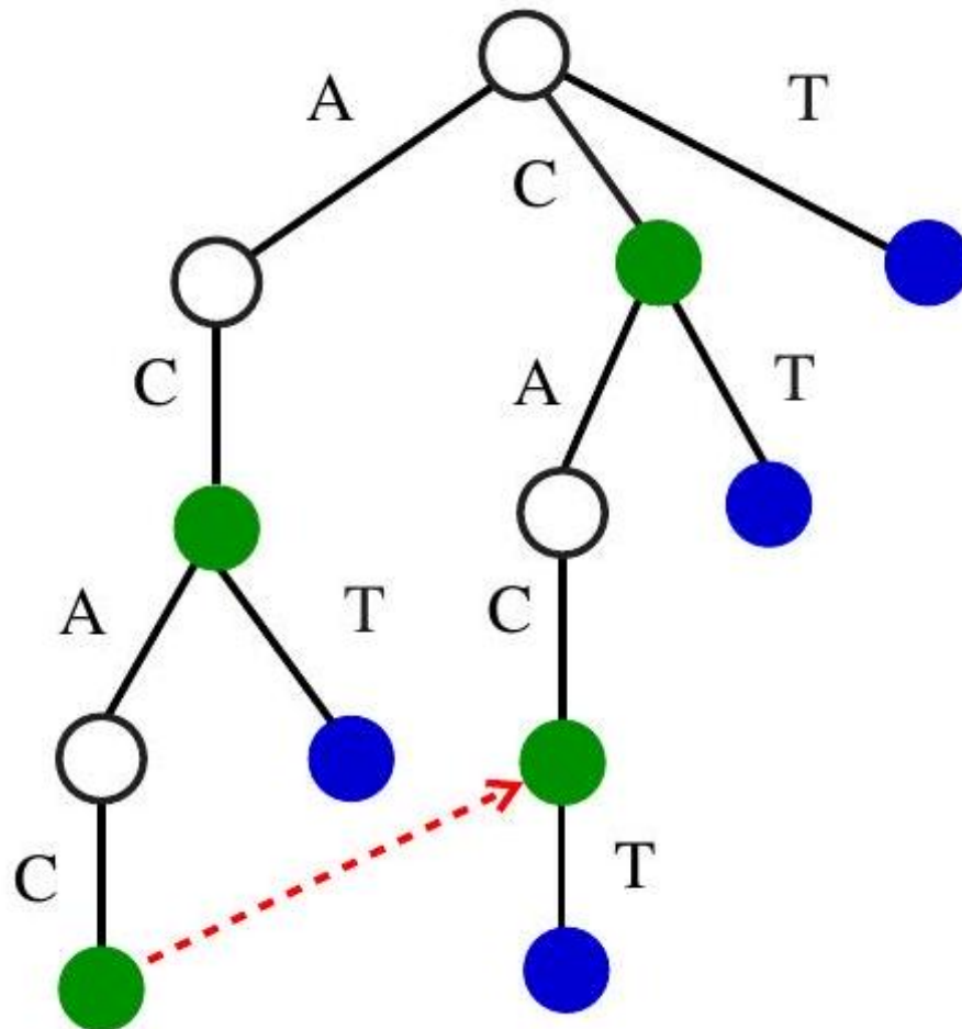
Figure 4.24: Suffix tree on ACAC and CACT , with the pointer to the suffix of ACAC . Green nodes correspond to suffixes of ACAC , with blue nodes to suffixes of CACT .
