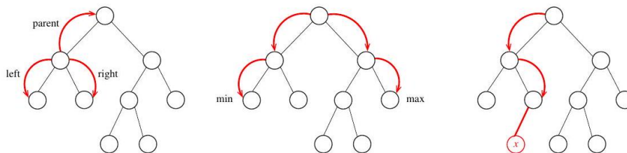
Figure 4.17: Relationships in a binary search tree. Parent and sibling pointers (left). Finding the minimum and maximum elements in a binary search tree (center). Inserting a new node in the correct position (right).
