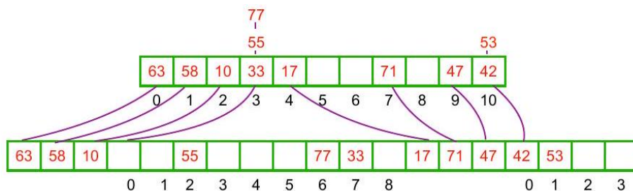
Figure 4.45: Perfect hashing uses a two-level hash table to guarantee lookup in constant time. The first-level table encodes an index range of l_i^2 elements in the second-level table, allocated to store the l_i items in first-level bucket i .
