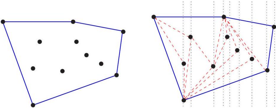
Figure 4.25: The convex hull of a set of points (left), constructed by left-to-right insertion (right).
