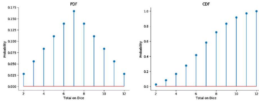
Figure 4.39: The probability density function (pdf) of the sum of two dice contains exactly the same information as the cumulative density function (cdf), but looks very different.
