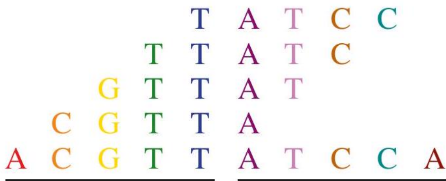
Figure 4.23: The concatenation of two fragments can be in S only if all subfragments are.
