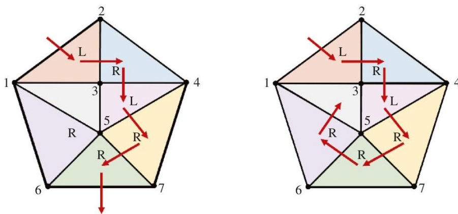
Figure 4.20: A strip with partial coverage using alternating left and right turns (left), and a strip with complete coverage by exploiting the flexibility of arbitrary turns (right).
