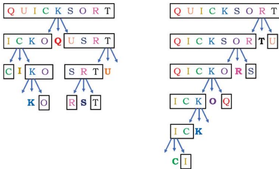
Figure 4.28: first selecting the first element in each subarray as pivot (on left), and then selecting the last element as pivot (on right).
