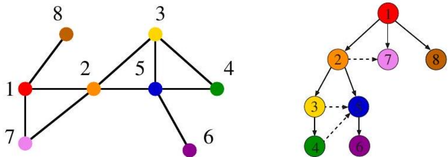
Figure 4.53: An undirected graph and its breadth-first search tree. Dashed lines, which are not part of the tree, show graph edges that go to discovered or processed vertices.
