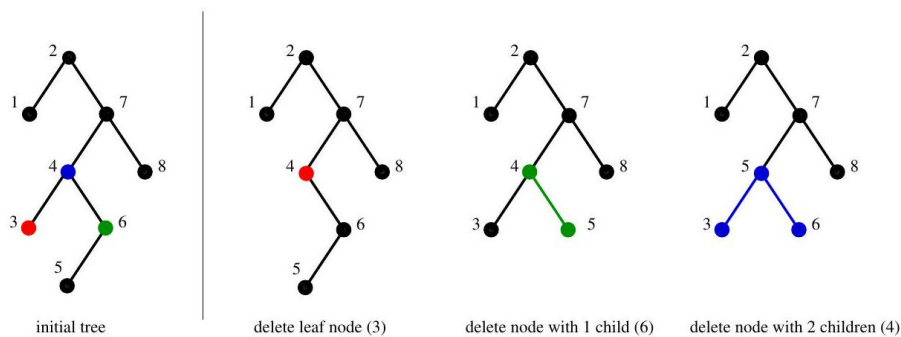
Figure 4.18: Deleting tree nodes with 0,1 , and 2 children. Colors show the nodes affected as a result of the deletion.
