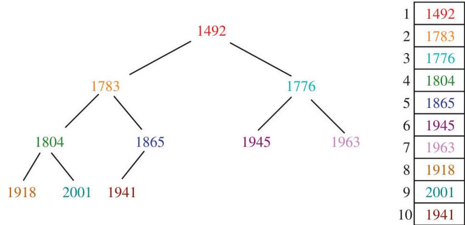
Figure 4.26: A heap-labeled tree of important years from American history (left), with the corresponding implicit heap representation (right).
