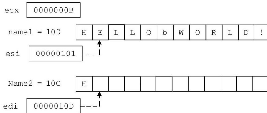
Figure 2.18: Using esi and edi to move a string
