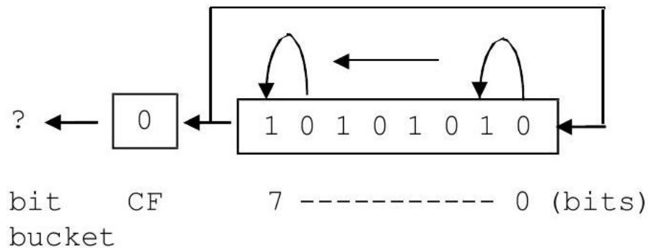
Figure 2.6: Initial contents of al Register
