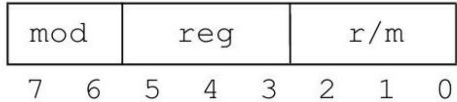
Figure 2.28: Format of mod reg r/m
