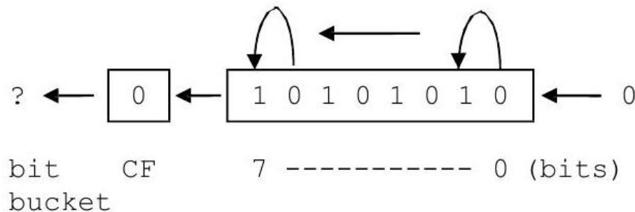
Figure 2.4: Results in al register after sal instruction
