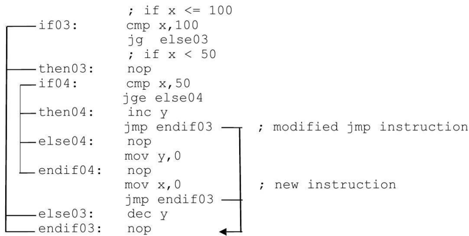
Figure 1.11: If-then-if structure with inadvisable jump
