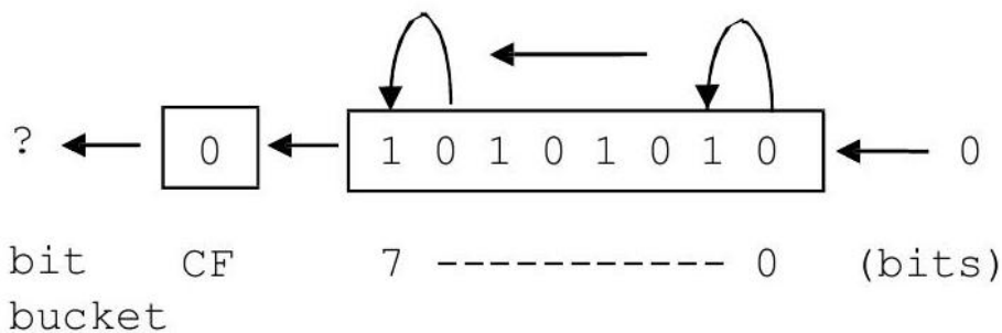
Figure 2.2: Results in al register after shl instruction
