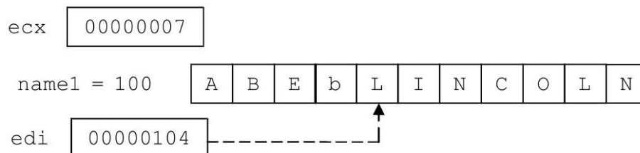
Figure 2.19: Using repne scasb
