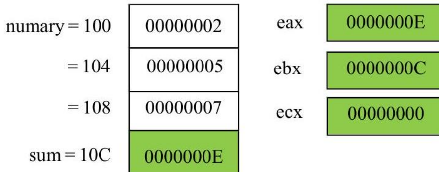
Figure 2.11: Using ebx for array processing
