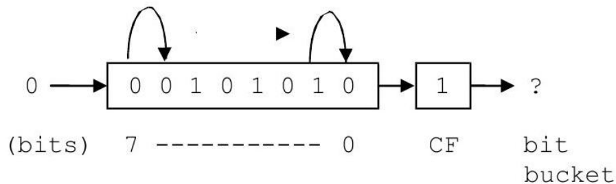
Figure 2.3: Results in al register after shl instruction
