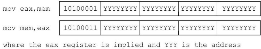
Figure 2.27: Format for the mov eax, mem and mov mem, eax instructions
