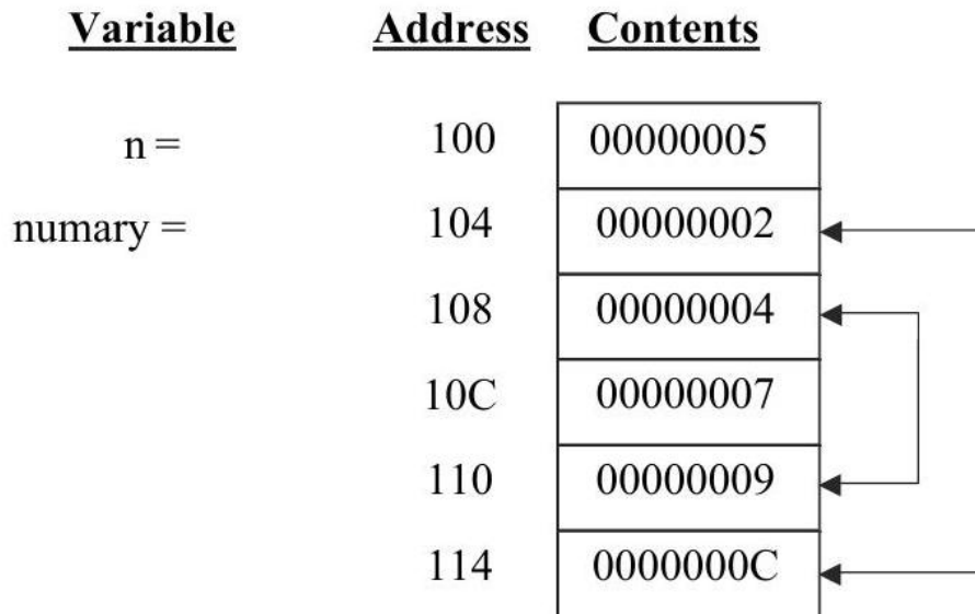
Figure 2.15: Swap routine
