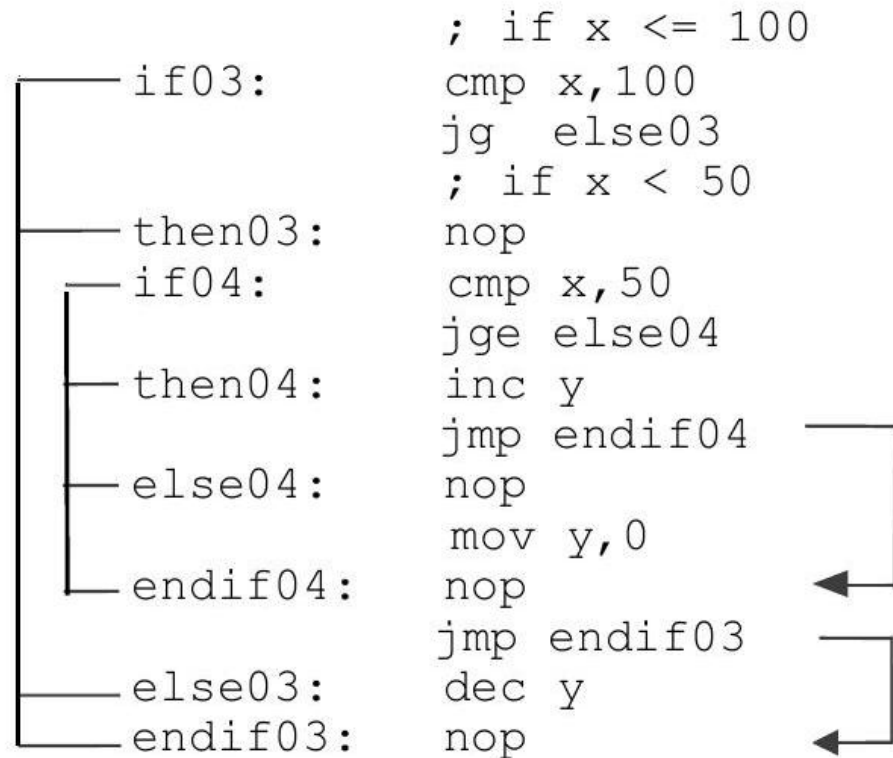
Figure 1.10: If-then-if structure
