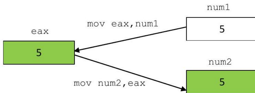
Figure 1.4: Mov instruction
