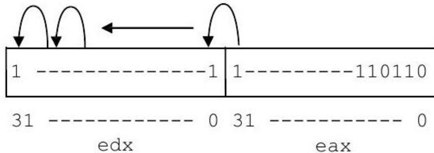
Figure 1.6: eax registers after execution of the imul instruction
