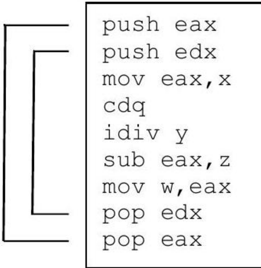
Figure 2.8: Saving and restoring multiple registers
