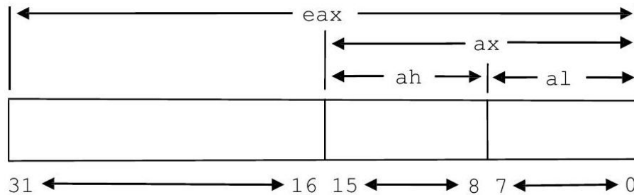
Figure 1.3: Format of the eax , ax , ah , and al registers
