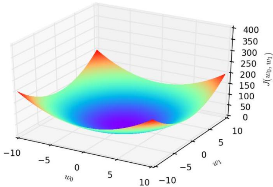
Figure 11.7: Linear regression defines a convex parameter space, where each point represents a possible line, and the minimum point defines the best fitting line.
