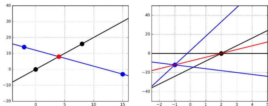
Figure 11.2: Points are equivalent to lines under a duality transform. The point (4, 8) in red (left) maps to the red line y = 4x - 8 on right. Both sets of three collinear points on the left correspond to three lines passing through the same point on right.
