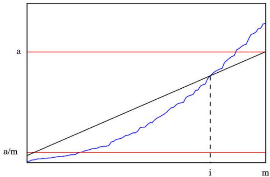
Figure 7.14: The Benjamini-Hochberg procedure minimizes false discovery rate, by accepting p -values only when p_i \leq \alpha i/m . The blue curve shows the sorted p values, and the diagonal defines the cutoff for when such a p -value is significant.
