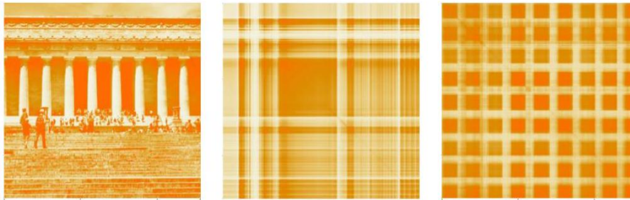
Figure 10.5: The Lincoln memorial M (left) and its covariance matrices. The big block in the middle of M \cdot M^T (center) results from the similarity of all rows from the middle stripe of M . The tight grid pattern of M^T \cdot M (right) reflects the regular pattern of the columns on the memorial building.
