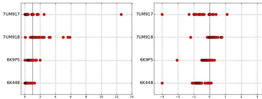
Figure 4.12: Plotting ratios on a scale cramps the space allocated to small ratios relative to large ratios (left). Plotting the logarithms of ratios better represents the underlying data (right).
