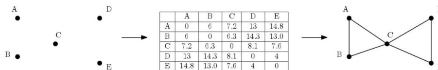
Figure 12.8: The pairwise distances between a set of points in space (left) define a complete weighted graph (center). Thresholding by a distance cutoff removes all long edges, leaving a sparse graph that captures the structure of the points (right).
