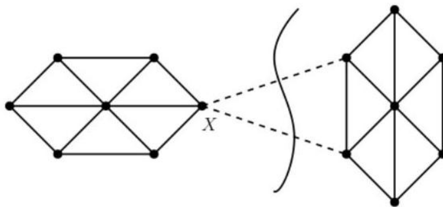
Figure 12.21: Low weight cuts in similarity graphs identify natural clusters.
