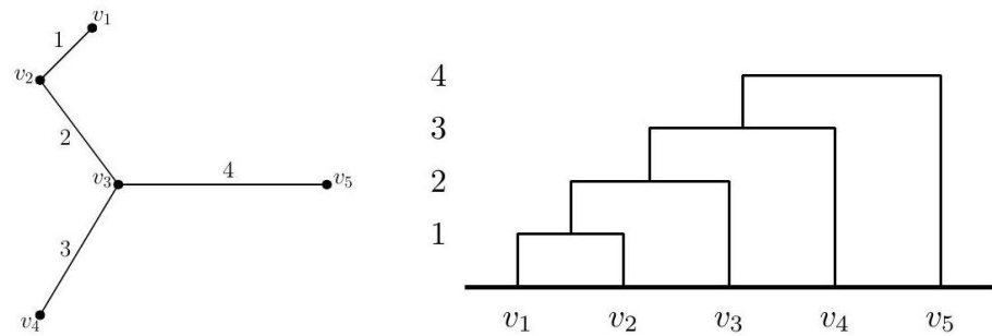
Figure 12.19: Single linkage clustering is equivalent to finding the minimum spanning tree of a network.
