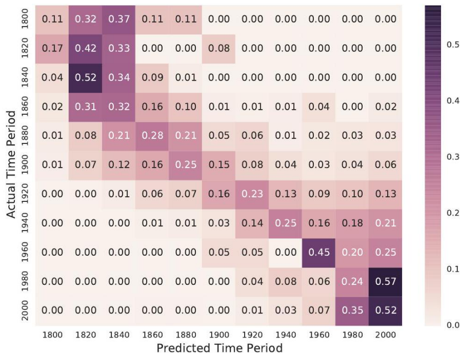
Figure 9.4: the main diagonal reflects accurate classification.
