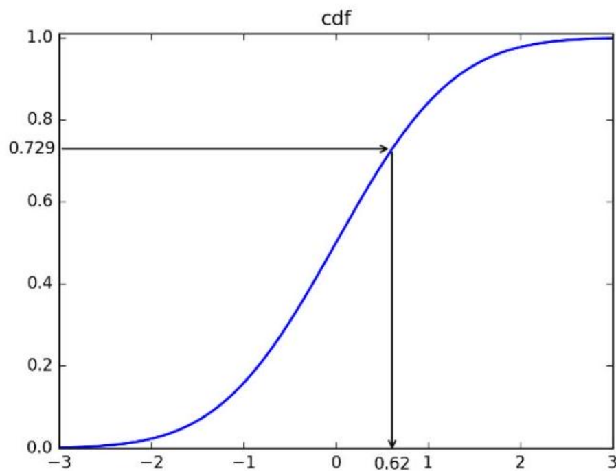
Figure 7.8: The inverse transform sampling method enables us to convert a random number generated uniformly from [0, 1] (here 0.729) to a random sample drawn from any distribution, given its cdf.
