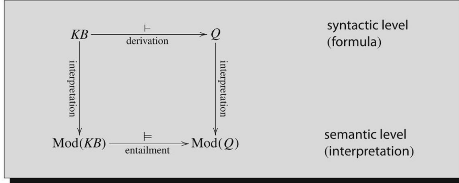
Fig. 2.1 Syntactic derivation and semantic entailment. \text{Mod}(X) represents the set of models of a formula X . The formula to be proved follows from the knowledge base. If a calculus is sound and complete, then syntactic derivation and semantic entailment are two equivalent relations (see Fig. 2.1).
