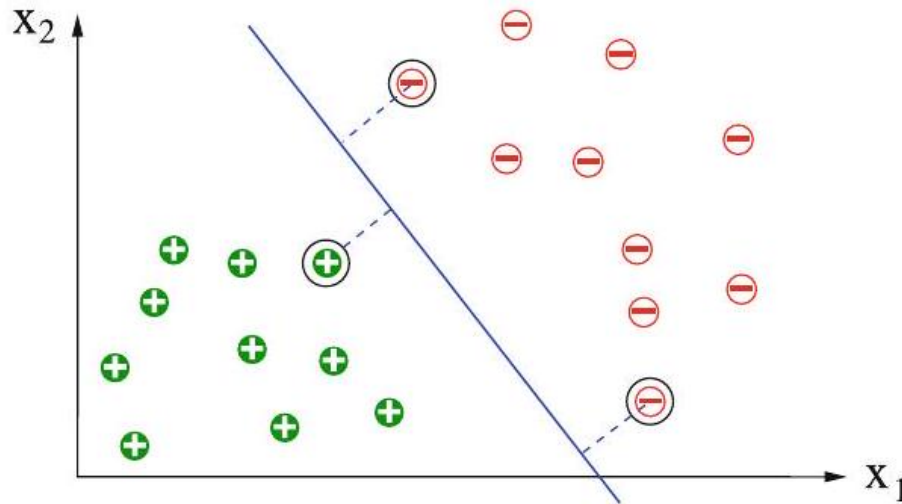
Fig. 9.25 Two classes with the maximally dividing line. The circled points are the support vectors
