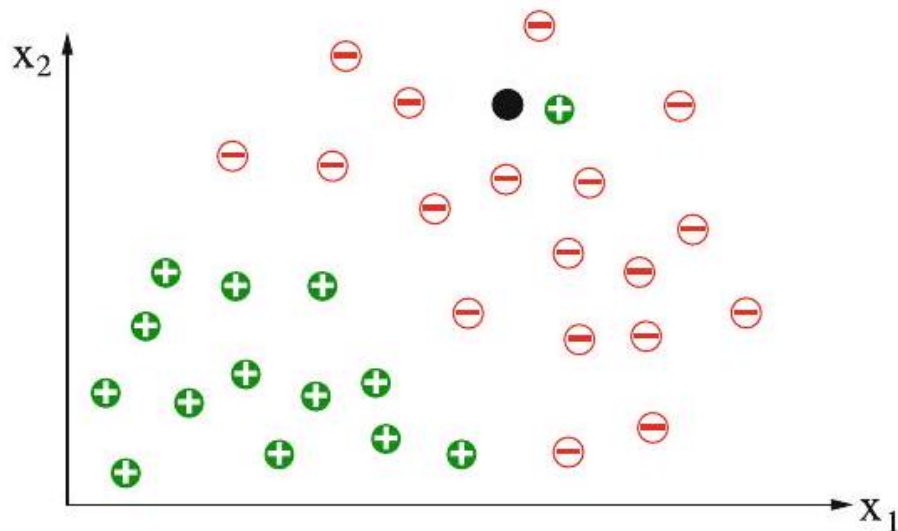
Fig. 8.15 The nearest neighbor method assigns the new point marked in black to the wrong (positive) class because the nearest neighbor is most likely classified wrong
