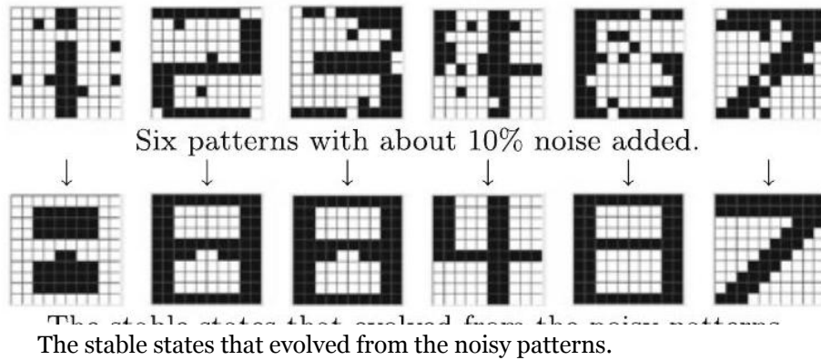
Fig. 9.7 For ten learned states the network shows chaotic behavior. Even with little noise the network converges to the wrong patterns or to artifacts
