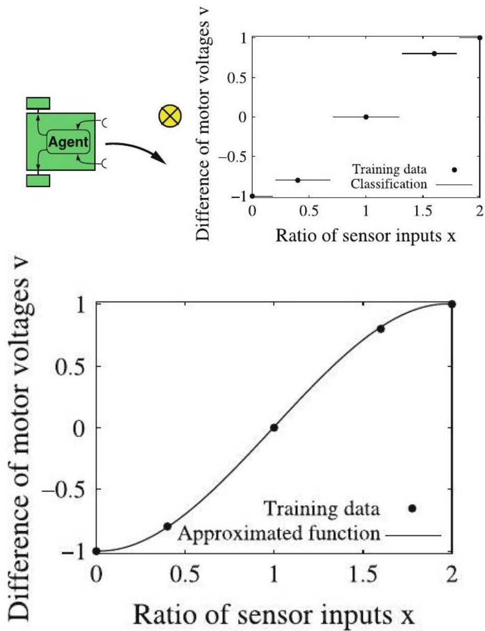
Fig. 8.18 The learning agent, which is supposed to avoid light (left), represented as a classifier (middle), and as an approximation (right)
