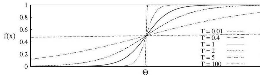
Fig. 9.4 The sigmoid function for various values of the parameter T . We can
