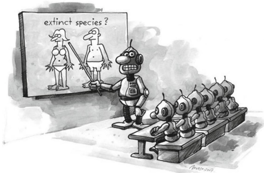
Fig. 8.1 Supervised learning ...
