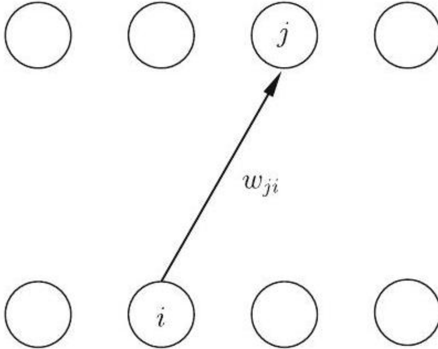
Fig. 9.19 Designation of the neurons and weights for the application of the backpropagation rule
