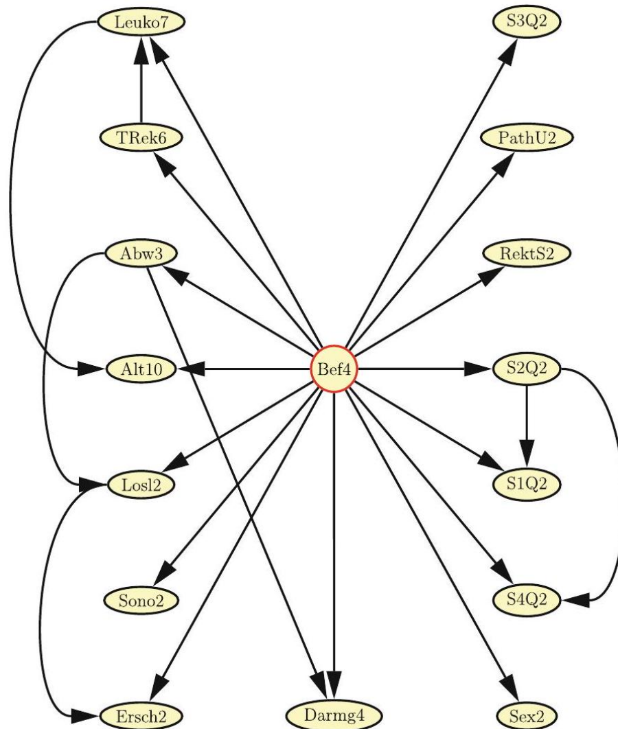
Fig. 7.14 Bayesian network for the Lexmed application
