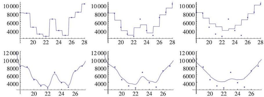
Fig. 8.19 Comparison of the k -nearest neighbor method (upper row) with k = 1 (left), k = 2 (middle) and k = 6 (right), to its distance weighted variant
