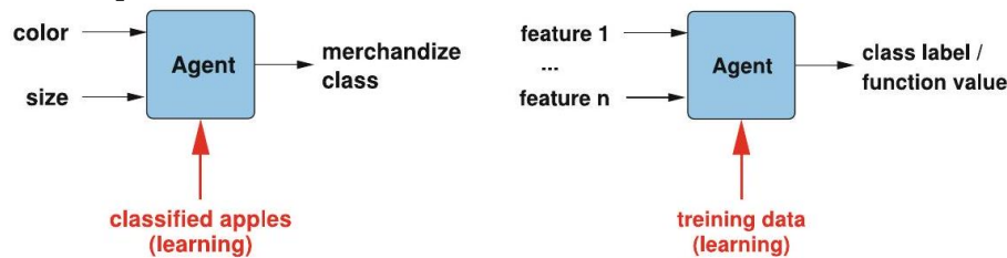
Fig. 8.4 Functional structure of a learning agent for apple sorting (left) and in general (right) which divides the classes as well as possible. A "good" division means that the percentage of falsely classified objects is as small as possible.
