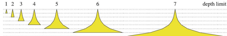
Fig. 6.10 Schematic representation of the development of the search tree in iterative deepening with limits from 1 to 7 . The breadth of the tree corresponds to a branching factor of 2
