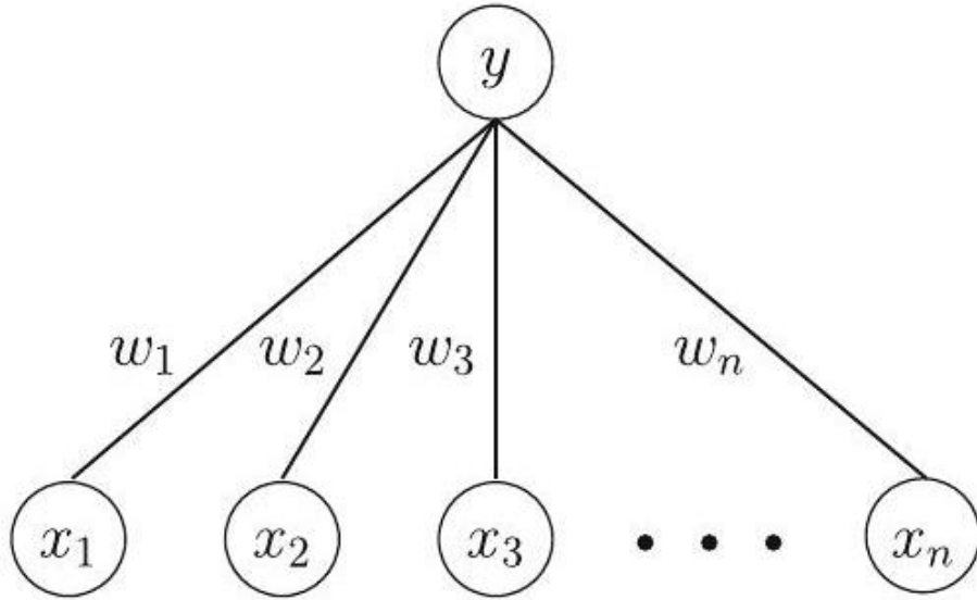
Fig. 9.13 A two-layer network with an output neuron
