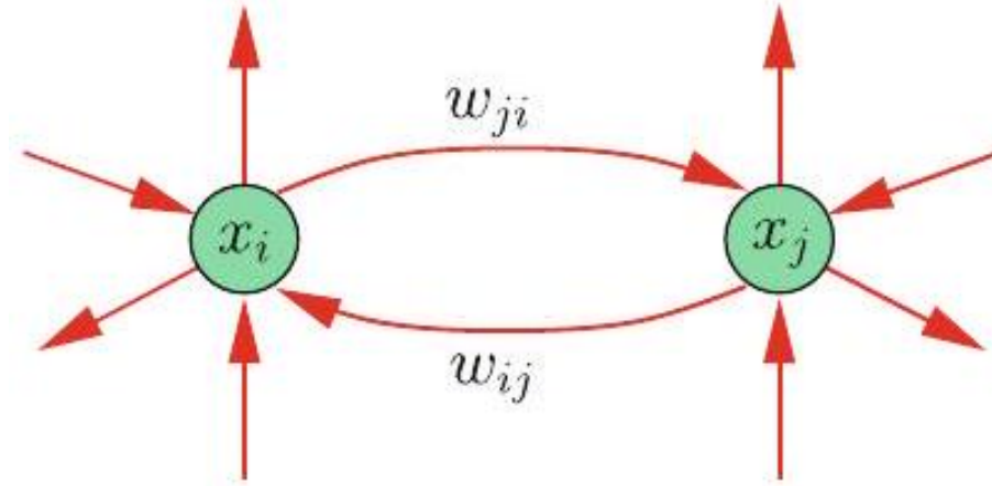
Fig. 9.5 Recurrent connections between two neurons in a Hopfield network w_{ij} . Each other pattern makes a negative contribution. Since each pixel corresponds to a neuron, here the weights between neurons which simultaneously have the same value are being reinforced. Please note this small difference to the Hebb rule.
