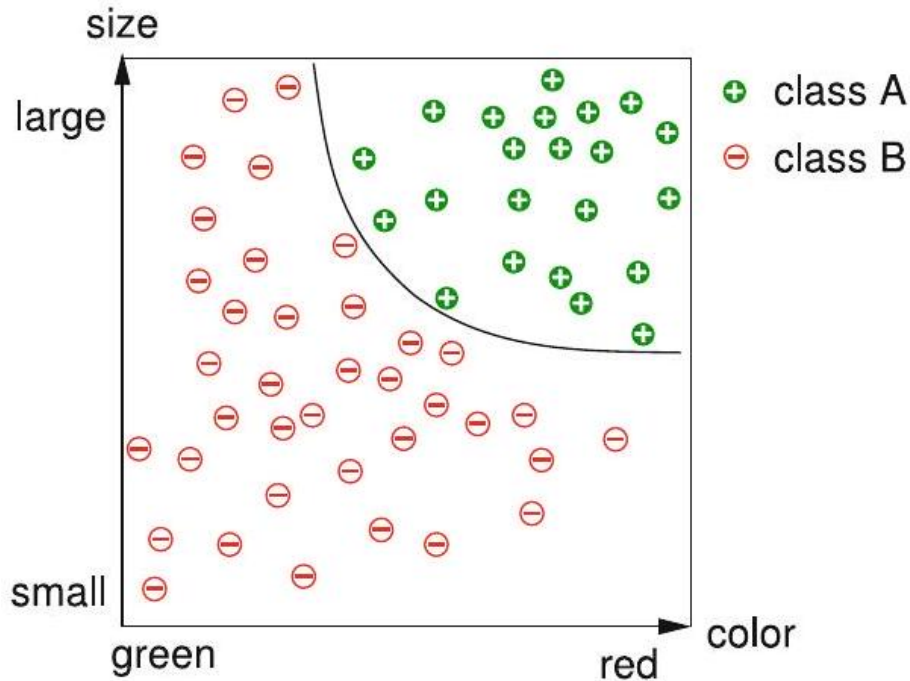
Fig. 8.3 The curve drawn in into the diagram divides the classes and can then be applied to arbitrary new apples
