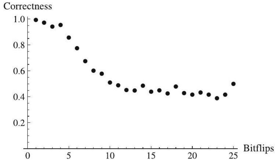
Fig. 8.12 Relative correctness of the perceptron as a function of the number of inverted bits in the test data
