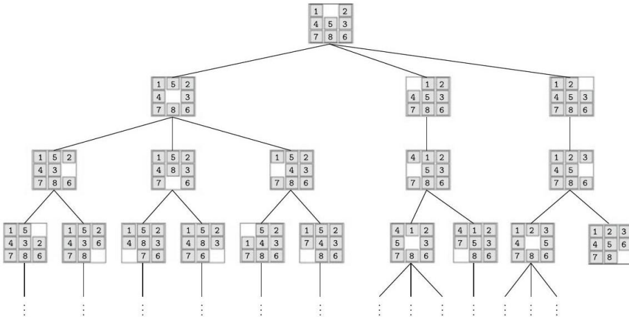
Fig. 6.4 Search tree for an 8-puzzle without cycles of length 2 that each state is repeated multiple times two levels deeper because in a simple uninformed search, every action can be reversed in the next step.
