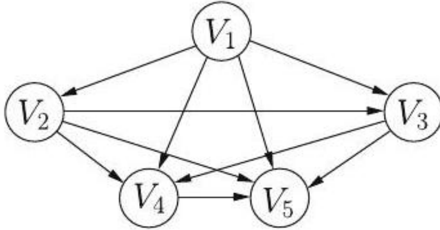
Fig. 8.30 The maximal network with five variables and edges (V_i, V_j) which fulfill the condition i < j
