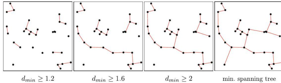
Fig. 8.36 The nearest neighbor algorithm applied to the data from Fig. 8.34 on page 227 at different levels with 12, 6, 3, 1 clusters in each step, that is, at each level, two subtrees are connected. At the top level all points are unified into one large cluster.
