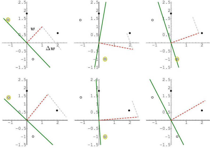
Fig. 8.10 Application of the perceptron learning rule to two positive ( \cdot ) and two negative ( \circ ) data points. The solid line shows the current dividing line wx = 0 . The orthogonal dashed line is the weight vector w and the second dashed line the change vector \Delta w = x or \Delta w = -x to be added, which is calculated from the currently active data point surrounded in light green
