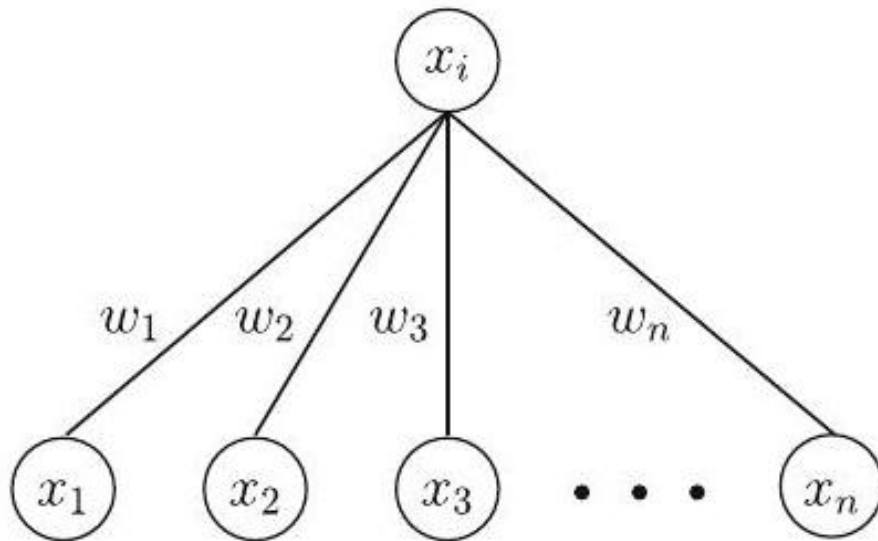
Fig. 9.3 The neuron with a step function works like a perceptron with a threshold
