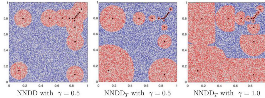
Fig. 8.32 \text{NNDD}_{\text{and}} \text{NNDD}_T applied to a set of 16 selected two-dimensional data points (black points). In each case, class membership has been determined for 10,000 randomly selected points. The points marked in red were classified as positive, i.e. assigned the training set's class, while the blue points are classified as negative
