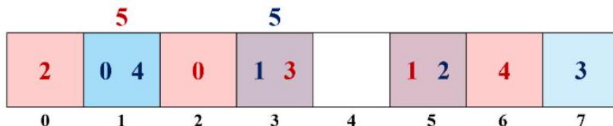
Figure 6.6: Hashing the integers 0, 1, 2, 3, and 4 into an n = 8 bit Bloom filter, using hash functions h_1(x) = 2x + 1 (blue) and h_2(x) = 3x + 2 (red). Searching for x = 5 would yield a false positive, since the two corresponding bits have been set by other elements.
