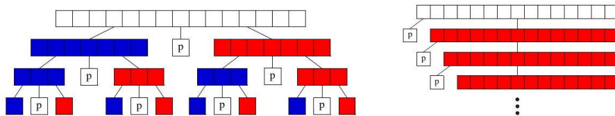
Figure 4.6: The best-case (left) and worst-case (right) recursion trees for quicksort. The left partition is in blue and the right partition in red. can halve n until we get down to 1, meaning h = \lceil \lg n \rceil . This happy situation is shown in Figure 4.6(left), and corresponds to the best case of quicksort.
