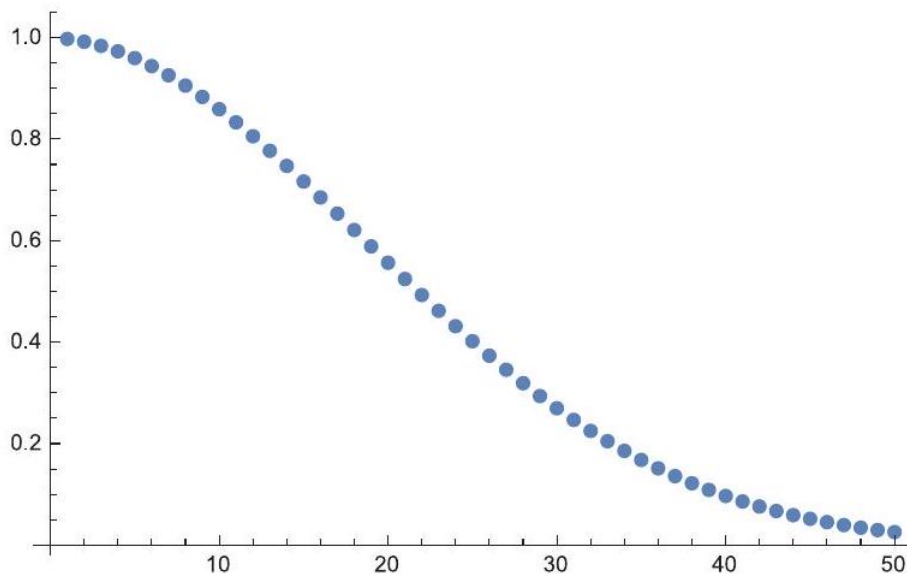
Figure 6.8: The probability of no collisions in a hash table decreases rapidly with n , the number of keys to hash. Here the hash table size is m = 365 . probability of no collisions drops below 1/2 for n = 23 and is less than 3% when n \geq 50 , as shown in Figure 6.8. In other words, odds are we have a collision when only 23 people are in the room. Solving this asymptotically, we begin to expect collisions when n = \Theta(\sqrt{m}) or equivalently when m = \Theta(n^2) .
