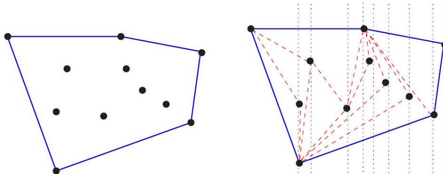
Figure 4.1: The convex hull of a set of points (left), constructed by left-to-right insertion (right).
