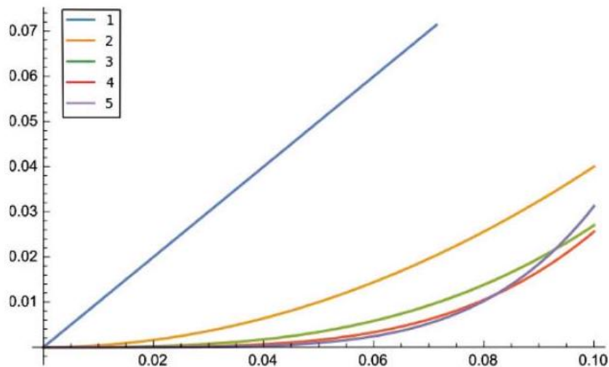
Figure 6.7: Bloom filter error probability as a function of load (m/n) for k from 1 to 5. By selecting the right k for the given load, we can dramatically
