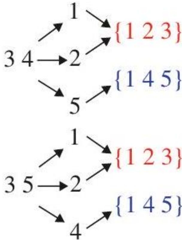
Figure 1.12: Guaranteeing a winning pair from \{1, 2, 3, 4, 5\} using only tickets \{1, 2, 3\} and \{1, 4, 5\} . The bottom figure shows how all missing pairs imply a covered pair on expansion.
