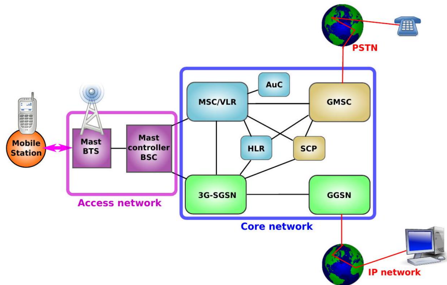
Fig. 6.19 The architecture of a telephone network based on GSM the transition to the Public Switched Telephone Network (PSTN). Ordinary data which is to be sent through the Internet is sent to a Serving GPRS Support Node (SGSN), which can handle GPRS, and which sends them on to a Gateway GPRS Support Node (GGSN), which handles the transition to the Internet.
