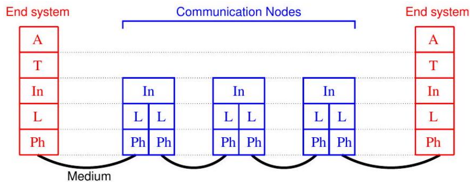
Fig. 6.12 End systems and communication nodes work as routers, with the typical functionality that they:
