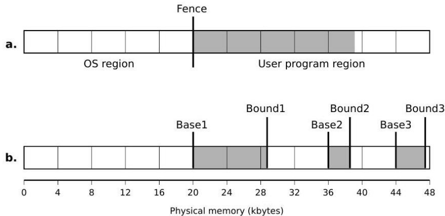
Fig. 9.17 Two simple techniques for memory protection a. Separation of user program from OS with a fence. b. Delimiting of areas with base-and-bounds limits
