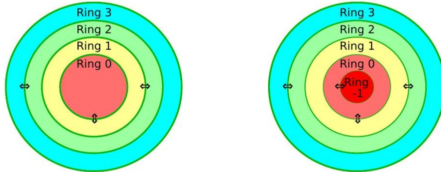
Fig. 9.20 Protection rings for a CPU Left: Standard Intel x86 and AMD Right: With Intel VT-x or AMD-V for hypervisor mode
