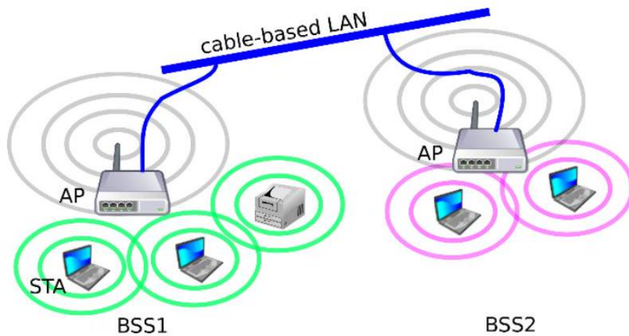
Fig. 6.17 WiFi Infrastructure Mode: An ESS with two BSSs
