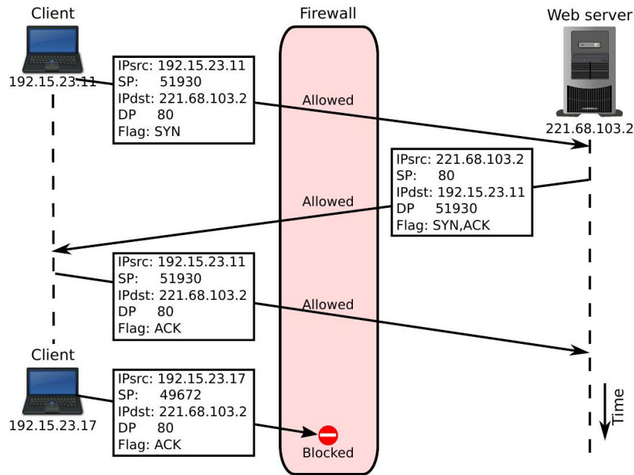
Fig. 8.18 An SPI firewall
