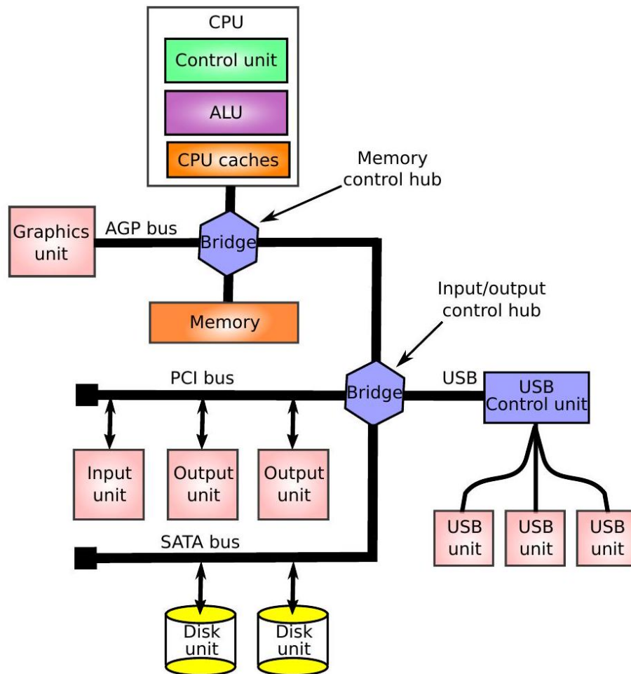
Fig. A. 6 Schematic architecture of a modern computer alternative type of bus for fast serial communication (up to 3.2Gbit/s ), and is used particularly for connection of audio-visual equipment such as video cameras and displays. The I/O control hub can also be used for direct attachment of communication equipment, and via an even slower subnet known as the LPC bus for attachment of a keyboard, mouse or other units which use serial communication, if they cannot be attached via the USB.
