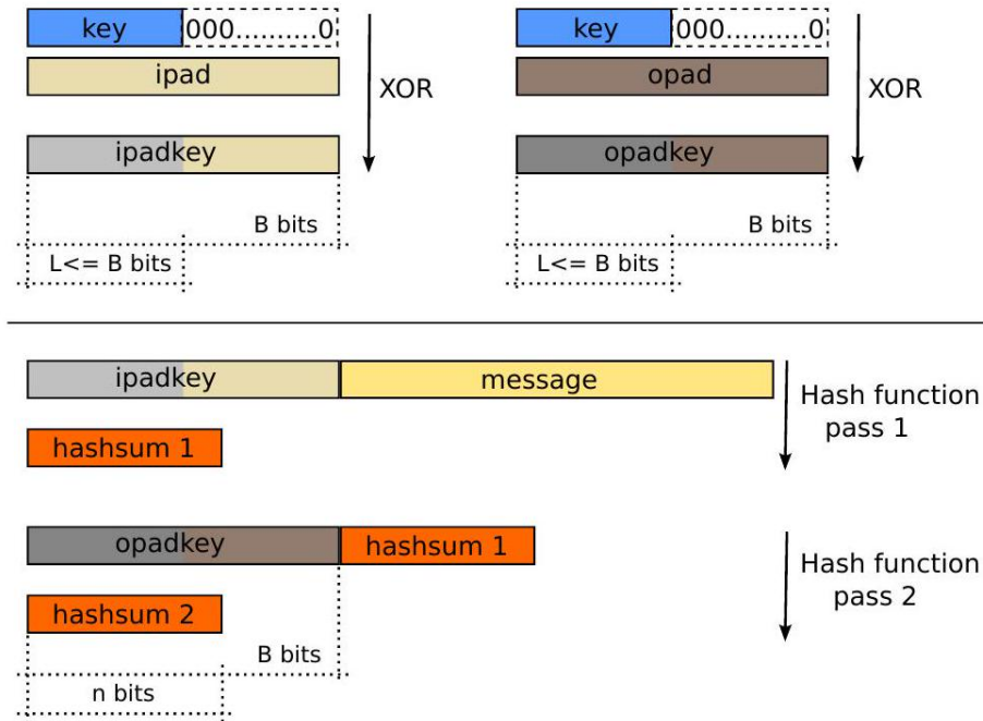
Fig. 5.5 Generating an HMAC (Source: Wikimedia Commons ©)
