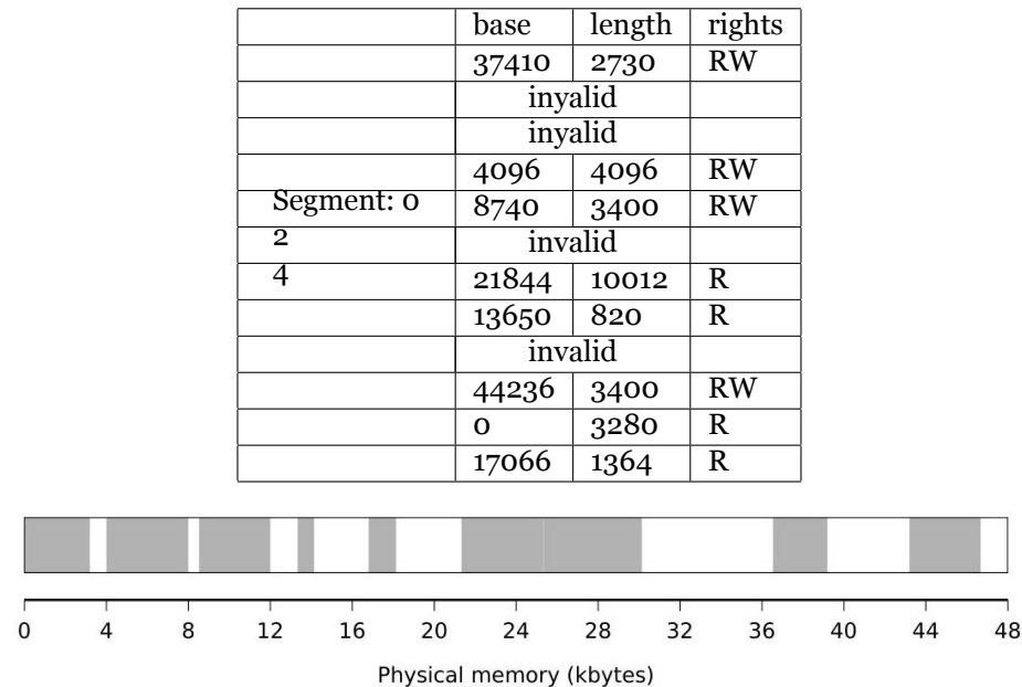
Fig. 9.18 A segment table and the allocation of space in the memory which it corresponds to memory from address 37410 and up and has length 2730 bytes, while Segment 6 is a segment which can only be read, placed in the memory from address 21844 and up, and with length 10012 bytes. The example shows a very small physical memory of only 48 kbytes. In a modern computer, the size would normally be very much larger—for example several Gbytes. The segment table itself would very often be stored in the memory in a special area when only the OS has access to.
