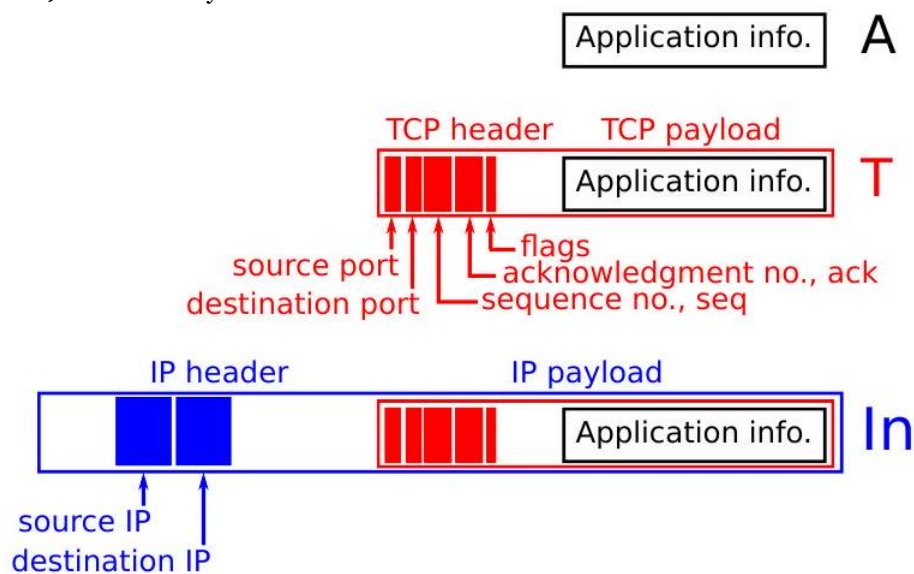
Fig. 6.10 Encapsulation in TCP and IP and the acknowledgment field ack contains the sequence number (modulo 2^{32} ) of the next data byte which the sender expects to receive from the other party. This implicitly acknowledges correct receipt of all data bytes up to and including number (ack-1).
