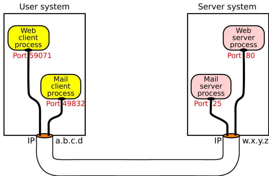
Fig. 6.9 Ports for use by TCP and UDP
