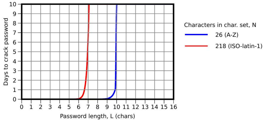
Fig. 9.7 Time to crack a password versus the password's length In the figure it is assumed, for the sake of example, that the attacker can test 1000 million passwords per second.
