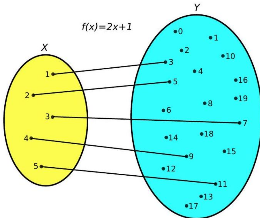
Fig. B. 1 Graph of the function f(x) = 2x + 1 with domain the set of integers \{1, 2, 3, 4, 5\} and co-domain the set of all non-negative integers less than 20 .
