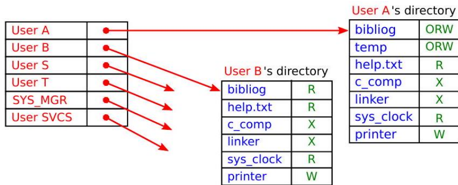
Fig. 9.13 Directories
