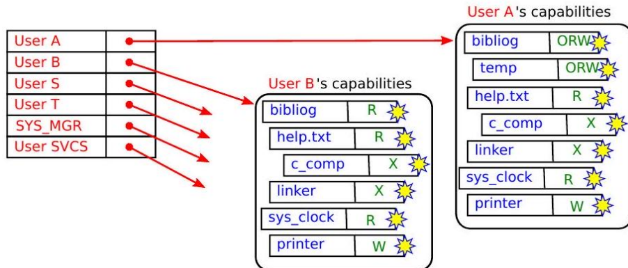
Fig. 9.14 Capabilities
