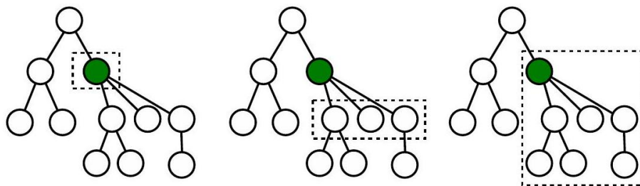
Fig. 10.10 Scope in LDAP searches. The filled circle is the chosen base object. From left to right: base, one and sub.
