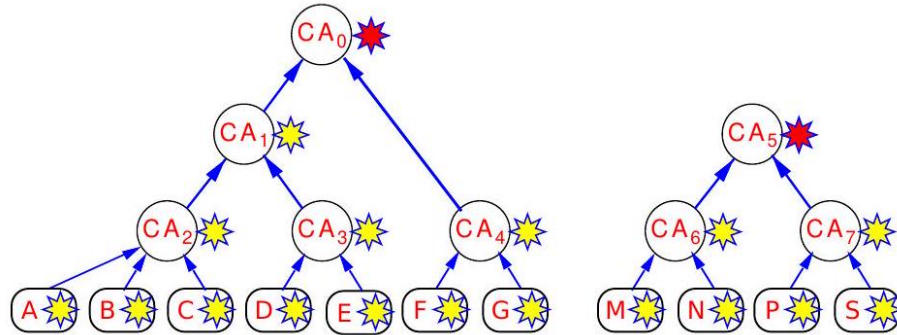
Fig. 5.17 Two trust hierarchies in a PKI certificate has been signed by CA_3 and CA_3 's certificate by CA_1 . And since subject A's certificate has been signed by CA_2 and F's certificate by CA_4 , then A and F can trust one another's certificates, since they have a common superior, CA_0 , in the hierarchy. CA_0 and CA_5 are the two root CAs, as described in Sect. 5.5. They have root certificates, shown as small red stars.
