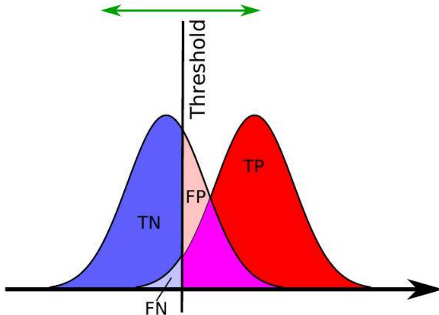
Fig. 8.24 Statistical variation makes it hard to make decisions FPR and FNR are affected by the threshold's position
