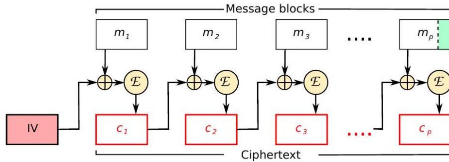
Fig. 4.10 Operation of DES in CBC mode
