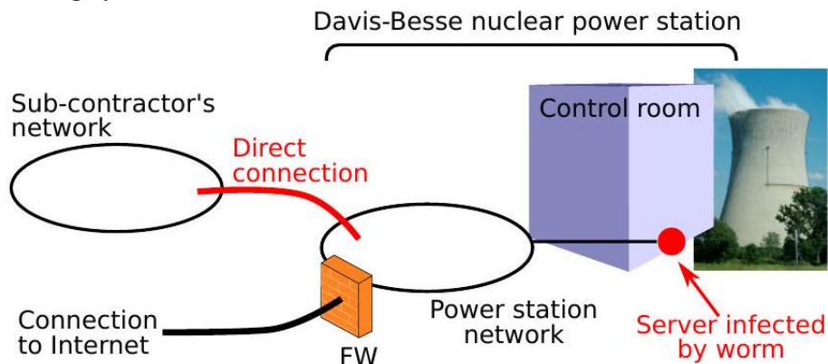
Fig. 8.34 The event in the Davis-Besse nuclear power station (Foto of Davis-Besse cooling tower: Wikimedia Commons (8))
