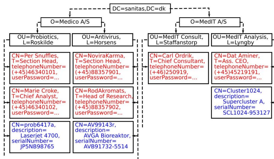
Fig. 10.9 An information hierarchy (DIT) for LDAP surname (SN) or a "common name" (CN), in addition to which there can optionally be a password, a phone number, a description and/or a collection of DNs for other objects (seeAlso) which describe the same person. These could for example describe the person's role (organizationalRole), a collection of information about the person's residence (residentialPerson) etc. Correspondingly, it is mandatory for an organisational object (organization) to provide an organization (O) attribute, for a organisational unit object (organizationalUnit) to provide an organizationalUnit
