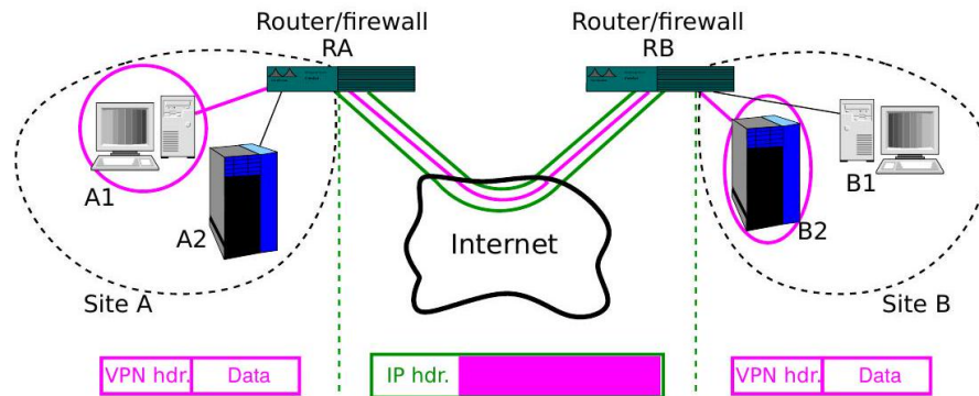
Fig. 8.11 Secure site-to-site tunneling in a VPN
