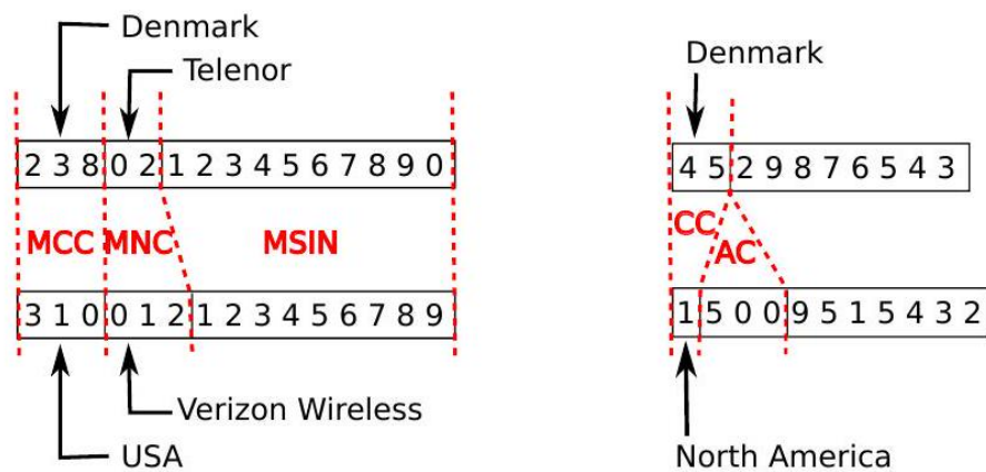
Fig. 6.20 The structure of an IMSI (left) and an MSISDN (right) in a database in the network's Authentication Centre ( AuC ), which checks the information in the SIM card before the subscriber is allowed to register on the network. We return to this topic in Chap. 8, where we discuss security in the mobile network in more detail.
