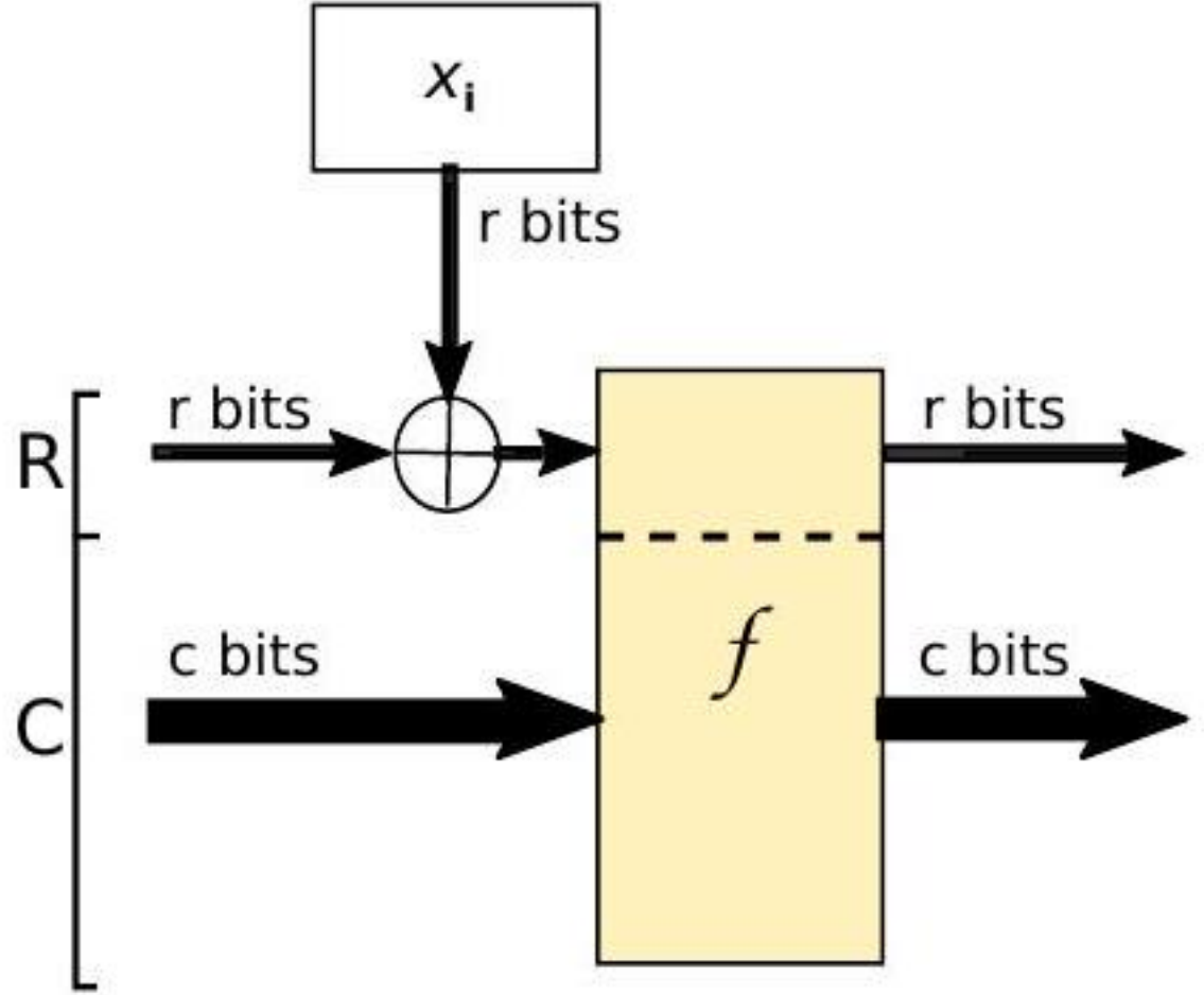
Figure 5.3: A step in the operation of a sponge
