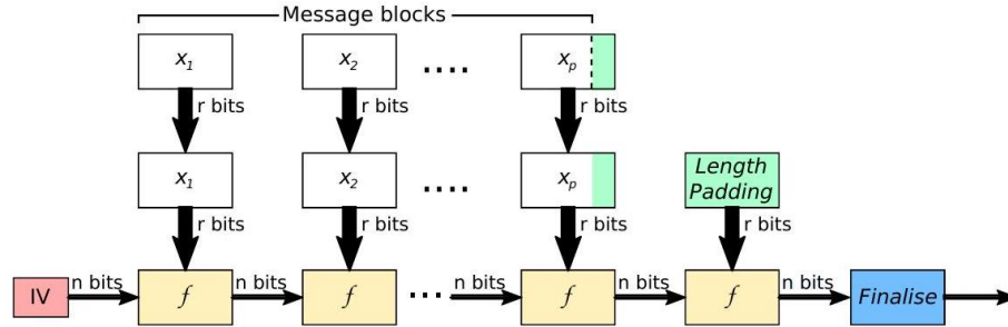
Figure 5.2: Principle of operation of a cryptographic hash function based on the Merkle-Damgaard construction
