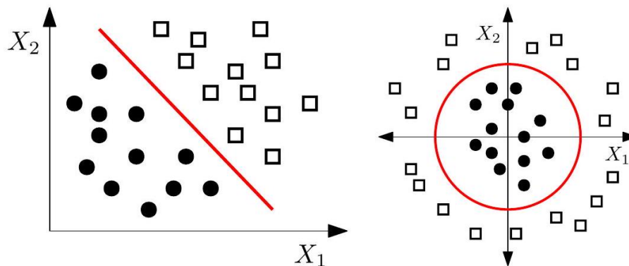
Figure 10.12: A separating line partitions two classes in feature space (left). However, non-linear separators are better at fitting certain training sets (right).
