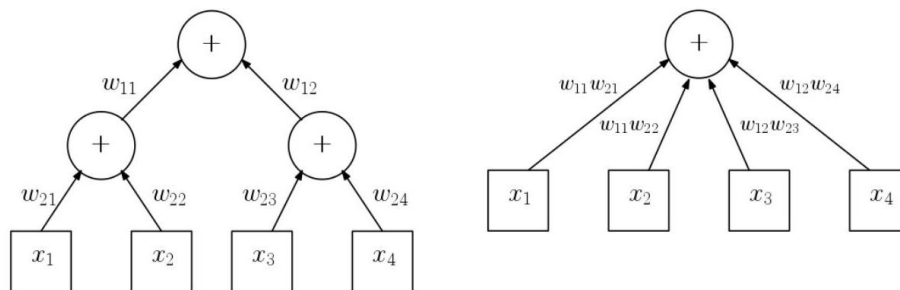
Figure 12.6: Addition networks do not benefit from depth. The two layer network (left) computes exactly the function as the equivalent one layer network (right).
