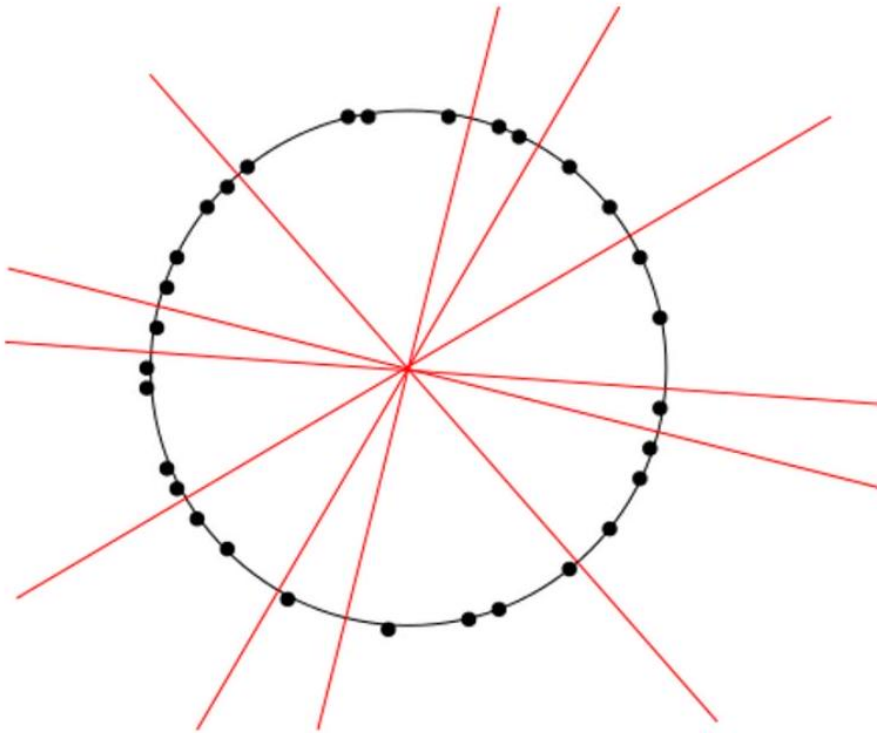
Figure 11.7: Figure 10.7: Nearby points on the circle generally lie on the same side of random lines through the origin. Locality-sensitive hash codes for each point can be composed as a sequence of sidedness tests (left or right) for any specific sequence of lines.
