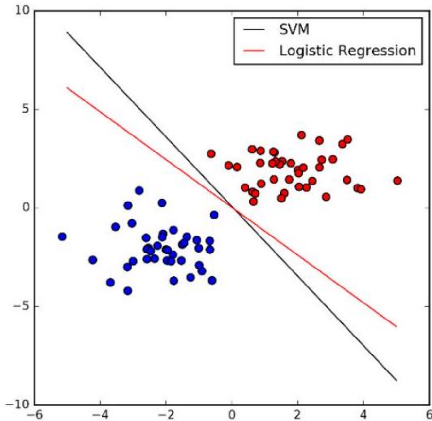
Figure 12.3: Both logistic regression and SVMs produce separating lines between point sets, but optimized for different criteria.
