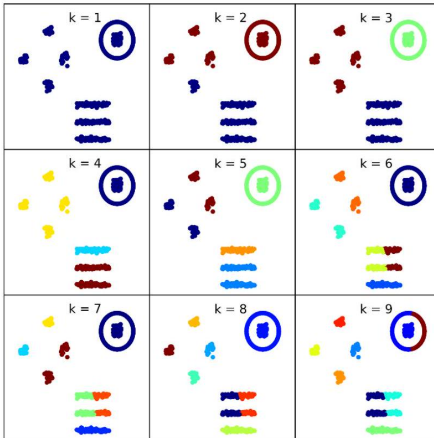
Figure 11.14: Figure 10.15: Running k -means for k = 1 to k = 9 . The “right” clustering is found for k = 3 , but the algorithm is unable to properly distinguish between nested circular clusters and long thin clusters for large k .
