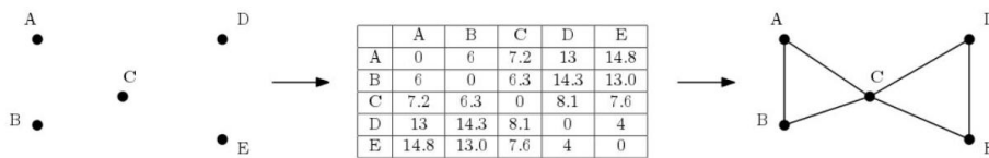
Figure 11.8: The pairwise distances between a set of points in space (left) define a complete weighted graph (center). Thresholding by a distance cutoff removes all long edges, leaving a sparse graph that captures the structure of the points (right).
