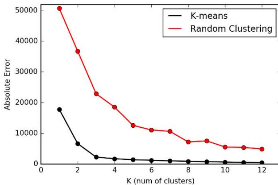
Figure 11.15: Figure 10.16: The error curve for k -means clustering on the point set of Figure 10.12, showing a bend in the elbow reflecting the three major clusters in the data. The error curve for random cluster centers is shown for comparison.
