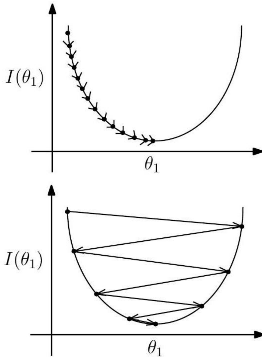
Figure 10.9: The effect of learning rate/step size. Taking too small a step size requires many iterations to converge, while too large a step size causes us to overshoot the minima.
