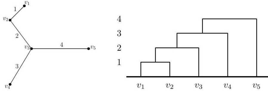
Figure 11.19: Figure 10.20: Kruskal's algorithm for minimum spanning tree is indeed singlelinkage agglomerative clustering, as shown by the cluster tree on right.
