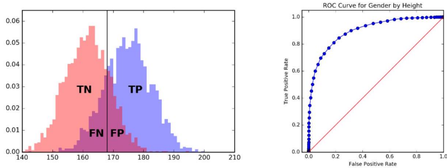
Figure 8.3: The ROC curve helps us select the best threshold to use in a classifier, by displaying the trade-off between true positives and false positive at every possible setting. The monkey ROCs the main diagonal here.
