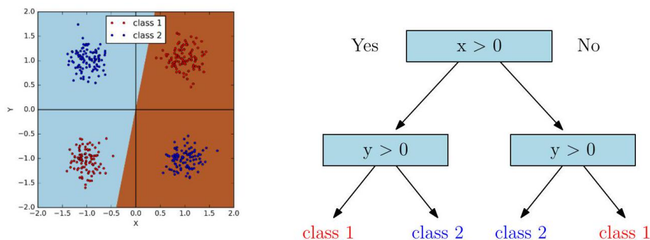
Figure 12.1: The exclusive OR function cannot be fit by linear classifiers. On the left, we present four natural clusters in x - y space. This demonstrates the complete inability of logistic regression to find a meaningful separator, even though a small decision tree easily does the job (right).
