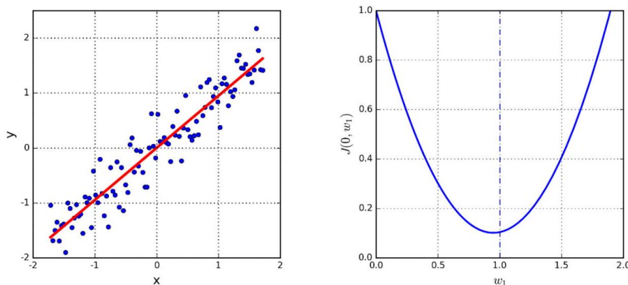
Figure 10.6: The best possible regression line y = w_1 x (left) can be found by identifying the w_1 that minimizes the error of the fit, defined by the minima of a convex function.
