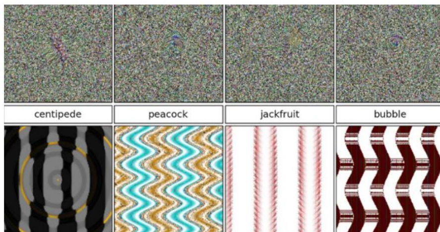
Figure 8.1: Synthetic images that are mistakenly recognized as objects by state-of-the-art Deep Learning neural networks, each with a confidence greater than 99.6%. Source: [?].
