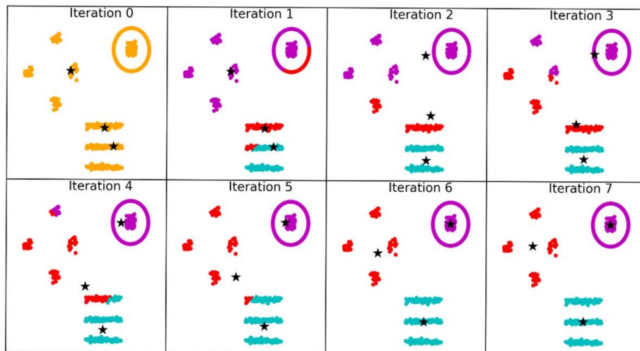
Figure 11.13: The iterations of k -means (for k = 3 ) as it converges on a stable and accurate clustering. Fully seven iterations are needed, because of the unfortunate placement of the three initial cluster centers near the logical center.
