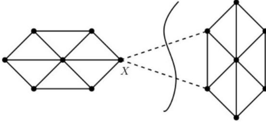
Figure 11.21: Low weight cuts in similarity graphs identify natural clusters.
