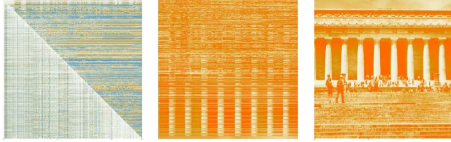
Figure 9.9: Figure 8.11: The LU decomposition of the Lincoln memorial (left), with the product L \cdot U (center). The rows of the LU matrix were permuted during calculation, but when properly ordered fully reconstructed the image (right).
