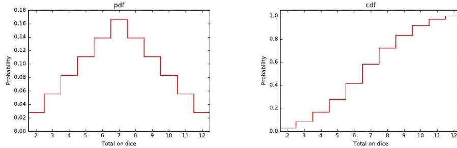
Figure 3.1: The probability density function (pdf) of the sum of two dice contains exactly the same information as the cumulative density function (cdf), but looks very different.
