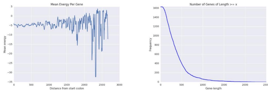
Figure 7.30: Folding energy of genes as a function of their length. Mistaking variance for signal: the extreme values in the left figure are artifacts from averaging small numbers of samples.
