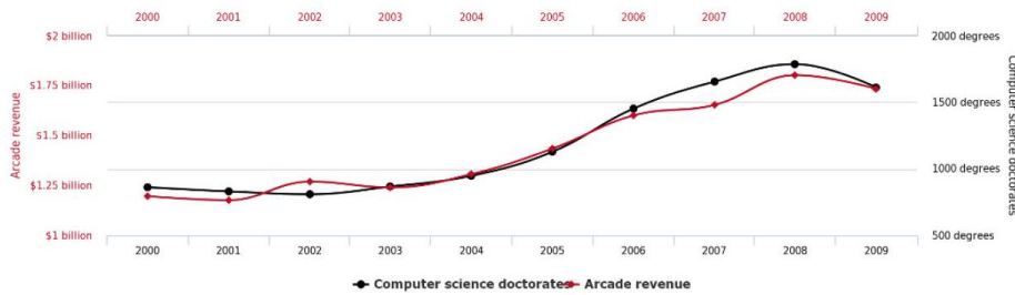
Figure 6.10: Correlation vs. causation: the number of Computer Science Ph.D.s awarded each year in the United States strongly correlates with video/pinball arcade revenue. (from [?])
