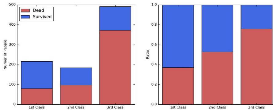
Figure 7.17: Stacked bar charts illustrating the survivorship rate on the doomed ship Titanic, by ticket class. The histogram (left) informs us of the size of each class, but scaled bars (right) better capture proportions. Primary conclusion: you were better off not to be traveling steerage (third class).
