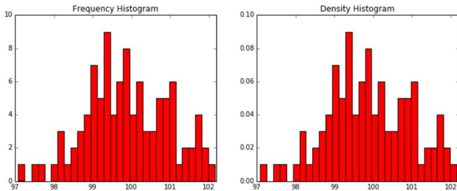
Figure 7.21: Dividing counts by the total yields a probability density plot, which is more generally interpretable even though the shapes are identical.
