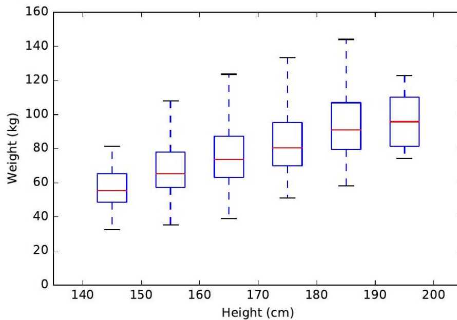
Figure 7.11: Box and whisker plots concisely show the range/quartiles (i.e. median and variance) of a distribution. (hairs) are added to show the range of the highest and lowest values. Figure 6.13 shows a box-and-whisker plot of weight as a function of height in a population sample. The median weight increases with height, but not the maximum, because fewer points in the tallest bucket reduces the chance for an outlier maximum value.
