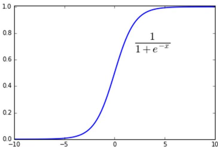
Figure 10.14: The logit function maps a score to a probability.
