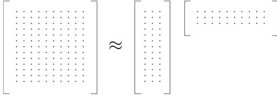
Figure 9.8: Factoring a feature matrix A \approx BC yields B as a more concise representation of the items and C as a more concise representations of the features A^T .
