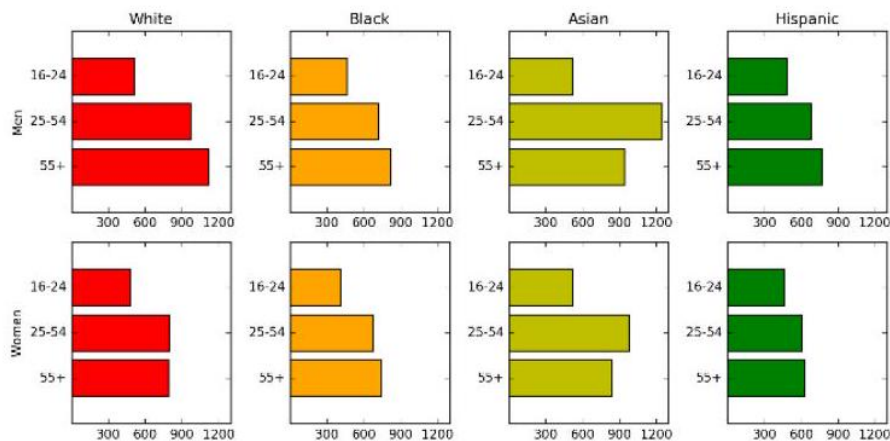
Figure 7.16: Small multiple bar plots/tables are excellent ways to represent multivariate data for comparison.
