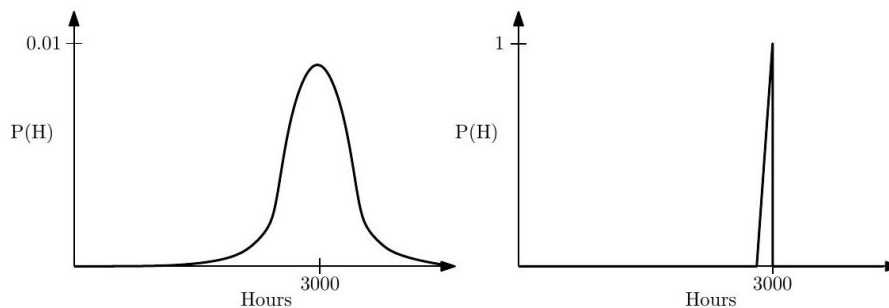
Figure 3.3: Two distinct probability distributions with \mu = 3000 for the lifespan of light bulbs: normal (left) and with zero variance (right).
