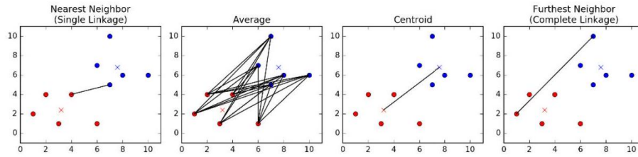
Figure 11.17: Four distance measures for identifying the nearest pair of clusters.
