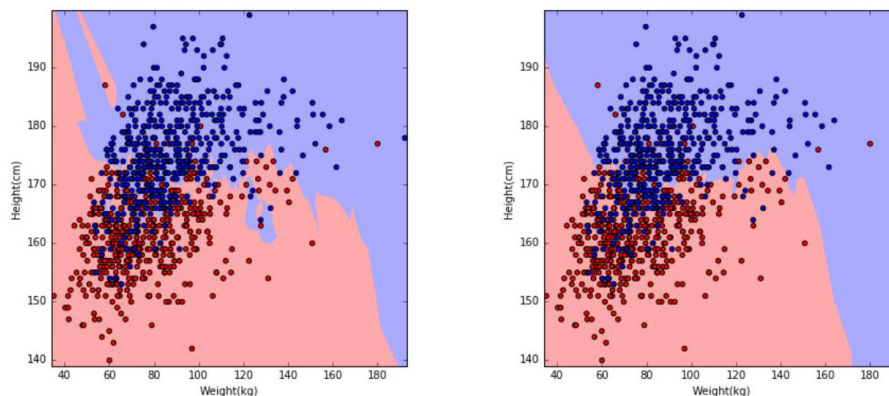
Figure 11.4: Figure 10.4: The effect of k on the decision boundary for gender classification using k -NN. Compare k = 3 (left) and k = 10 (right) with k = 1 in Figure 10.3.
