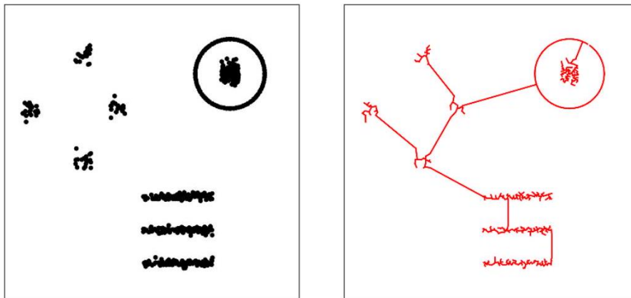
Figure 11.18: Figure 10.19: Single linkage clustering is equivalent to finding the minimum spanning tree of a network.
