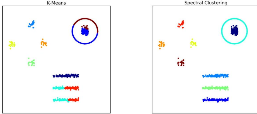
Figure 11.20: The results of k -means (left) and cut-based spectral clustering (right) on our 9 -cluster example. Spectral clustering correctly finds connected clusters here that k -means cannot.
