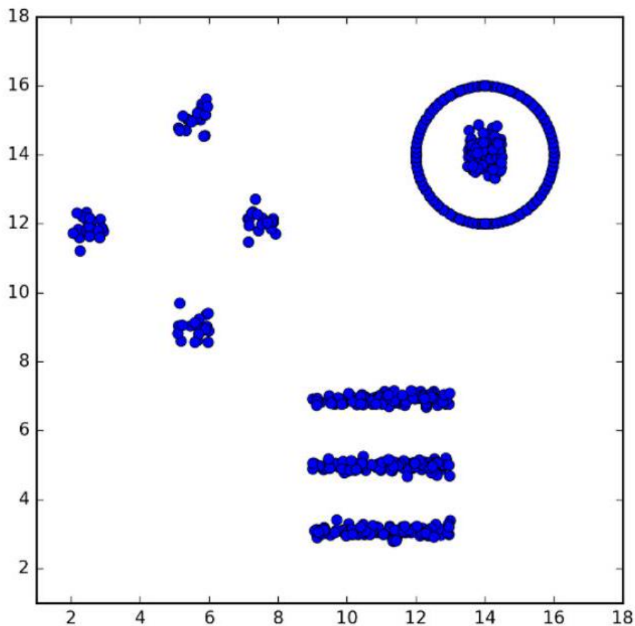
Figure 11.12: How many clusters do you see here?
