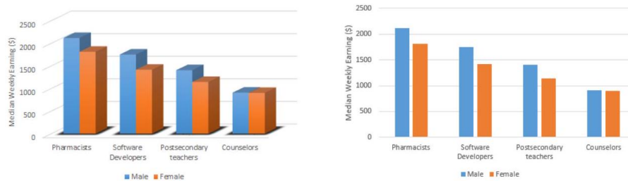
Figure 7.3: Three-dimensional monoliths casting rendered shadows (l) may look impressive. But they really are just chartjunk, which serves to reduce the clarity and data-ink ratio from just showing the data (r).
