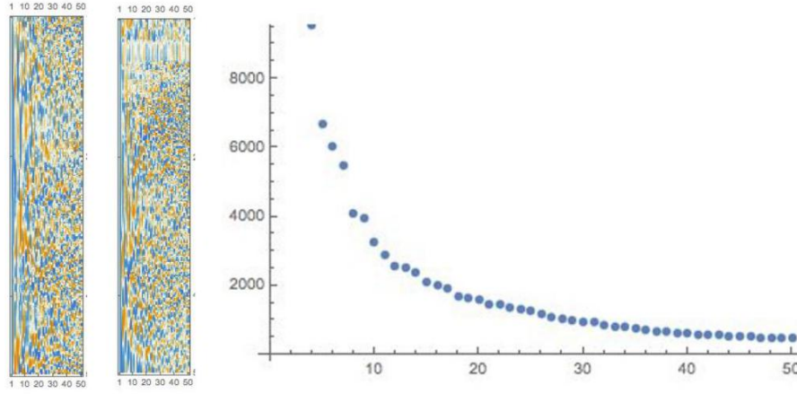
Figure 9.12: Singular value matrices in the decomposition of Lincoln, for 50 singular values.
