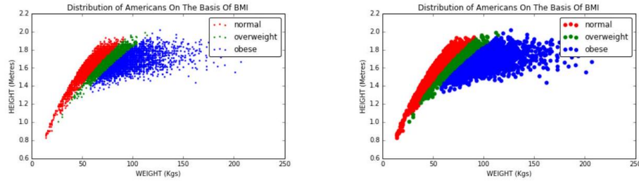
Figure 7.12: Smaller dots on scatter plots (left) reveal more detail than the default dot size (right).
