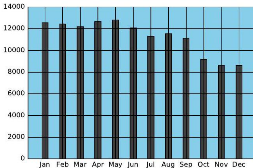
Figure 7.5: A monthly time series of sales. How can we improve/simplify this bar chart time series?
