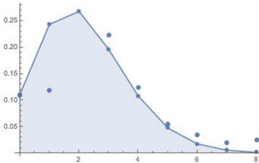
Figure 6.6: Figure 5.6: The observed fraction of families with x kids (isolated points) is accurately modeled by Poisson distribution, defined by an average of \mu = 2.2 children per family (polyline).
