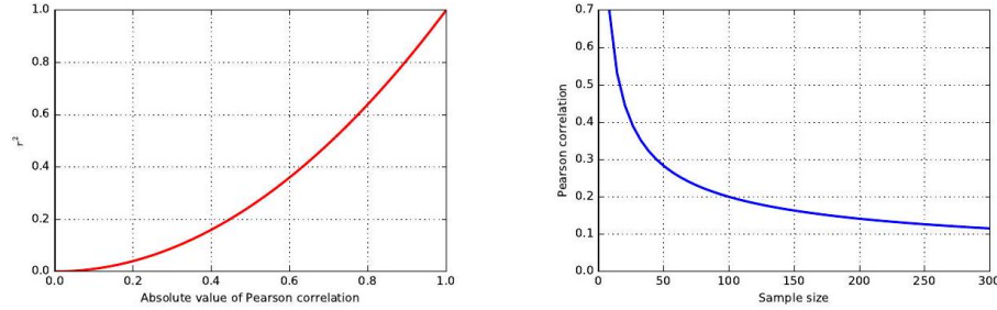
Figure 3.6: Limits in interpreting significance. The r^2 value shows that weak correlations explain only a small fraction of the variance (left). The level of correlation necessary to be statistically significance decreases rapidly with sample size n (right).
