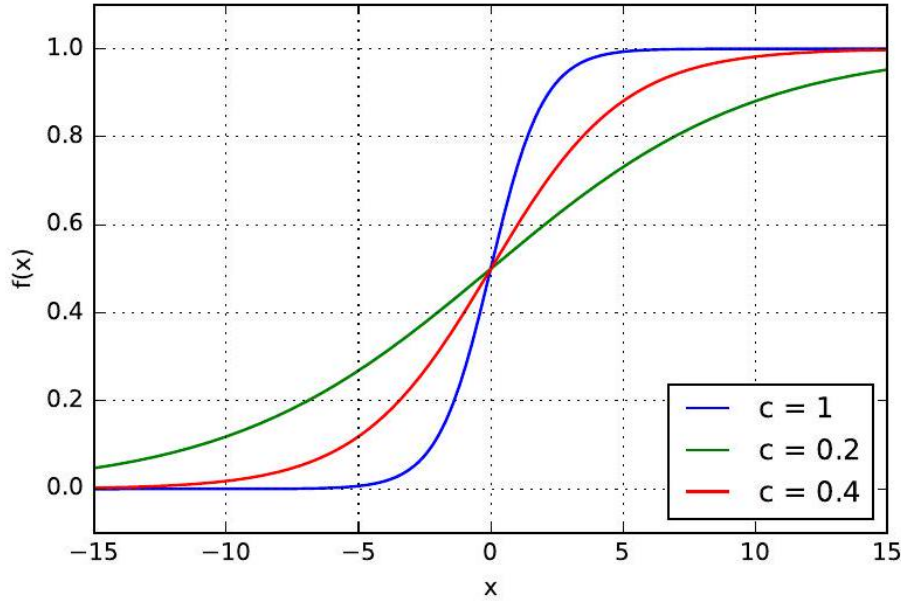
Figure 5.4: The shape of the logit function, for three different values for c .
