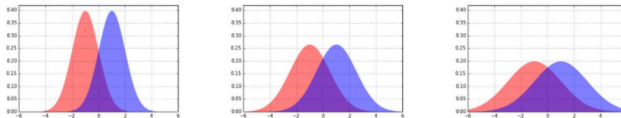
Figure 6.12: Pairs of normal distributions with the same difference in their means but increasing variance, from left to right. As the variance increases, there becomes greater overlap between the distributions, making it harder to tell them apart.
