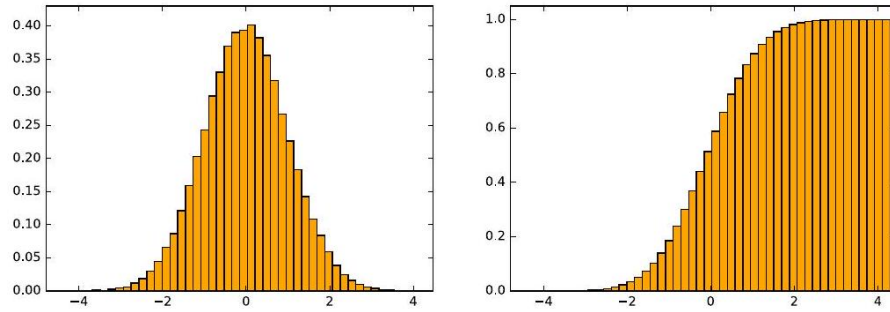
Figure 7.22: Generally speaking, histograms are better for displaying peaks in a distribution, but cdfs are better for showing tails.
