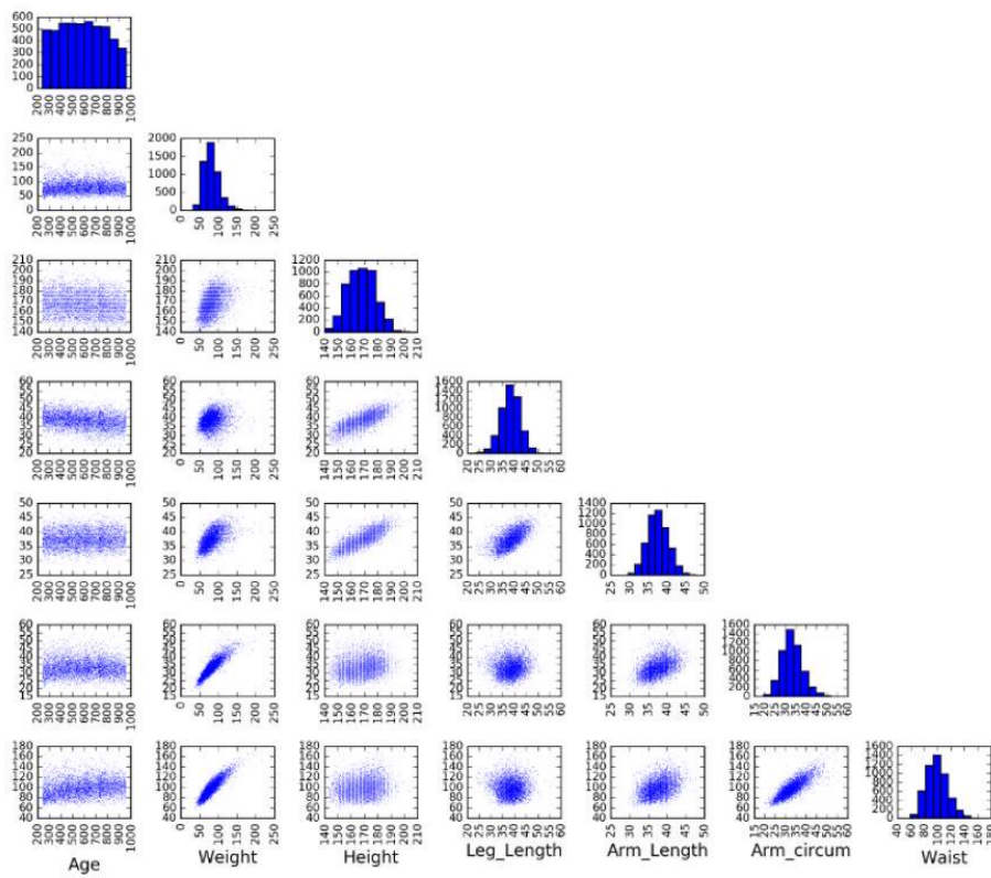
Figure 7.1: The array of dot plots of variable pairs provides quick insight into the distributions of data values and their correlations.
