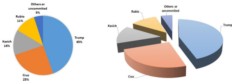
Figure 7.18: Pie charts of delegates to the 2016 Republican convention by candidate. Which one is better and why?
