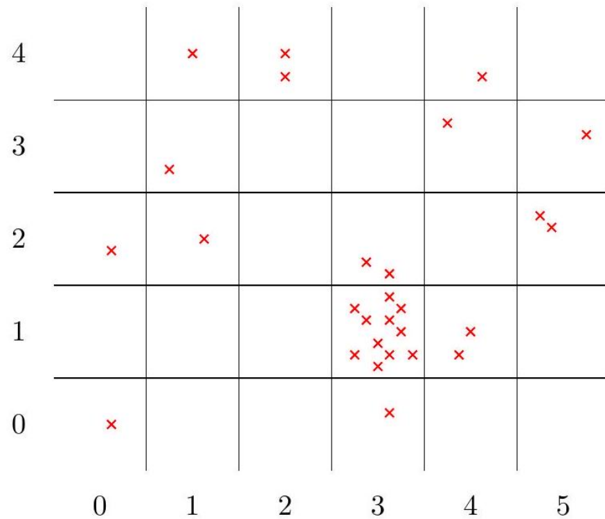
Figure 11.6: A grid index data structure provides fast access to nearest neighbors when the points are uniformly distributed, but can be inefficient when points in certain regions are densely clustered.
