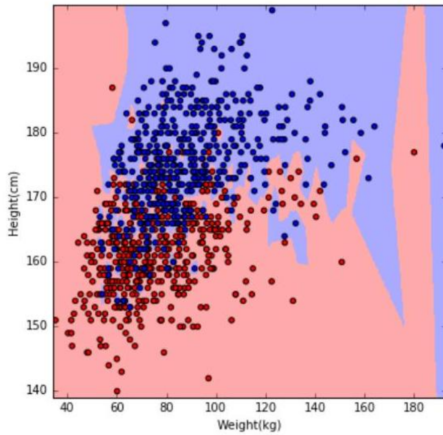
Figure 11.3: The decision boundary of nearest-neighbor classifiers can be non-linear.
