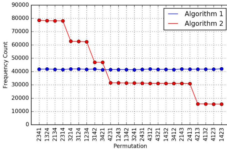
Figure 6.16: The generation frequency of all 4! = 24 permutations using two different algorithms. Algorithm 1 generates them with uniform frequency, while algorithm 2 is substantially biased.
