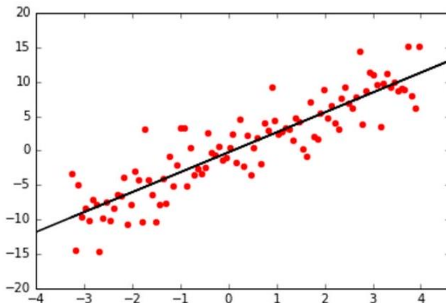
Figure 10.1: Linear regression produces the line which best fits a set of points.
