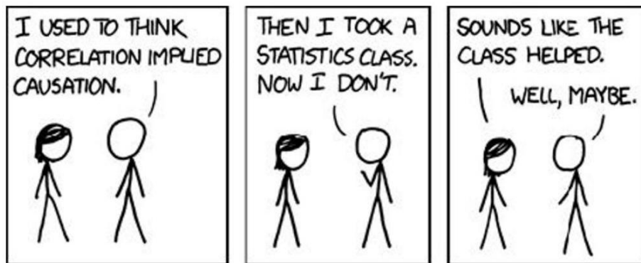
Figure 3.8: Correlation does not imply causation. (Source https://www.xkcd.com/552 .)
