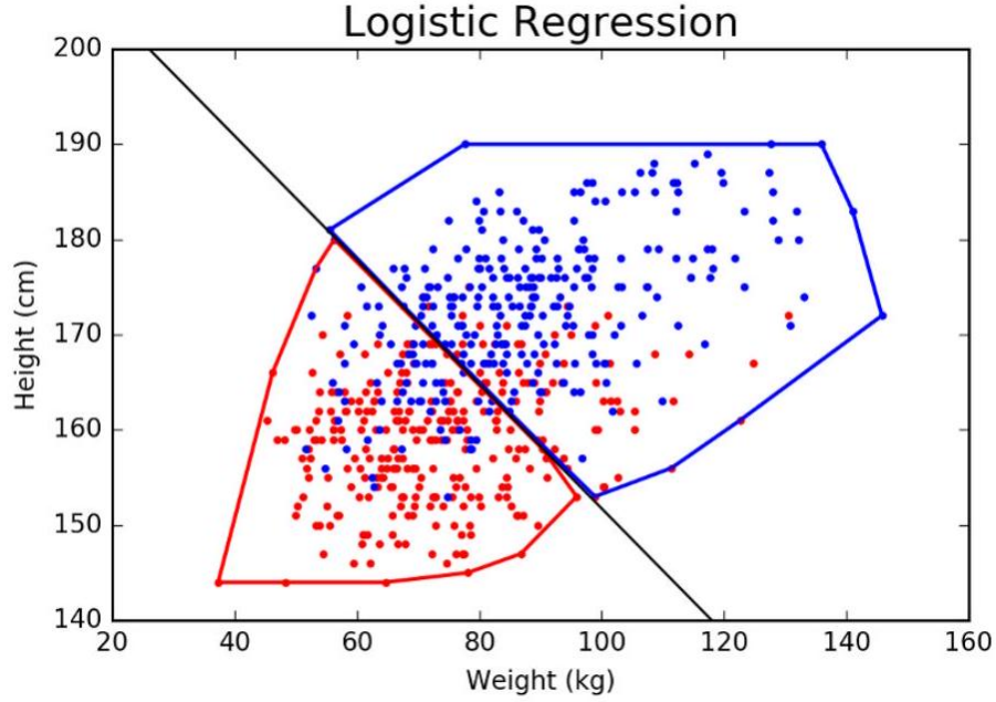
Figure 10.16: The logistic regression classifier best separating men and women in weight-height space. The red region contains 229 women and only 63 men, while the blue region contains 223 men to 65 women.
