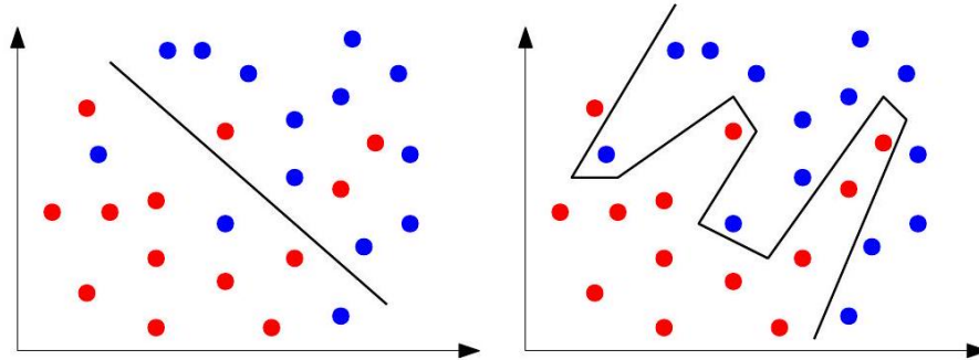
Figure 10.13: Linear classifiers cannot always separate two classes (left). However, perfect separation achieved using complex boundaries usually reflects overfitting more than insight (right).
