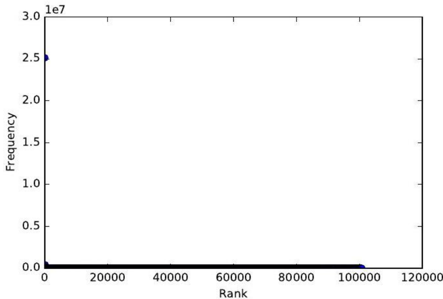
Figure 7.28: A dotplot of word frequency by rank. What do you see?
