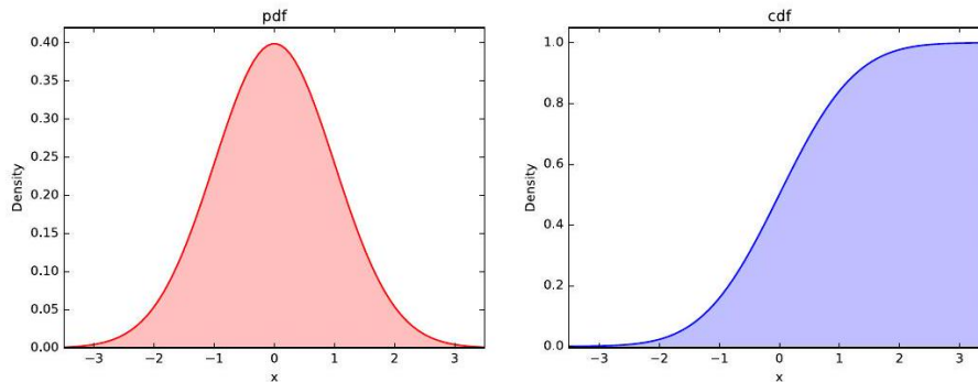
Figure 6.3: The probability density function (pdf) of the normal distribution (left) with its corresponding cumulative density function (cdf) on right.
