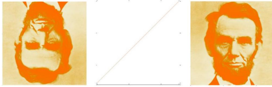
Figure 9.6: Multiplying the Lincoln matrix M by the reverse permutation matrix r (center). The product r \cdot M flips Lincoln upside down (left), while M \cdot r parts his hair on the other side of his head (right).
