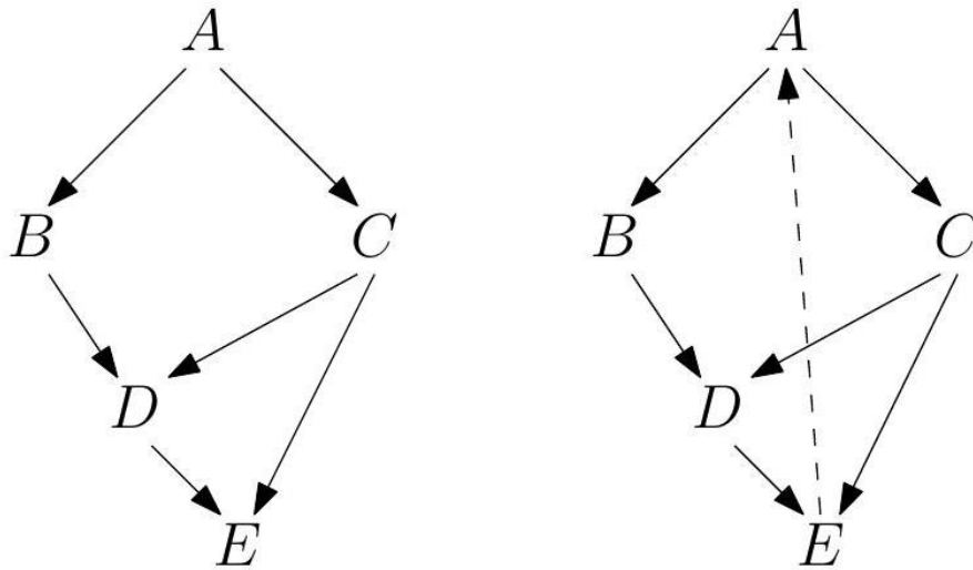
Figure 5.5: Consistently ordered preferences yield an acyclic graph or DAG (left). Inconsistent preferences result in directed cycles, which can be broken by deleting small sets of carefully selected edges, here shown dashed (right).
