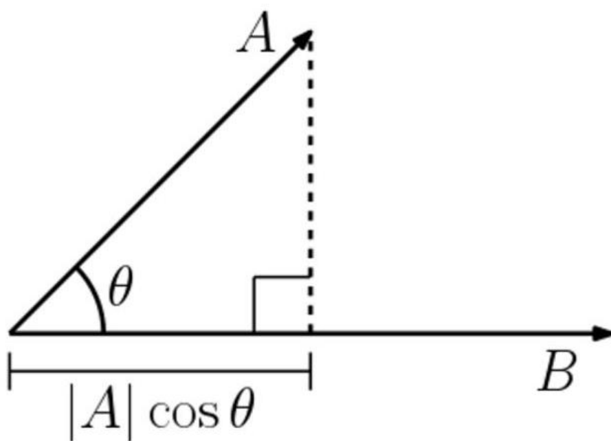
Figure 9.2: The dot product of two vectors defines the cosine of the angle between them.
