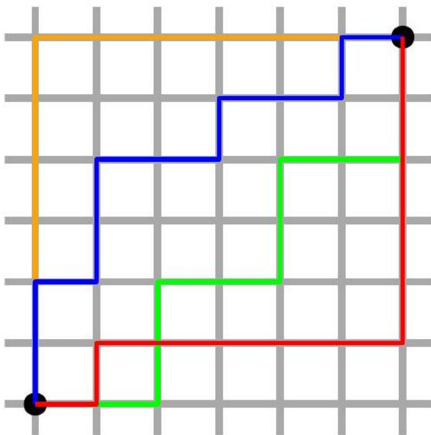
Figure 11.1: Many different paths across a grid have equal Manhattan ( L_1 ) distance.
