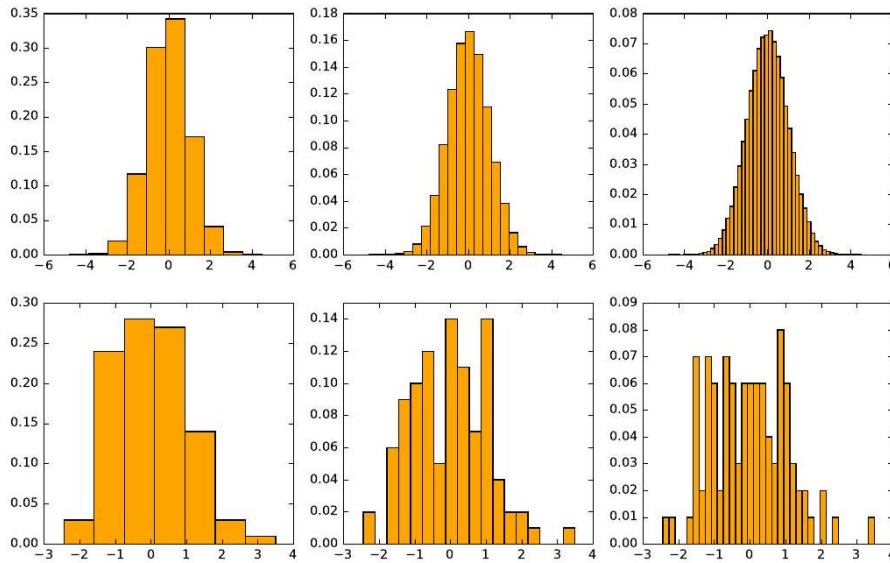
Figure 7.20: Histograms of a given distribution can look wildly different depending on the number of bins. A large data set benefits from many bins (top). But the structure of a smaller data set is best shown when each bin a non-trivial number of element.
