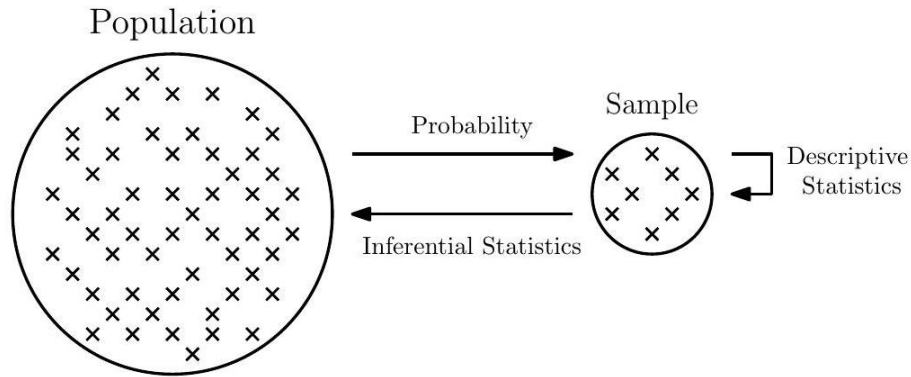
Figure 6.1: The central dogma of statistics: analysis of a small random sample enables drawing rigorous inferences about the entire population.
