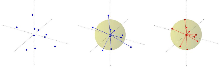
Figure 9.1: Points can be reduced to vectors on the unit sphere, plus magnitudes.
