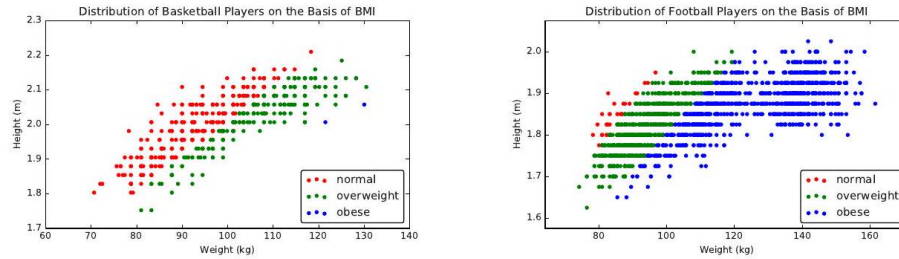
Figure 5.2: BMI distributions of professional basketball (left) and football (right) players.
