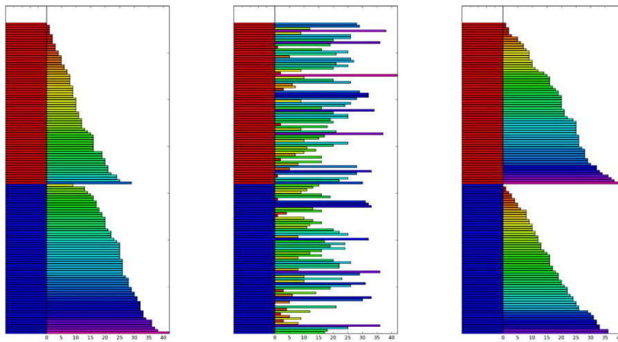
Figure 6.14: Permutation tests reveal the significance of the correlation between gender and the height (left). A random assignment of gender to height (center) results in a substantially different distribution of outcomes when sorted (right), validating the significance of the original relationship. c = 65 single cousins (or 32.5 married pairs) suffice, once the children have been excluded ( f = 0.672 ).
