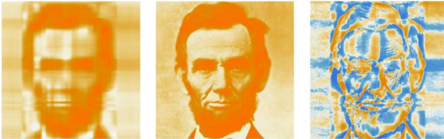
Figure 9.13: Lincoln's face reconstructed from 5 (left) and 50 (center) singular values, with the error for k = 50 (right).
