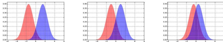
Figure 6.11: Pairs of normal distributions with the same variance, but decreasing difference in their means from left to right. As the means get closer, the greater overlap between the distributions makes it harder to tell them apart.
