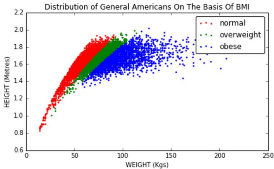
Figure 5.1: Figure 4.1: Height-weight scatter plot, for 1000 representative Americans. Colors illustrate class labels in the BMI distribution.
