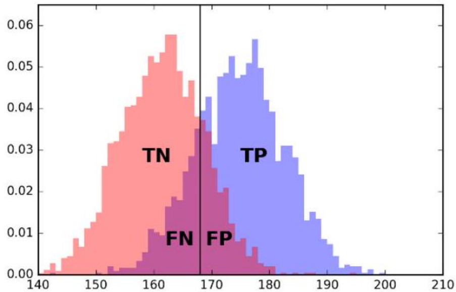
Figure 8.2: What happens if we classify everyone of height \geq 168 centimeters as male? The four possible results in the confusion matrix reflect which instances were classified correctly (TP and TN) and which ones were not (FN and FP).
