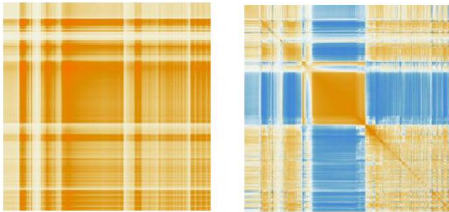
Figure 9.10: The Lincoln memorial's biggest eigenvector suffices to capture much of the detail of its covariance matrix.
