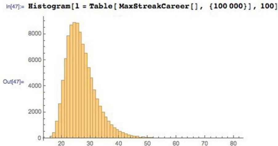
Figure 6.17: Figure 5.18: The distribution of longest hitting streaks, over 100,000 simulated careers. DiMaggio's actual 56-game hitting streak stands at the very tail of this distribution, thus demonstrating the difficulty of this feat.
