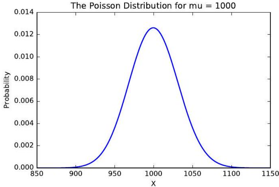
Figure 6.5: The lifespan distribution of lightbulbs with an expected life of \mu = 1000 hours, as modeled by a Poisson distribution.
