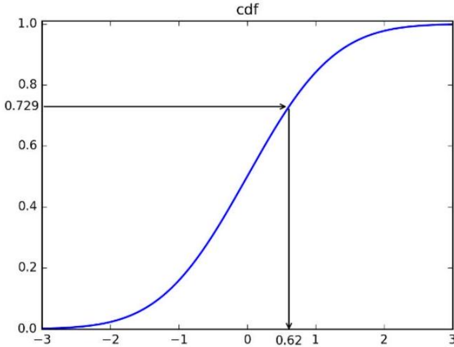
Figure 6.8: The inverse transform sampling method enables us to convert a random number generated uniformly from [0, 1] (here 0.729) to a random sample drawn from any distribution, given its cdf.
