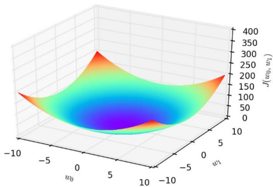
Figure 10.7: Linear regression defines a convex parameter space, where each point represents a possible line, and the minimum point defines the best fitting line.
