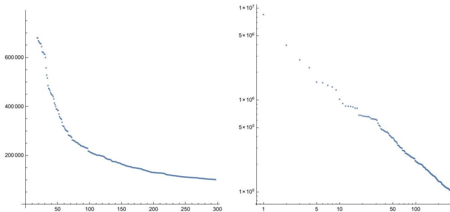
Figure 6.7: Figure 5.7: The population of U.S. cities by decreasing rank (left). On the right is the same data, now including the very largest cities, but plotted on a log-log scale. That they sit on a line is indicative of a power law distribution.
