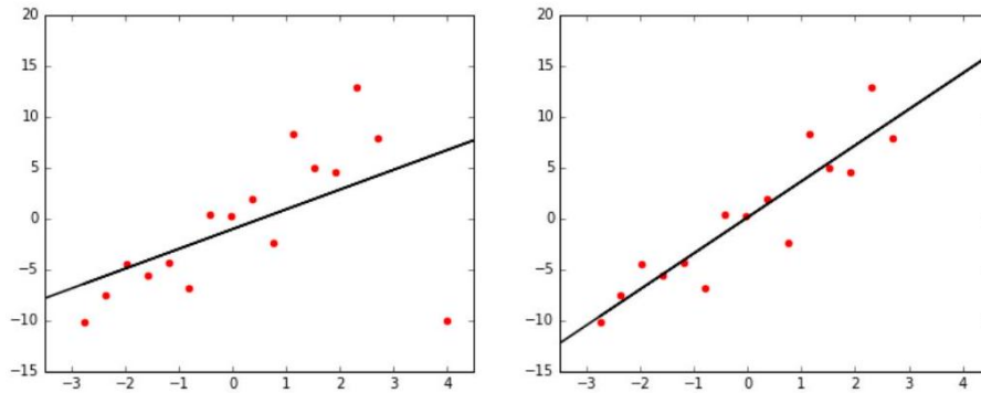
Figure 10.4: Removing outlier points (left) can result in much more meaningful fits (right).
