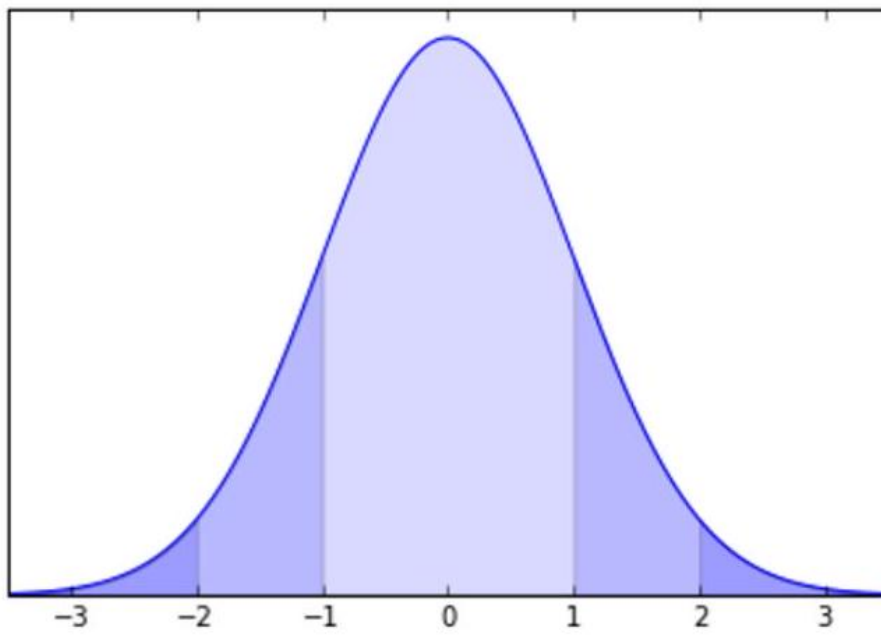
Figure 6.4: The normal distribution implies tight bounds on the probability of lying far from the mean. 68% of the values must lie within one sigma of the mean, and 95% within 2\sigma , and 99.7% within 3\sigma .
