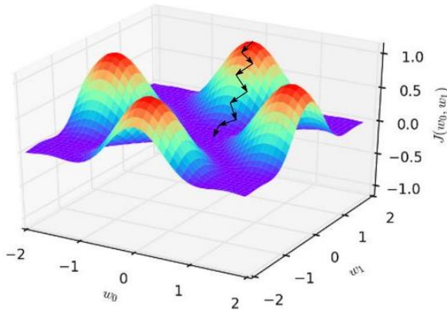
Figure 10.10: Gradient descent search finds local minima for non-convex surfaces, but does not guarantee a globally optimum solution.
