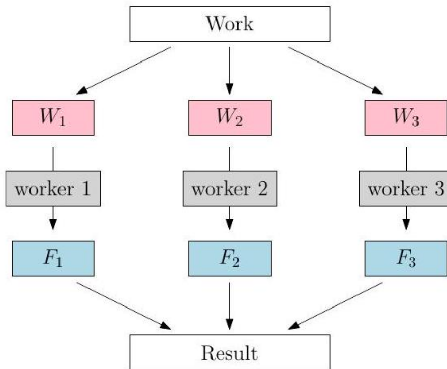
Figure 13.1: Divide and conquer is the algorithmic paradigm of distributed computing.
