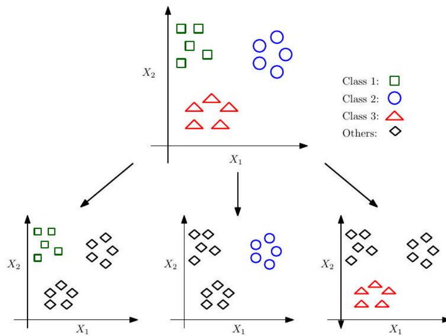
Figure 10.18: Voting among multiple one-vs.-rest classifiers is generally the best way to do multi-class classification.
