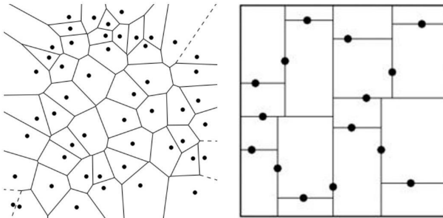
Figure 11.5: Data structures for nearest neighbor search include Voronoi diagrams (left) and kd -trees (right).
