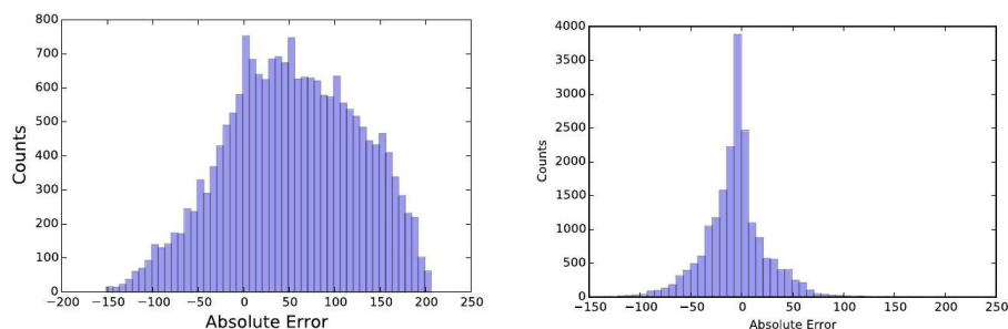
Figure 8.4: Error distribution histograms for random (left) and naive Bayes classifiers predicting the year of authorship for documents (right).
