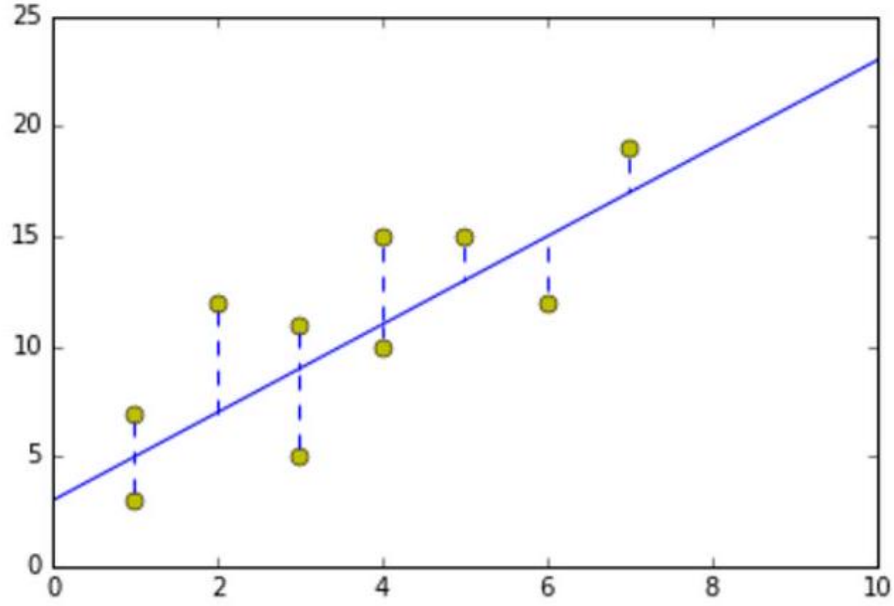
Figure 10.3: The residual error in least squares is the projection of y_i - f(X) down to X , not the shortest distance between the line and the point.
