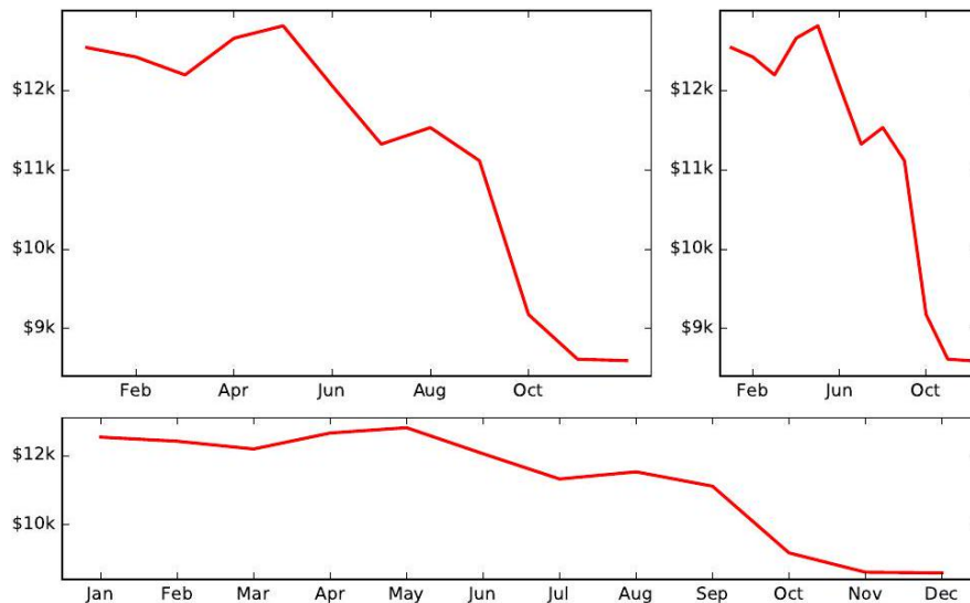
Figure 7.4: Three renderings of the same financial time series. Which most accurately represents the situation?
