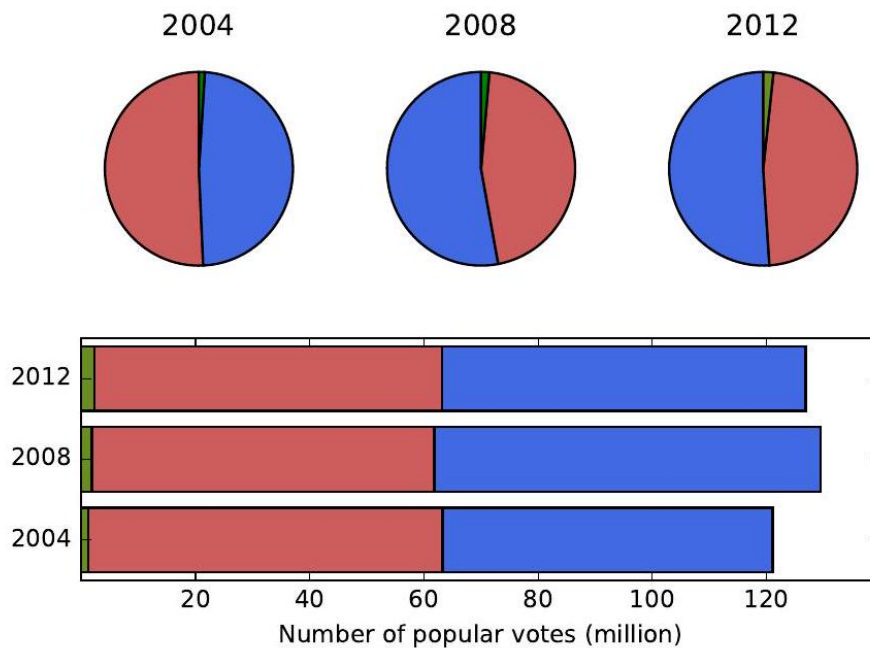
Figure 7.15: Voter data from three U.S. presidential elections. Bar plots and pie charts display the frequency or proportion of categorical variables. Relative magnitudes in a time series can be displayed by modulating the area of the line or circle.
