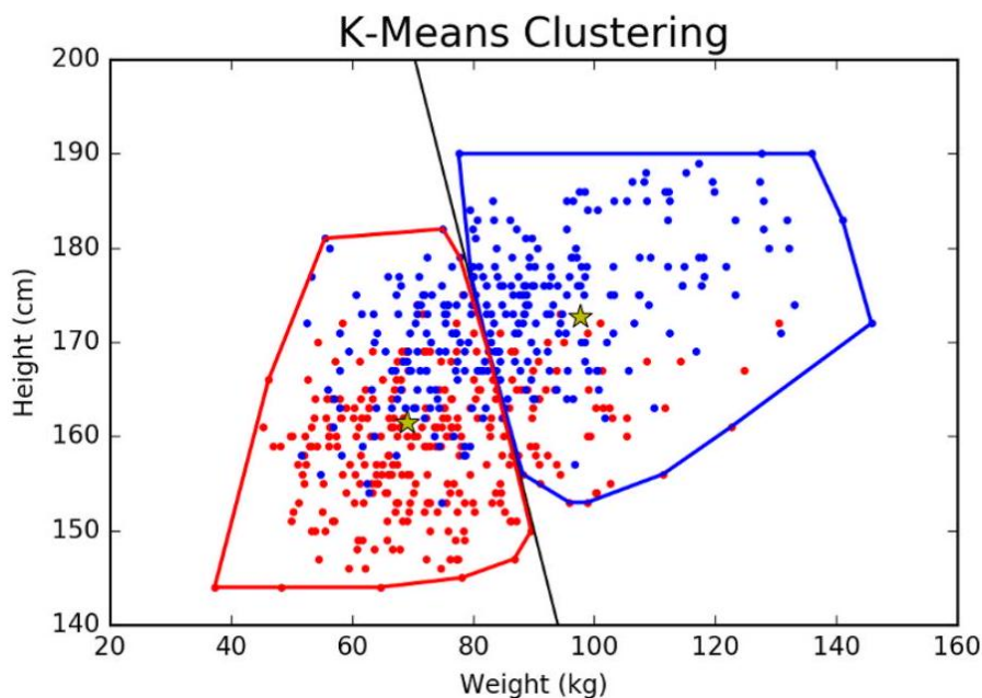
Figure 11.11: Figure 10.11: Clustering people in weight-height space, using 2-means clustering. The left cluster contains 240 women and 112 men, while the right cluster contains 174 men to 54 women. Compare this to the logistic regression classifier trained on this same data set, in Figure 9.17.
