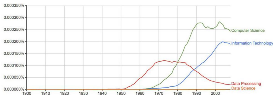
Figure 2.5: The rise and fall of data processing, as witnessed by Google Ngrams.
