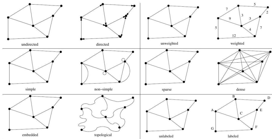
Figure 11.9: Figure 10.9: Important properties/flavors of graphs
