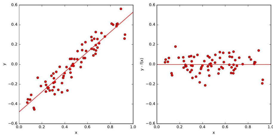
Figure 3.7: Plotting r_i = y_i - f(x_i) shows that the residual values have lower variance and mean zero. The original data points are on the left, with the corresponding residuals on the right.
