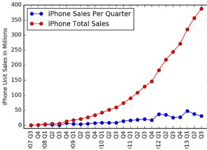
Figure 3.2: iPhone quarterly sales data presented as cumulative and incremental (quarterly) distributions. Which curve did Apple CEO Tim Cook choose to present?
