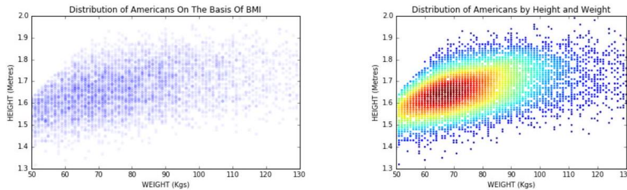
Figure 7.13: Overlapping dots can obscure scatter plots, particularly for large data sets. Reducing the opacity of the dots (left) shows some of the fine structure of the data (left). But a colored heatmap more dramatically reveals the distribution of the points (right).
