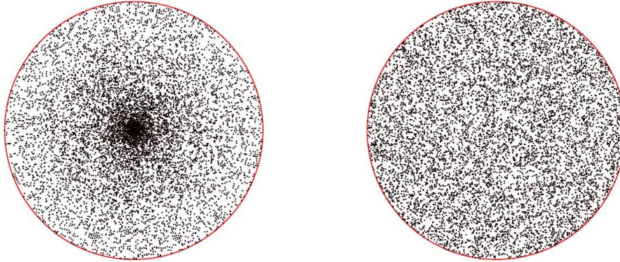
Figure 6.9: Randomly generating 10,000 points by angle-radius pairs clearly oversamples near the origin of the circle (left). In contrast, Monte Carlo sampling generates points uniformly within the circle (right).
