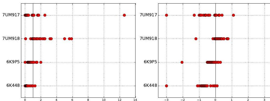
Figure 3.10: Plotting ratios on a scale cramps the space allocated to small ratios relative to large ratios (left). Plotting the logarithms of ratios better represents the underlying data (right).
