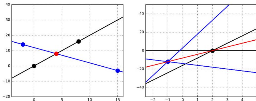
Figure 10.2: Points are equivalent to lines under a duality transform. The point (4, 8) in red (left) maps to the red line y = 4x - 8 on right. Both sets of three collinear points on the left correspond to three lines passing through the same point on right.
