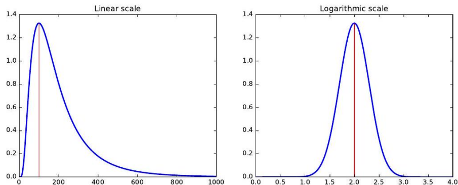
Figure 3.11: Hitting a skewed data distribution (left) with a log often yields a more bell-shaped distribution (right).
