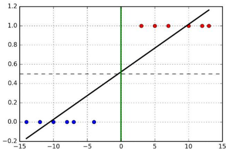
Figure 10.11: The optimal regression line cuts through the classes, even though a perfect separator line ( x = 0 ) exists.
