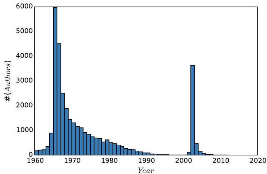
Figure 4.2: What artifacts can you find in this time series, counting the number of author's names first appearing in the scientific literature each year?
