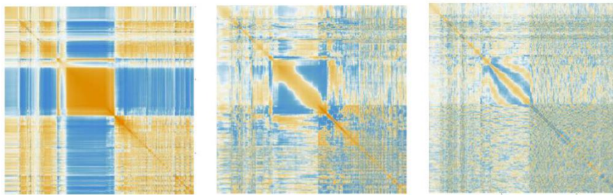
Figure 9.11: Error in reconstructing the Lincoln memorial from the one, five, and fifty largest eigenvectors.
