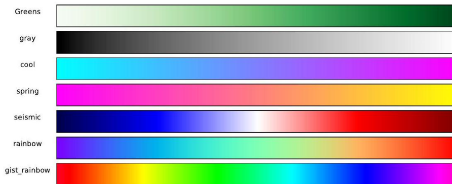
Figure 7.8: Color scales from Python's Matplotlib, varying hue, saturation, and brightness. Rainbow color maps are perceptually non-linear, making it difficult to recognize the magnitudes of differences.
