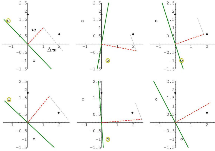
Figure 9.10: Application of the perceptron learning rule to two positive ( \cdot ) and two negative ( \circ ) data points. The solid line shows the current dividing line wx = 0 . The orthogonal dashed line is the weight vector w and the second dashed line the change vector \Delta w = x or \Delta w = -x to be added, which is calculated from the currently active data point surrounded in light green
