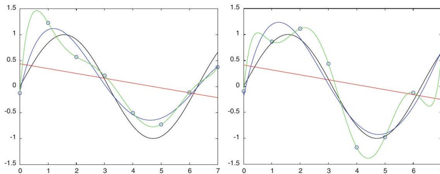
Figure 9.25: Two different data sets approximated by polynomials of degree 1, 4 and 7. The bias variance tradeoff is clearly visible
