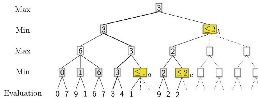
Figure 7.14: A minimax game tree with look-ahead of four half-moves
