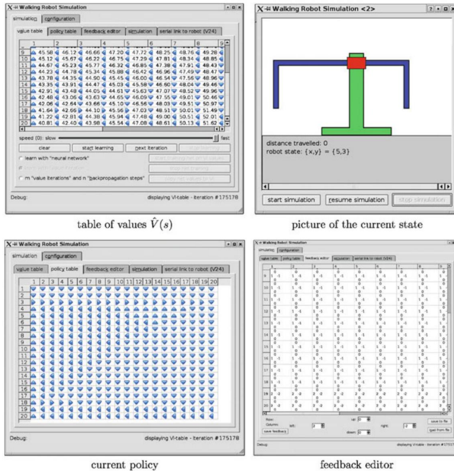
Figure 11.7: Four different windows of the walking robot simulator
