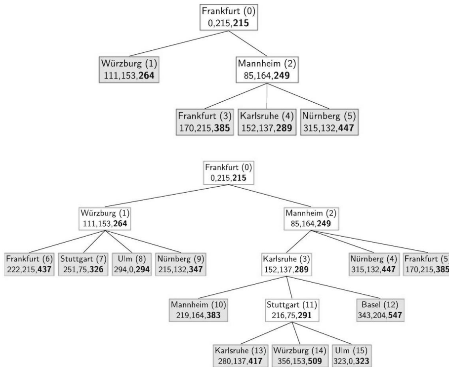
Figure 7.11: Two snapshots of the A^* search tree for the optimal route from Frankfurt to Ulm. In the boxes below the name of the city s we show g(s) , h(s) , f(s) . Numbers in parentheses after the city names show the order in which the nodes have been generated by the "Successor" function
