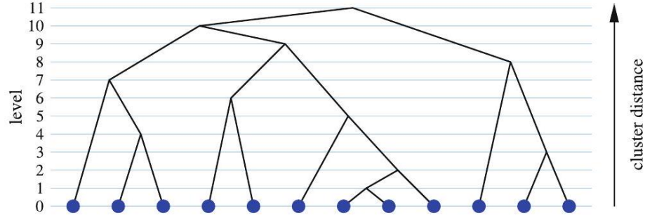
Figure 9.32: In hierarchical clustering, the two clusters with the smallest distance are combined in each step
