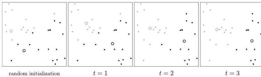
Figure 9.31: k-means with two classes ( k = 2 ) applied to 30 data points. Far left is the dataset with the initial centers, and to the right is the cluster after each iteration. After three iterations convergence is reached
