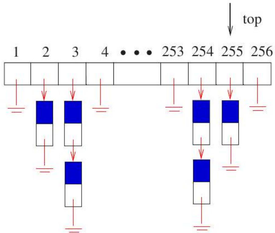
Figure 6.8: A bounded-height priority queue for triangle strips.
