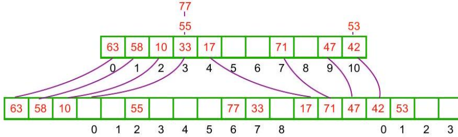
Figure 9.8: Perfect hashing uses a two-level hash table to guarantee lookup in constant time. The first-level table encodes an index range of l_i^2 elements in the second-level table, allocated to store the l_i items in first-level bucket i .
