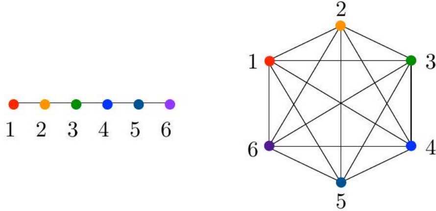
Figure 9.4: How long does a random walk take to visit all n nodes of a path (left) or a complete graph (right)?
