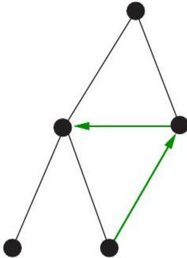
Figure 10.13: The possible edge cases for graph traversal. Forward edges and cross edges can occur in DFS only on directed graphs .
