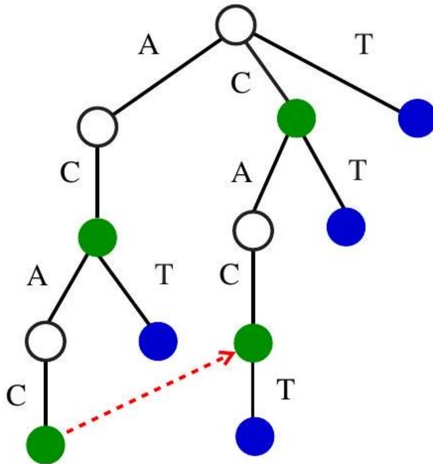
Figure 6.11: Suffix tree on ACAC and CACT , with the pointer to the suffix of ACAC . Green nodes correspond to suffixes of ACAC , with blue nodes to suffixes of CACT .
