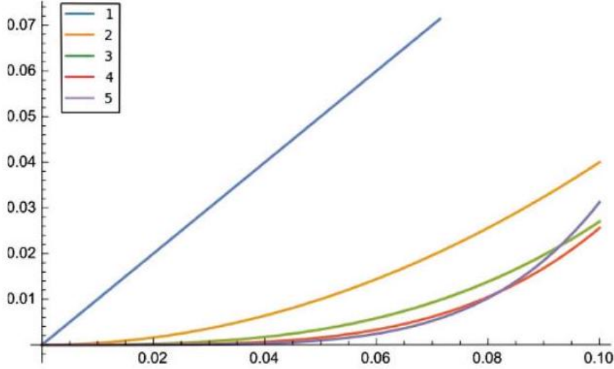
Figure 9.6: Bloom filter error probability as a function of load ( m/n ) for k from 1 to 5 . By selecting the right k for the given load, we can dramatically reduce false positive error rate with no increase in table space.
