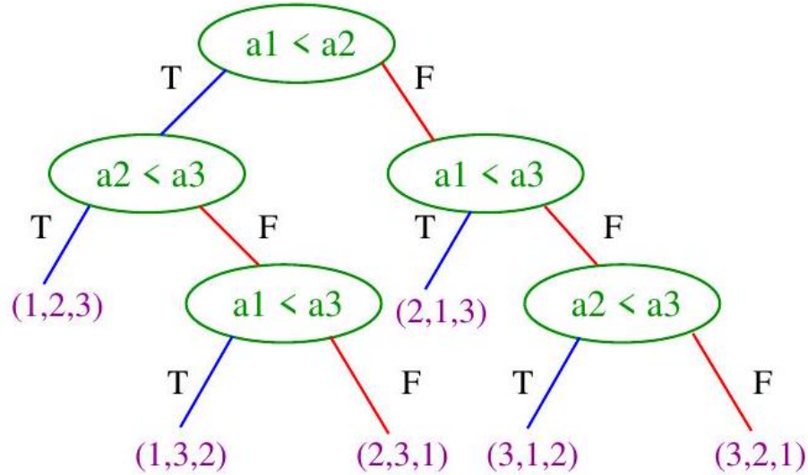
Figure 7.8: Interpreting insertion sort of input array a as a decision tree. Each leaf represents a given input permutation, while the root-to-leaf path describes the sequence of comparisons the algorithm does to sort it.
