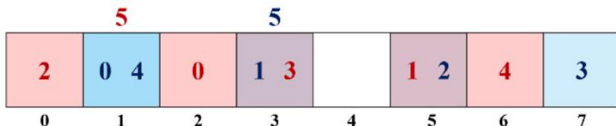
Figure 9.5: Hashing the integers 0, 1, 2, 3, and 4 into an n = 8 bit Bloom filter, using hash functions h_1(x) = 2x + 1 (blue) and h_2(x) = 3x + 2 (red). Searching for x = 5 would yield a false positive, since the two corresponding bits have been set by other elements.
