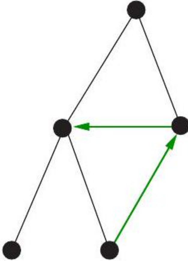
Figure 7.14: The possible edge cases for graph traversal. Forward edges and cross edges can occur in DFS only on directed graphs.
