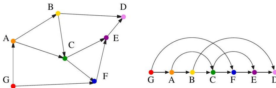
Figure 7.15: A DAG with only one topological sort (G, A, B, C, F, E, D) connected component as the starting point. Both must start with a vertex in each component to traverse a disconnected graph. The only important difference between them is the way they organize and label the edges.
