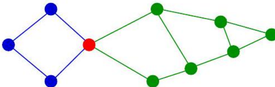
Figure 7.11: An articulation vertex is the weakest point in the graph. edge going from x to an ancestor y creates a cycle with the tree path from y to x . Such a cycle is easy to find using dfs:
