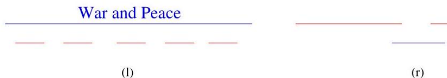
Figure 1.6: Bad instances for the (l) earliest job first and (r) shortest job first heuristics. The optimal solutions are in red.
