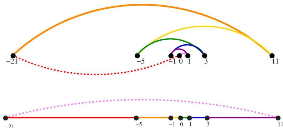
Figure 1.3: A bad instance for the nearest-neighbor heuristic, with the optimal solution. Colors are sequenced as ordered in the rainbow. this:
