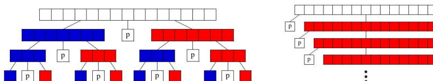
Figure 4.6: The best-case (left) and worst-case (right) recursion trees for quicksort. The left partition is in blue and the right partition in red. can halve n until we get down to 1, meaning h = \lceil \lg n \rceil . This happy situation is shown in Figure 4.6(left), and corresponds to the best case of quicksort.
