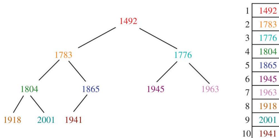
Figure 4.2: A heap-labeled tree of important years from American history (left), with the corresponding implicit heap representation (right). array of keys, and use the position of the keys to implicitly play the role of the pointers.
