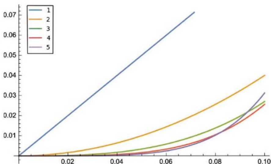
Figure 6.7: Bloom filter error probability as a function of load (m/n) for k from 1 to 5. By selecting the right k for the given load, we can dramatically reduce false positive error rate with no increase in table space. saying yes when the answer is no.
