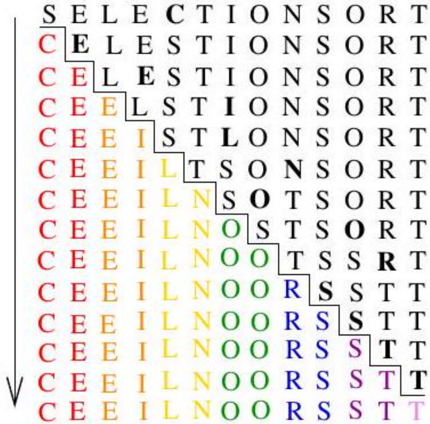
Figure 2.5: Animation of selection sort in action.
