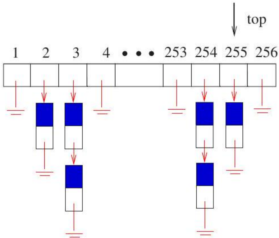
Figure 3.8: A bounded-height priority queue for triangle strips. that it would be fast and simple, although there is no reason to expect that it must find the smallest possible set of left-right strips for a given triangulation. The greedy heuristic should result in a relatively small number of strips,
