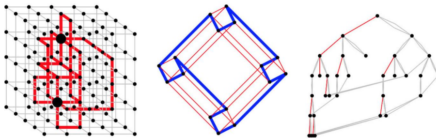
Figure 7.6: Representative Combinatorica graphs: edge-disjoint paths (left), Hamiltonian cycle in a hypercube (center), animated depth-first search traversal (right).
