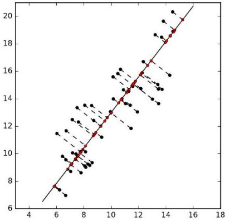
Figure 8.16: PCA projects the black points onto orthogonal axis, rotated to yield the alternate representation in red (left). The values of each component are given by projecting each point onto the appropriate axis (right). positions now define the first dimension (or principal component) of our new representation, as shown in Figure 8.16
