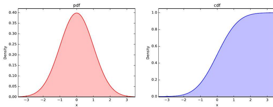
Figure 5.3: The probability density function (pdf) of the normal distribution (left) with its corresponding cumulative density function (cdf) on right. in the lightbulb case: if we only turn on the bulb n = 1000 times, the most likely
