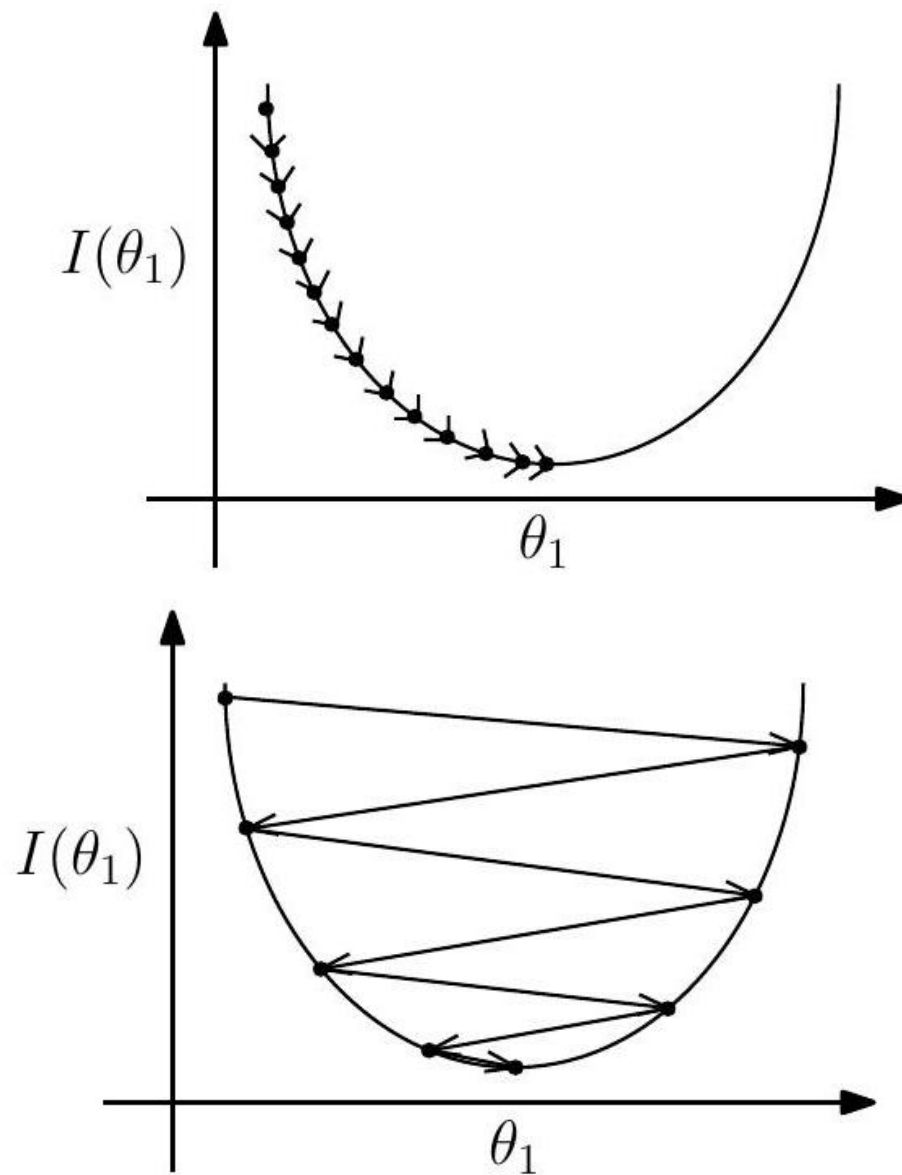
Figure 9.10: The effect of learning rate/step size. Taking too small a step size requires many iterations to converge, while too large a step size causes us to overshoot the minima.
