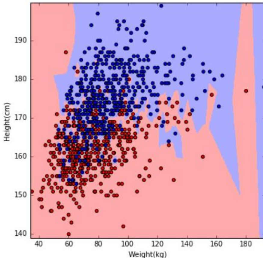
Figure 10.3: The decision boundary of nearest-neighbor classifiers can be
