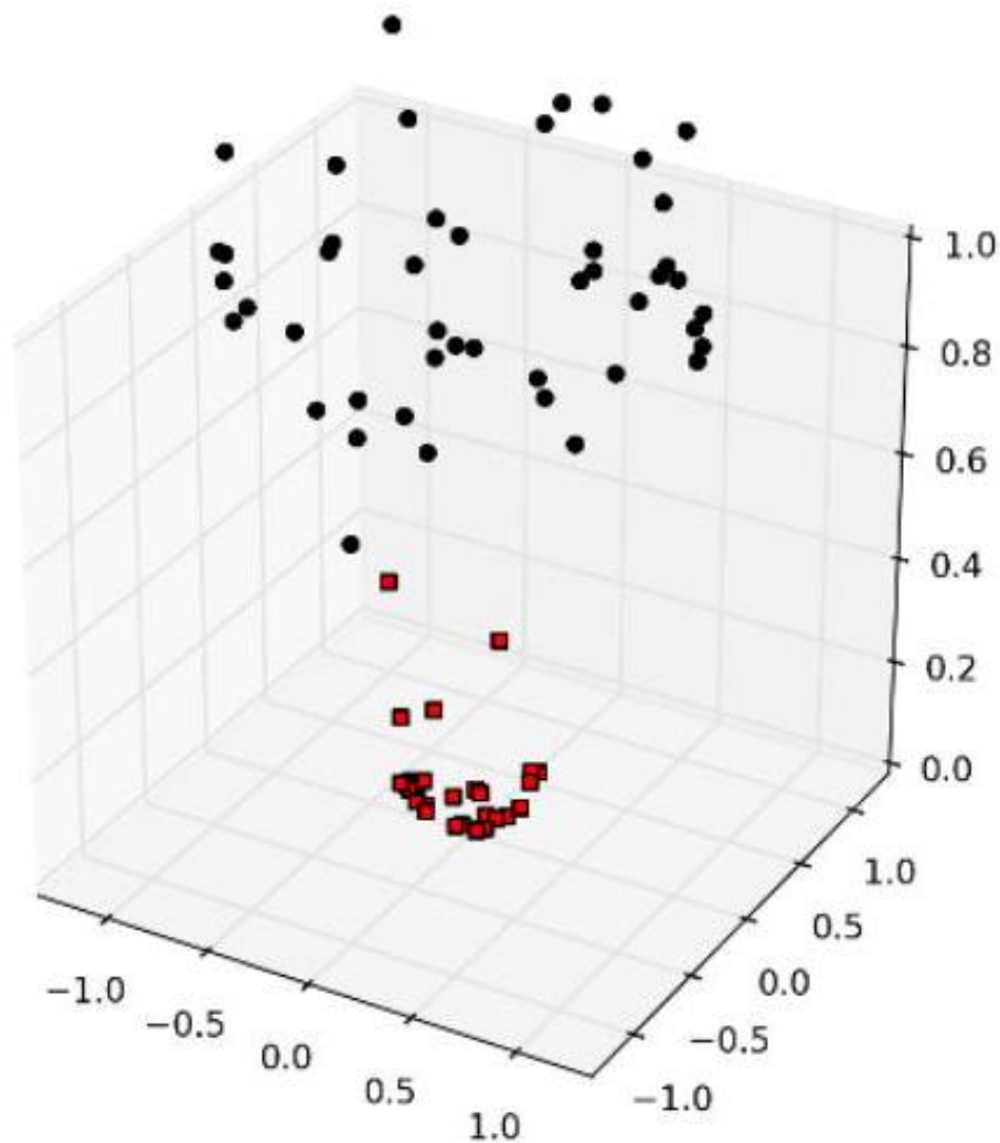
Figure 11.10: Projecting points to higher dimensions can make them linearly separable.
