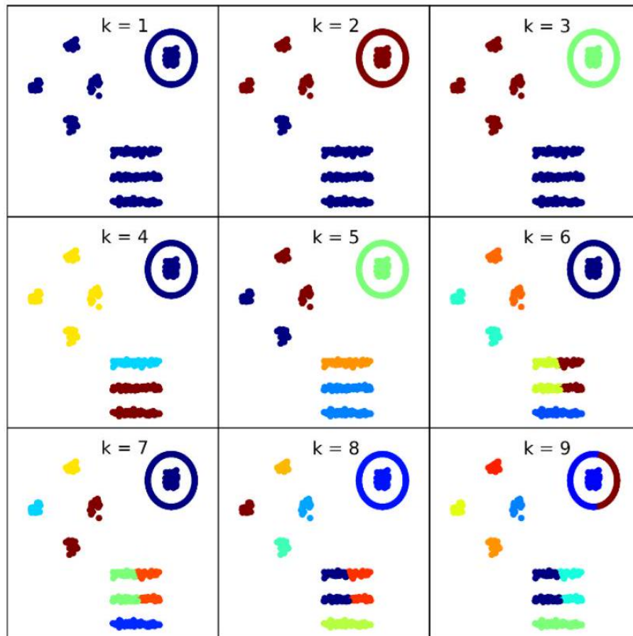
Figure 10.15: Running k -means for k = 1 to k = 9 . The "right" clustering is found for k = 3 , but the algorithm is unable to properly distinguish between nested circular clusters and long thin clusters for large k .
