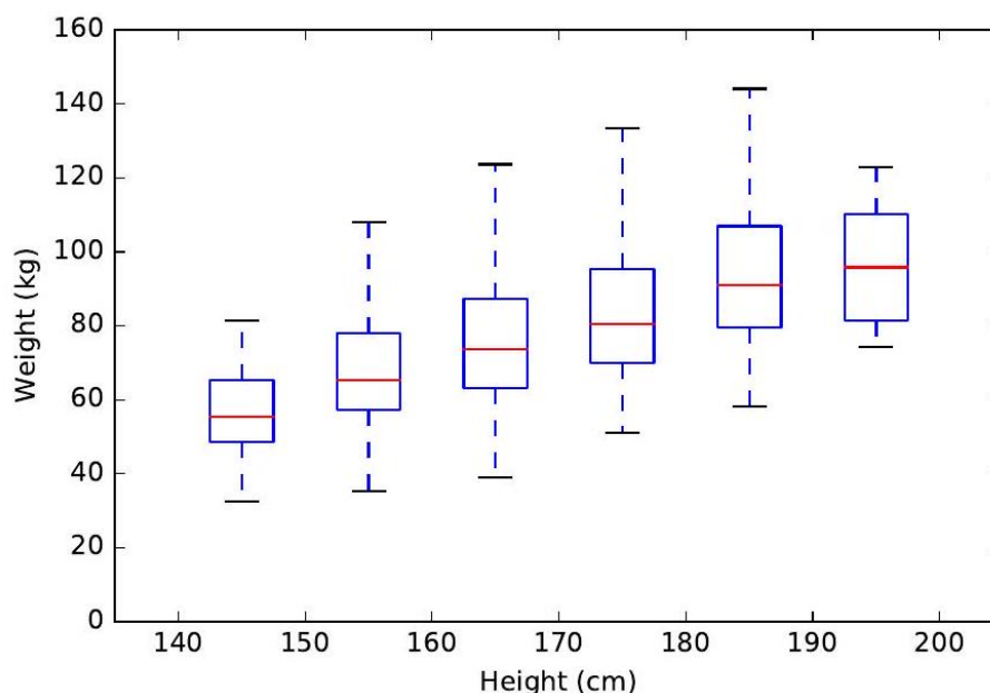
Figure 6.13: Box and whisker plots concisely show the range/quartiles (i.e. median and variance) of a distribution. (hairs) are added to show the range of the highest and lowest values. Figure 6.13 shows a box-and-whisker plot of weight as a function of height in a population sample. The median weight increases with height, but not the maximum, because fewer points in the tallest bucket reduces the chance for an outlier maximum value.
