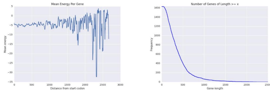
Figure 6.32: Folding energy of genes as a function of their length. Mistaking variance for signal: the extreme values in the left figure are artifacts from averaging small numbers of samples. we just discover that energy varies inversely with gene length?
