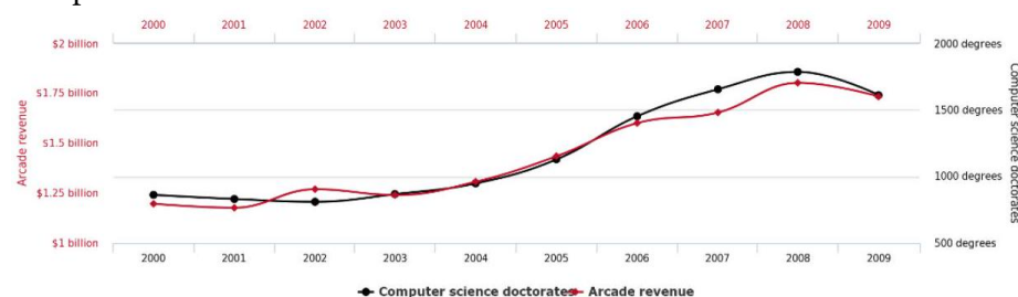
Figure 5.10: Correlation vs. causation: the number of Computer Science Ph.Ds awarded each year in the United States strongly correlates with video/pinball arcade revenue. (from [?])
