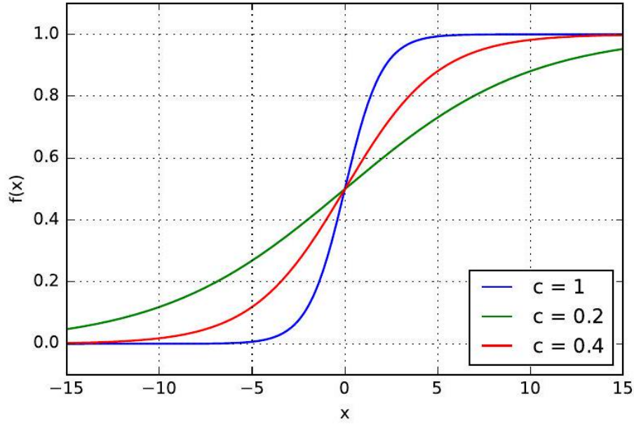
Figure 4.5: The shape of the logit function, for three different values for c . All is clear here except how to determine \mu_A . Given an estimate of the probability that A beats B ( P_{A>B} ), then
