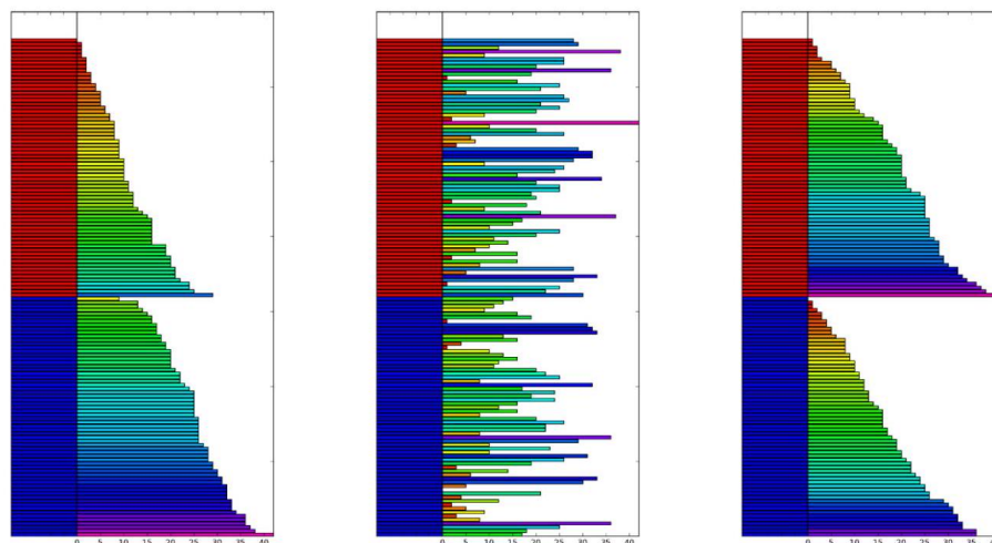
Figure 5.15: Permutation tests reveal the significance of the correlation between gender and the height (left). A random assignment of gender to height (center) results in a substantially different distribution of outcomes when sorted (right), validating the significance of the original relationship.
