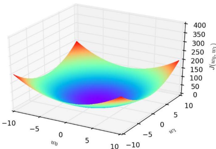
Figure 9.7: Linear regression defines a convex parameter space, where each
