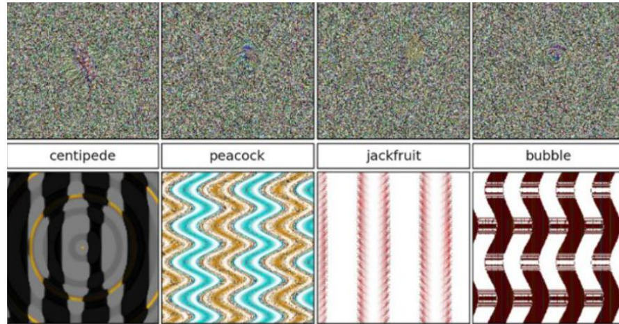
Figure 7.1: Synthetic images that are mistakenly recognized as objects by state-of-the-art Deep Learning neural networks, each with a confidence greater than 99.6%. Source: [?].
