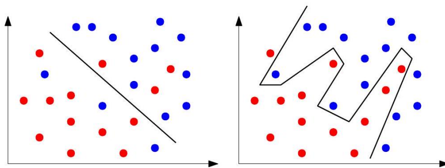
Figure 9.14: Linear classifiers cannot always separate two classes (left). However, perfect separation achieved using complex boundaries usually reflects overfitting more than insight (right).
