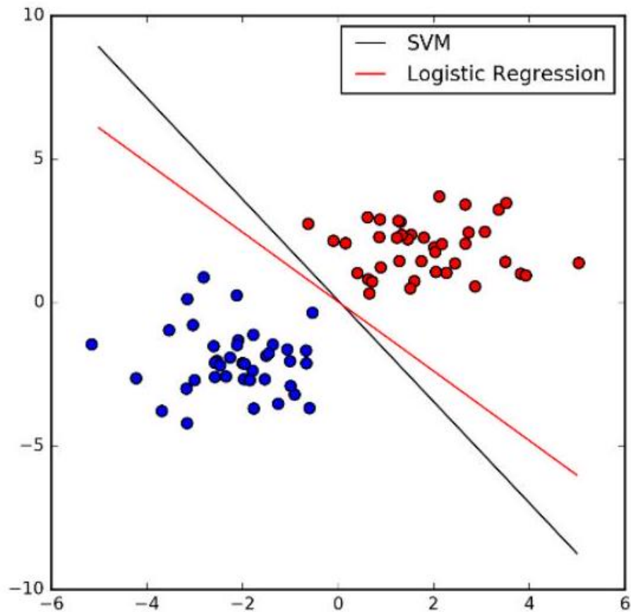
Figure 11.9: Both logistic regression and SVMs produce separating lines between point sets, but optimized for different criteria. best position of the line. These contact points are the support vectors defining the channel.
