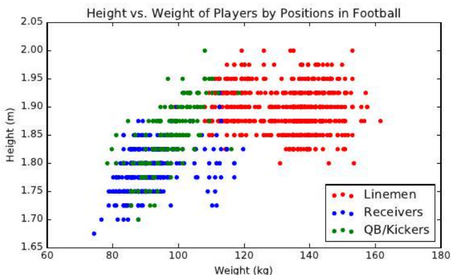
Figure 4.3: Position in basketball (left) and football (right) is largely determined by size.
