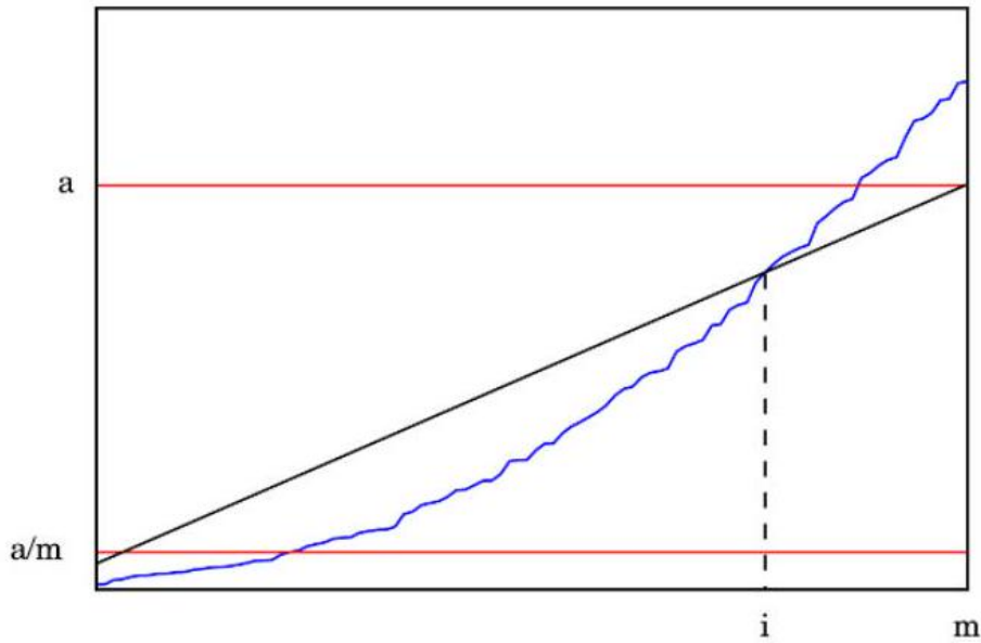
Figure 5.14: The Benjamini-Hochberg procedure minimizes false discovery rate, by accepting p -values only when p_i \leq \alpha i / m . The blue curve shows the sorted p values, and the diagonal defines the cutoff for when such a p -value is significant.
