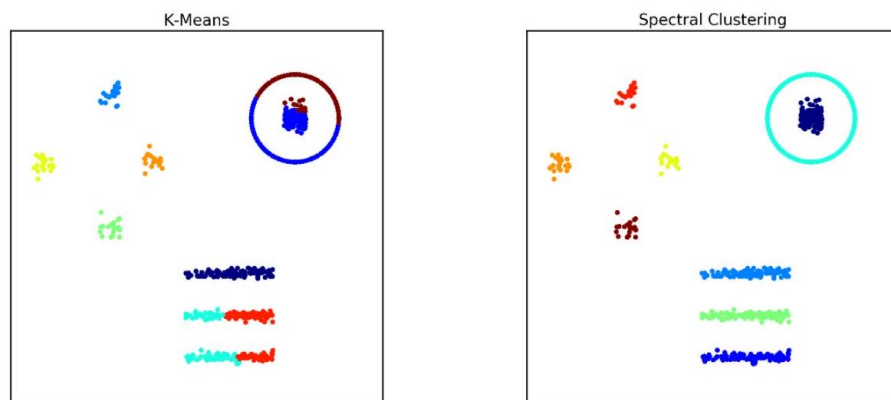
Figure 10.21: The results of k -means (left) and cut-based spectral clustering (right) on our 9 -cluster example. Spectral clustering correctly finds connected
