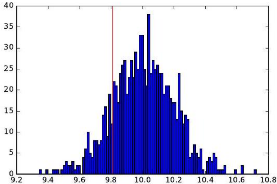
Figure 5.16: Permutation tests score significance by the position of the score on actual data against a distribution of scores produced by random permutations. A position on the extreme tail (left) is highly significant, but one within the body of the distribution (left) is uninteresting. randomly shuffled data sets should be less likely to support it. By conducting many trials against randomized data, we can establish exactly how unusual the phenomenon is that you are testing for.
