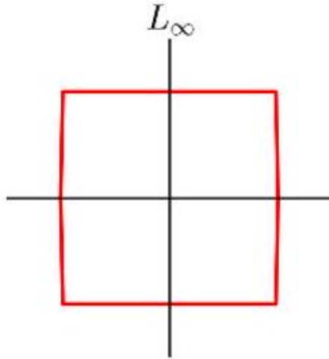
Figure 10.2: The shape of circles defining equal distances changes with k . Consider the distance of points p_1 = (2, 0) and p_2 = (2, 1.99) from the origin:
