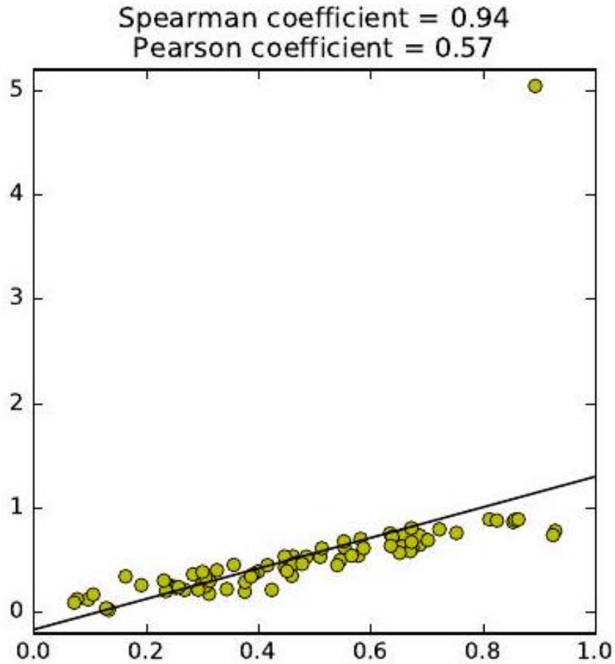
Figure 2.7: A monotonic but not linear point set has a Spearman coefficient r = 1 even though it has no good linear fit (left). Highly-correlated sequences are recognized by both coefficients (center), but the Pearson coefficient is much more sensitive to outliers (right).
