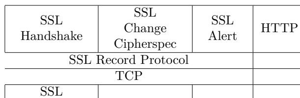
Figure 5.14: Fig. 8.14 SSL architecture
