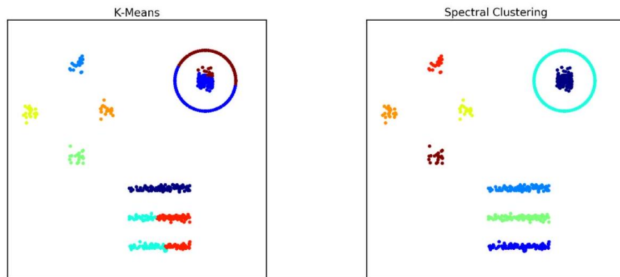
Figure 10.21: The results of k -means (left) and cut-based spectral clustering (right) on our 9-cluster example. Spectral clustering correctly finds connected clusters here that k -means cannot. We seek clusters that are connected in an appropriate similarity graph.
