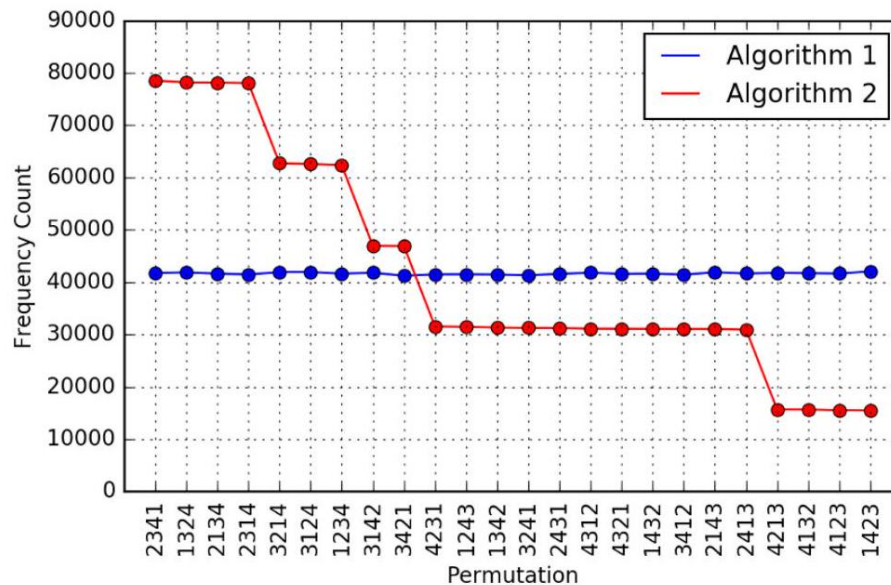
Figure 5.17: The generation frequency of all 4! = 24 permutations using two different algorithms. Algorithm 1 generates them with uniform frequency, while algorithm 2 is substantially biased. recurs on the rest. It generates permutations uniformly at random. The second
