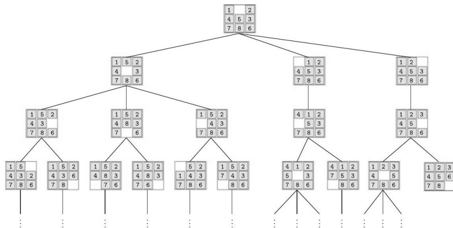
Figure 18: Search tree for an 8-puzzle without cycles of length 2
