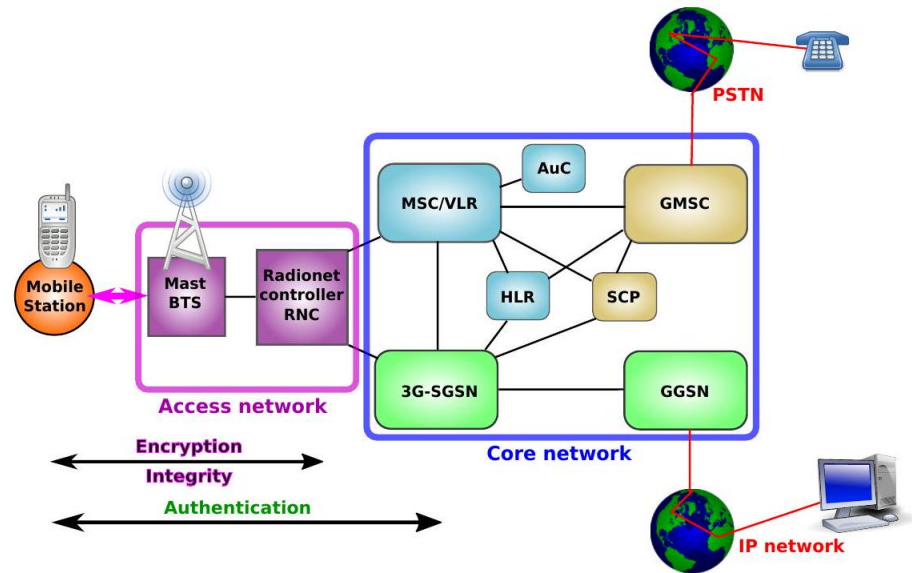
Figure 7.27: The architecture of a telephone network based on UMTS
