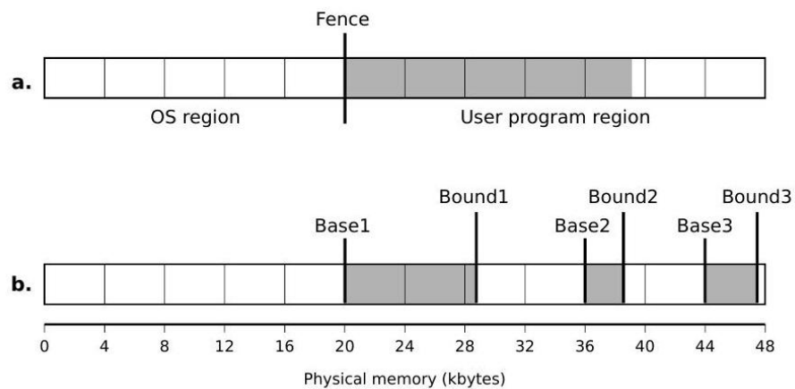
Figure 7.48: Fig. 9.17 Two simple techniques for memory protection
