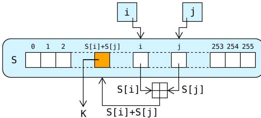
Figure 4.24: The lookup step in RC4's keystream generator. (Diagram: Wikimedia Commons ©)
