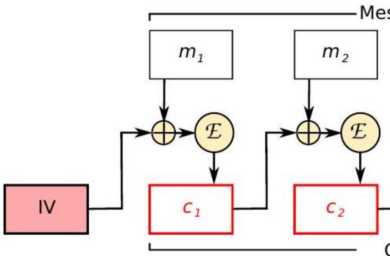
Figure 4.20: Operation of DES in CBC mode
