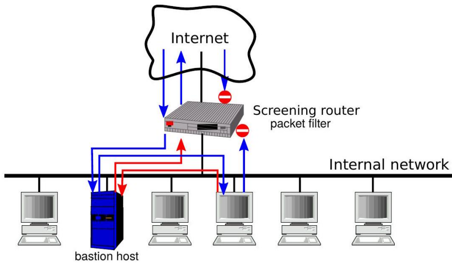
Figure 7.22: A screened host setup
