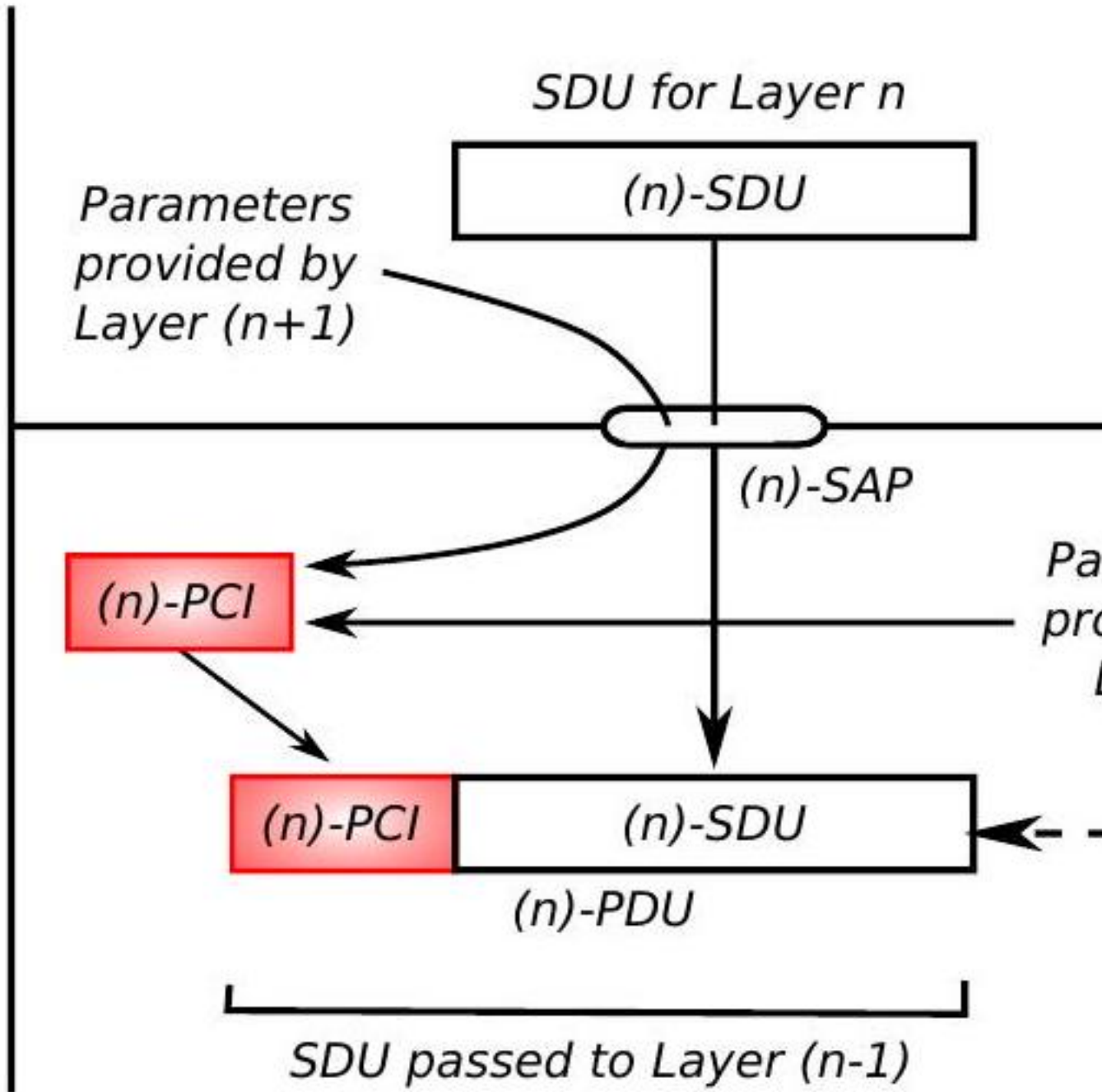
Figure 6.3: Adding PCI to a PDU.
