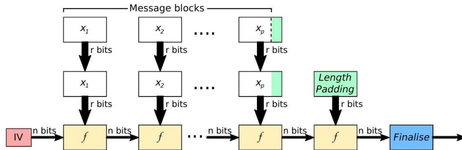
Figure 5.2: Principle of operation of a cryptographic hash function based on the Merkle-Damgaard construction
