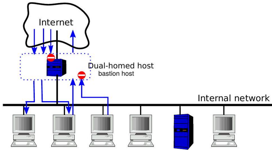
Figure 7.21: A dual-homed host setup
