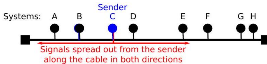
Figure 6.14: Communication in Ethernet
