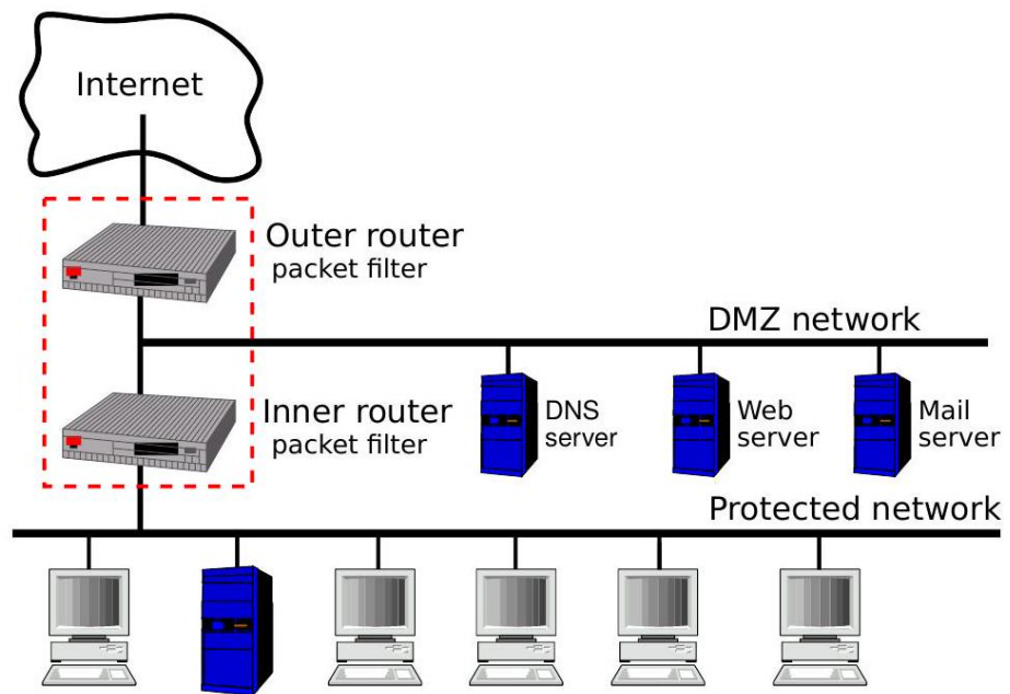
Figure 7.23: A screened subnet setup with DMZ
