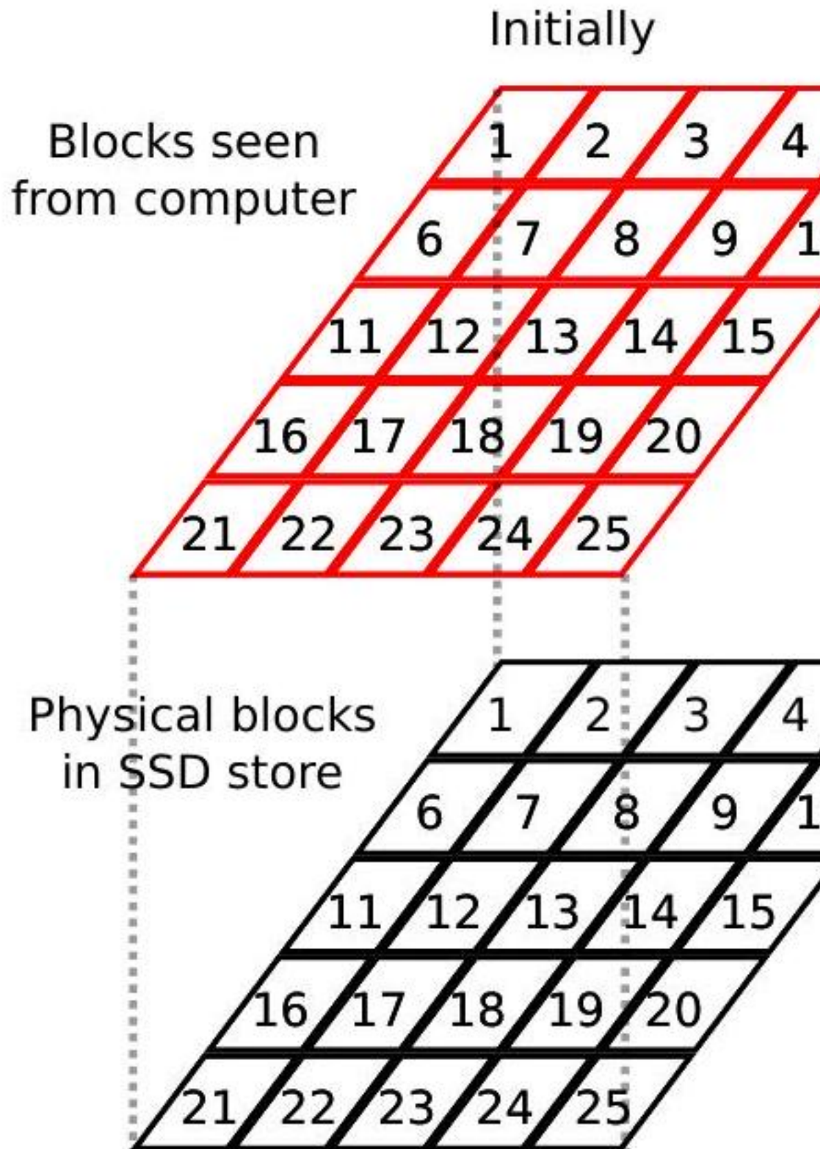
Figure 8.14: Wear levelling in an SSD
