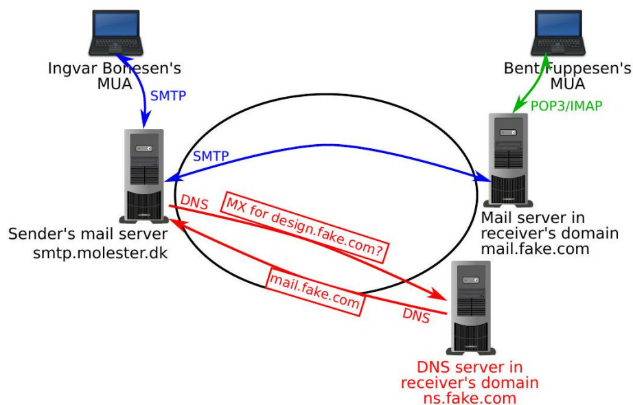
Figure 7.2: Mail relaying in the Internet
