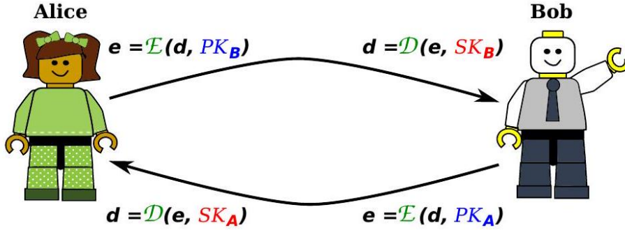
Figure 4.25: Encryption and decryption in a PKCS
