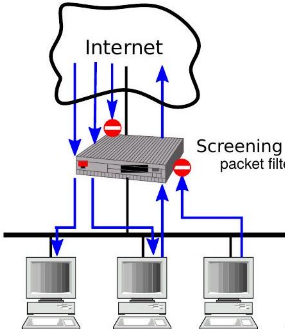
Figure 7.20: Fig. 8.20 A screening router setup
