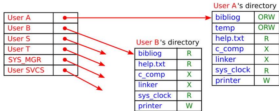
Figure 7.44: Fig. 9.13 Directories
