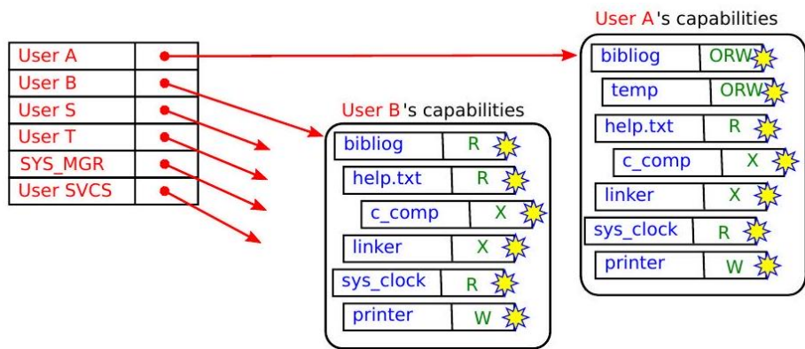
Figure 7.45: Fig. 9.14 Capabilities
