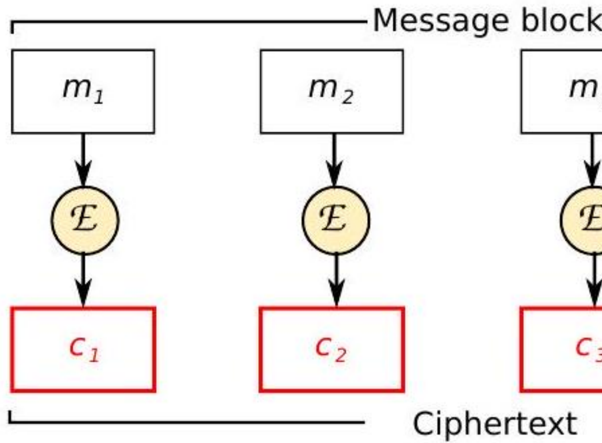
Figure 4.19: Operation of DES in ECB mode
