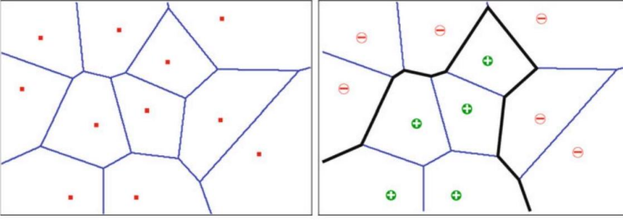
Figure 57: A set of points together with their Voronoi-Diagram (left) and the dividing line generated for the two classes M_+ and M_- (right).
