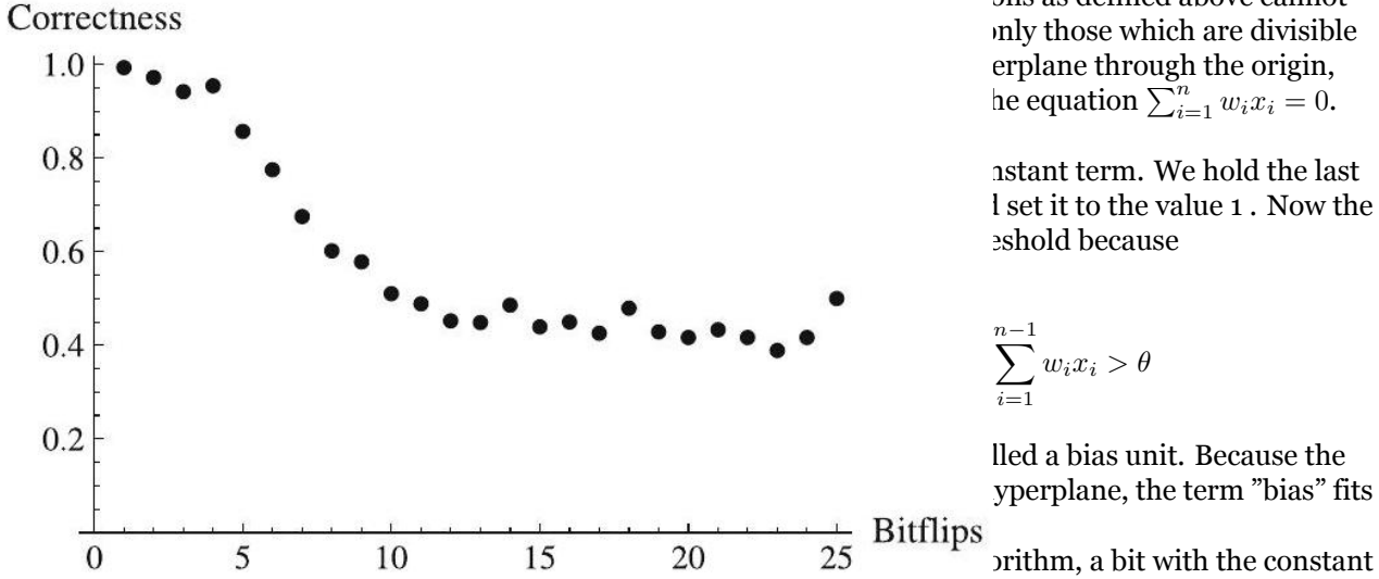
Figure 55: Relative correctness of the perceptron threshold function learned during the learning process. of inverted bits in the test data
