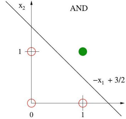
Figure 51: The boolean function AND (true, 0 \hat{=} false)
