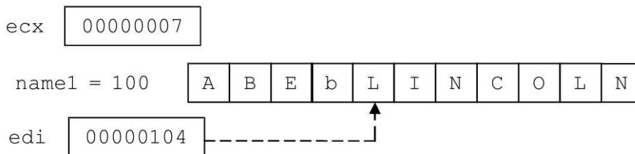
Figure 30: Using repne scasb
