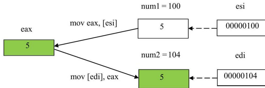
Figure 25: Using esi and edi to move data from memory to memory
