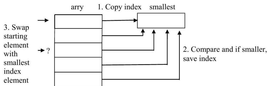
Figure 28: Simplified selection sort
