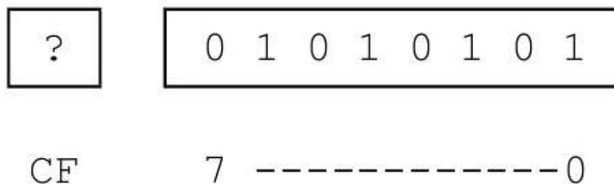
Figure 12: Initial contents of al register
