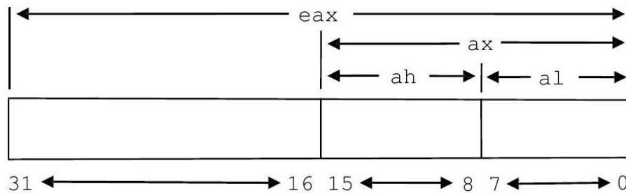
Figure 3: Format of the eax , ax , ah , and al registers
