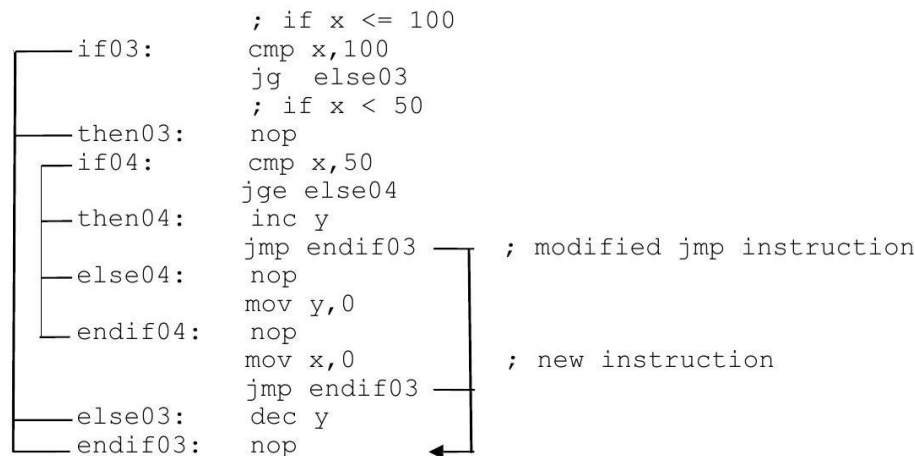
Figure 11: If-then-if structure with inadvisable jump
