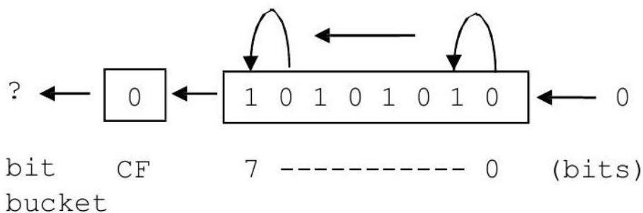
Figure 13: Results in al register after shl instruction
