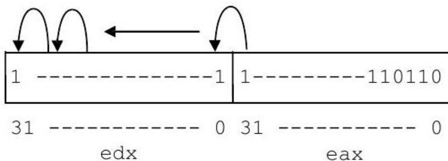
Figure 6: eax registers after execution of the imul instruction
