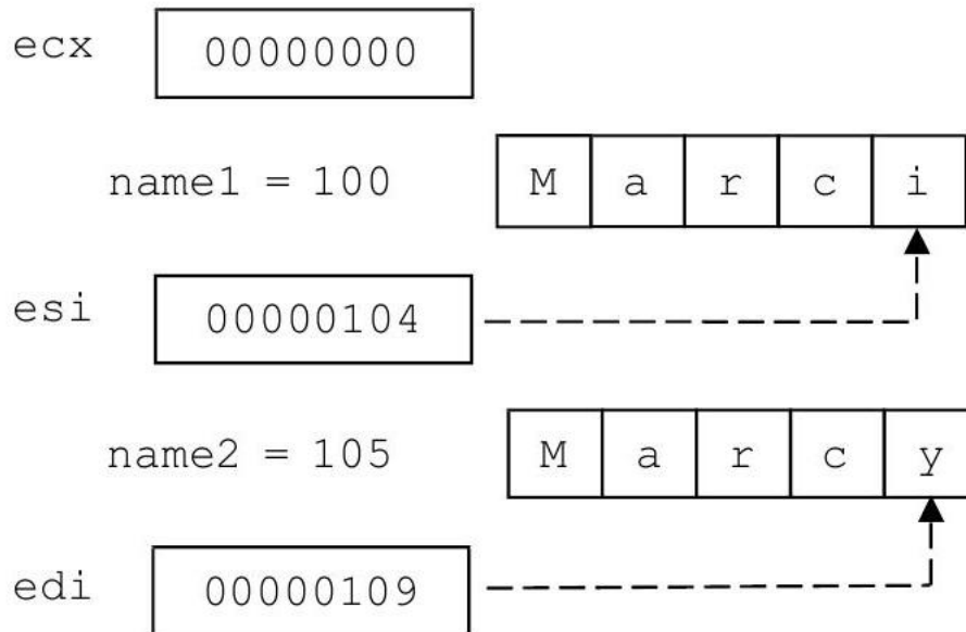
Figure 34: Using repe cmpsb and backing up one character
