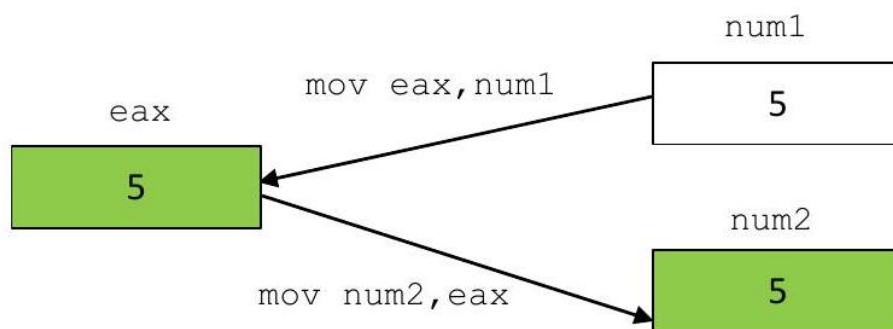
Figure 4: Mov instruction
