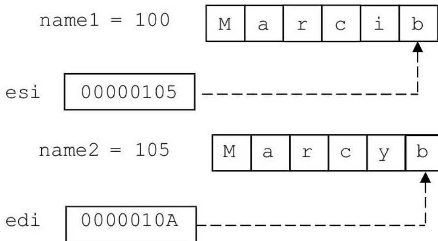
Figure 33: Using repe cmpsb with extra blanks □
