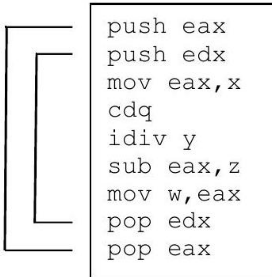
Figure 19: Saving and restoring multiple registers
