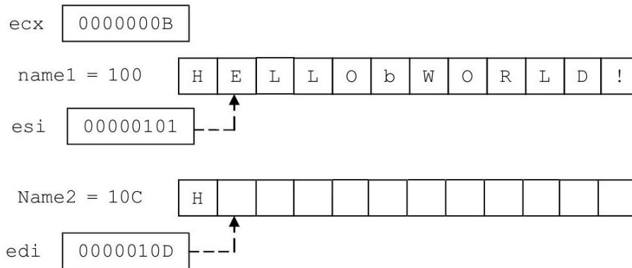
Figure 29: Using esi and edi to move a string
