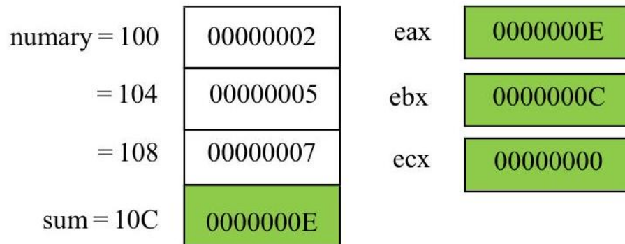
Figure 22: Using ebx for array processing
