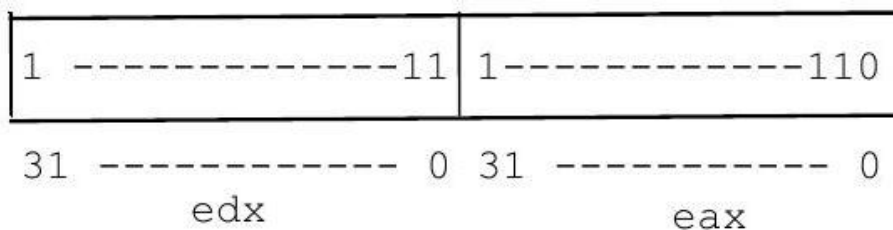
Figure 7: Propagating the sign bit from eax through edx
