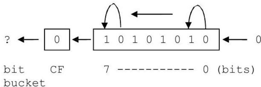
Figure 15: Results in al register after sal instruction
