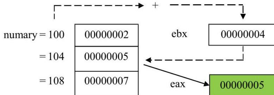
Figure 23: Using ebx register to access a single element
