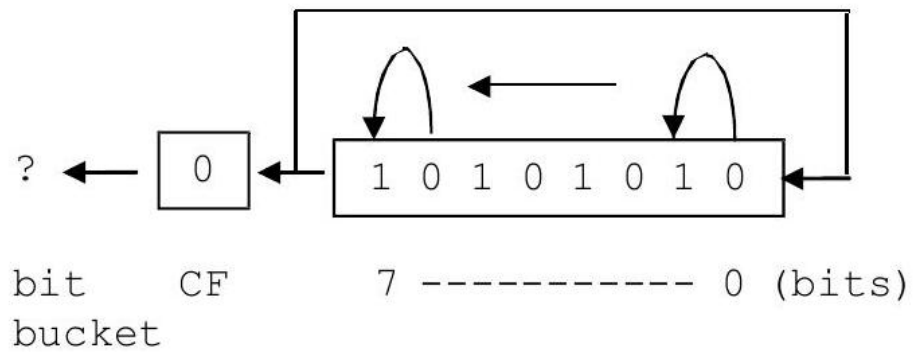
Figure 17: Initial contents of al Register
