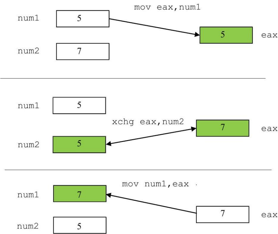
Figure 20: Swapping using the xchg instruction
