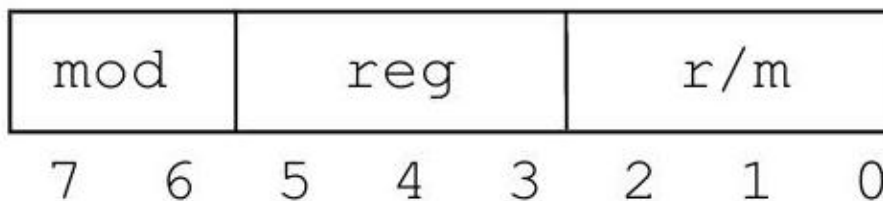
Figure 39: Format of mod reg r/m
