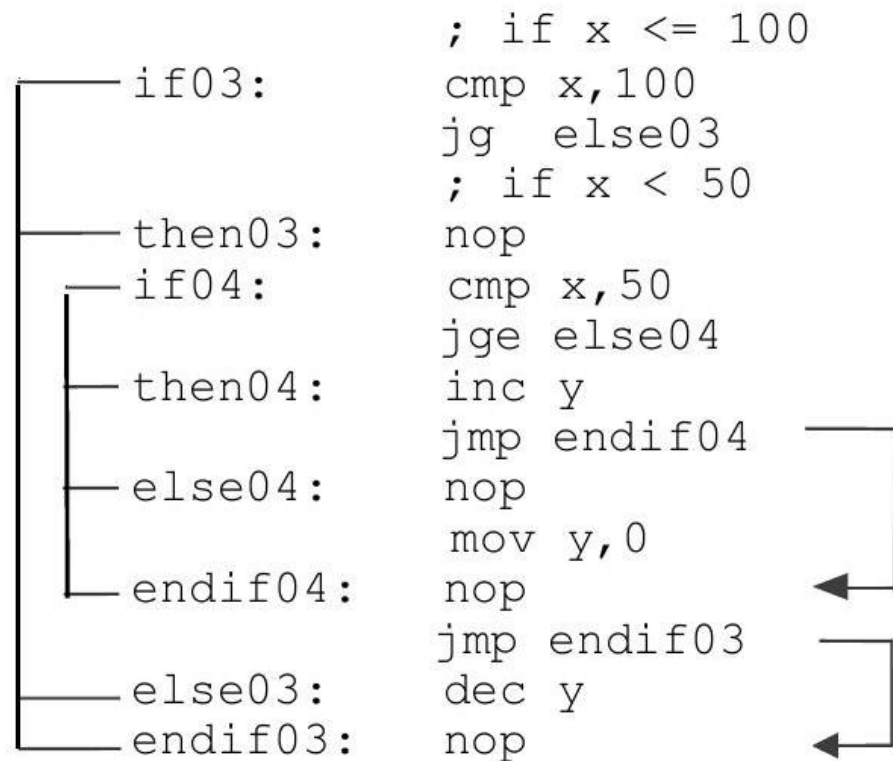
Figure 10: If-then-if structure
