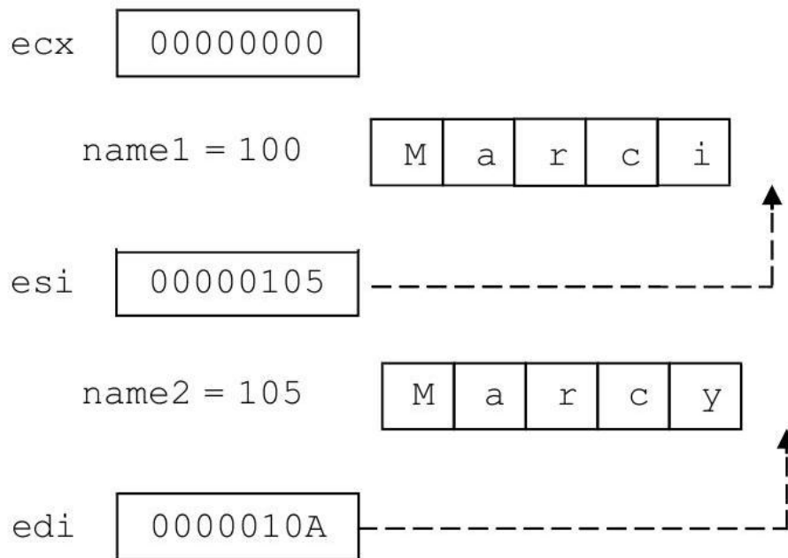
Figure 32: Using repe cmpsb with difference in last character
