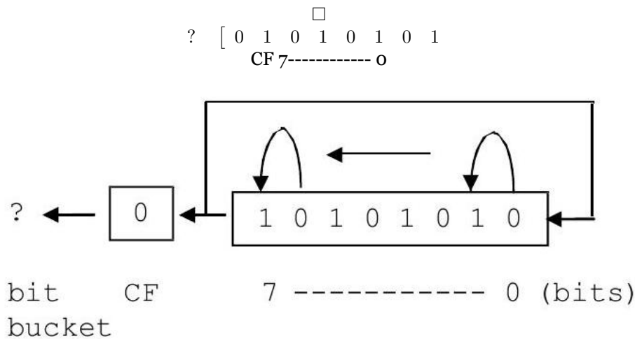
Figure 17: Initial contents of al Register
