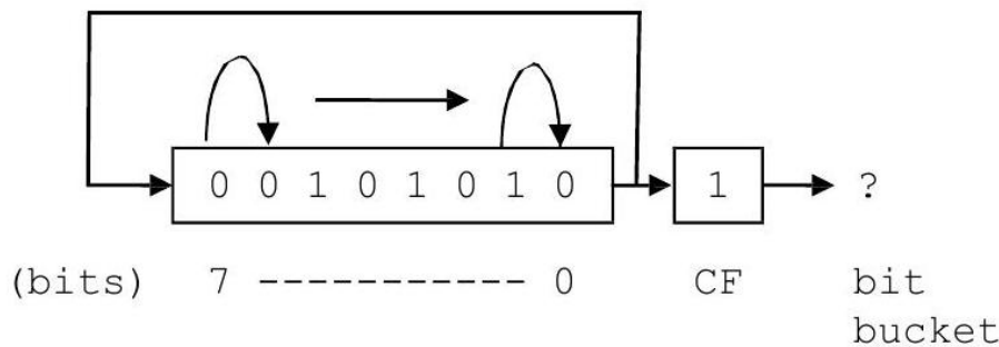
Figure 18: Results in al register after rol instruction
