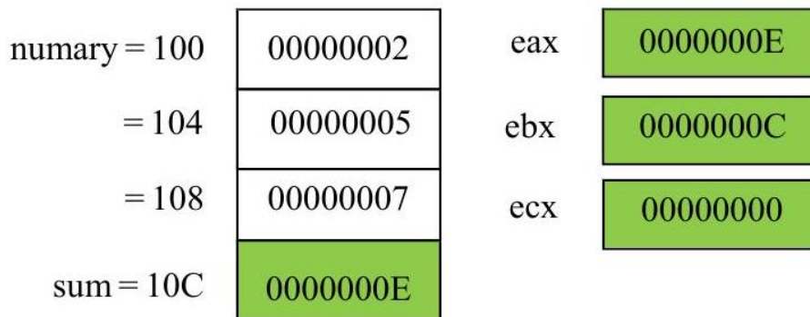
Figure 22: Using ebx for array processing
