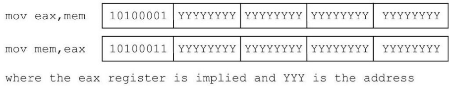
Figure 38: Format for the mov eax, mem and mov mem, eax instructions
