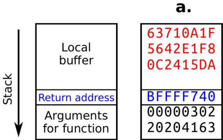
Fig. 120: Buffer Overflow
