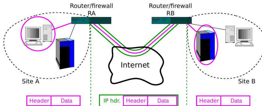
Fig. 76: Site-to-site tunneling
