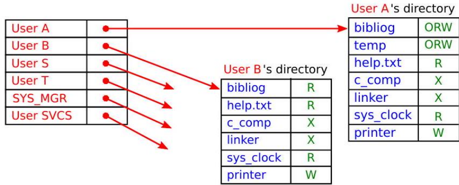
Fig. 109: Directories
