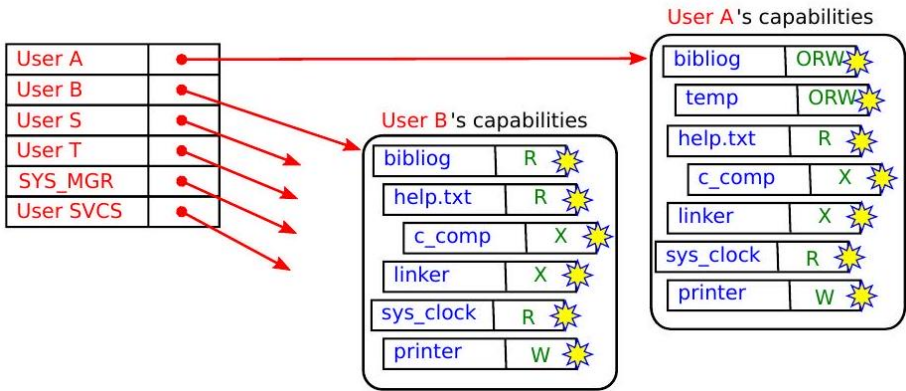
Fig. 110: Capabilities
