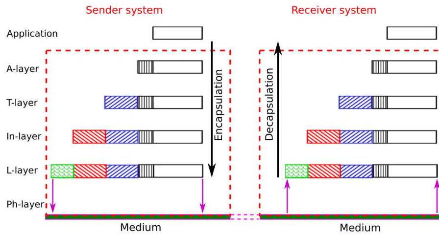
Fig. 51: Encapsulation and decapsulation in the Internet
