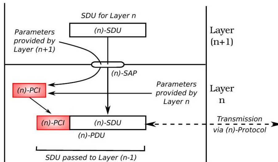
Fig. 48: Adding PCI to a PDU.
