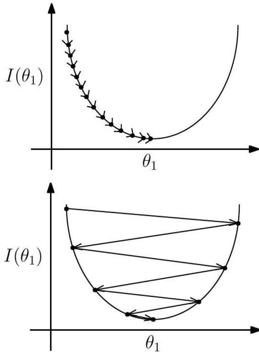
Figure 112: The effect of learning rate/step size. Taking too small a step size requires many iterations to converge, while too large a step size causes us to overshoot the minima.
