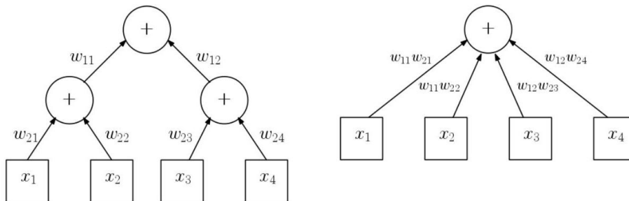
Figure 150: Addition networks do not benefit from depth. The two layer network (left) computes exactly the function as the equivalent one layer network (right).
