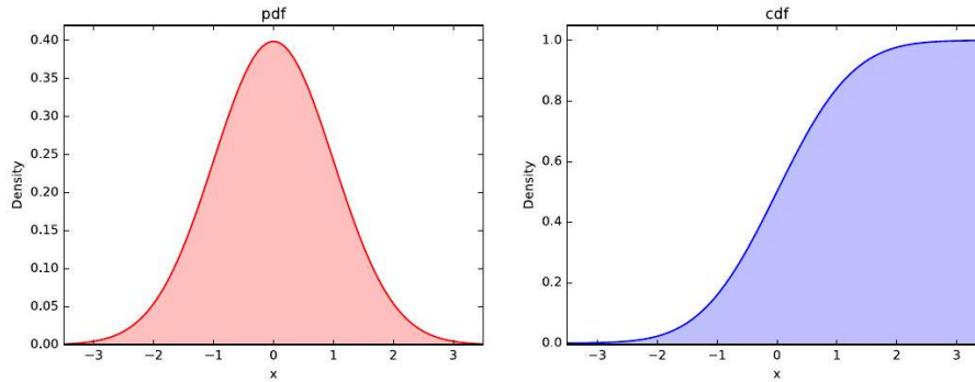
Figure 34: The probability density function (pdf) of the normal distribution (left) with its corresponding cumulative density function (cdf) on right.
