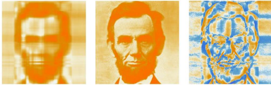
Figure 102: Lincoln's face reconstructed from 5 (left) and 50 (center) singular values, with the error for k = 50 (right).
