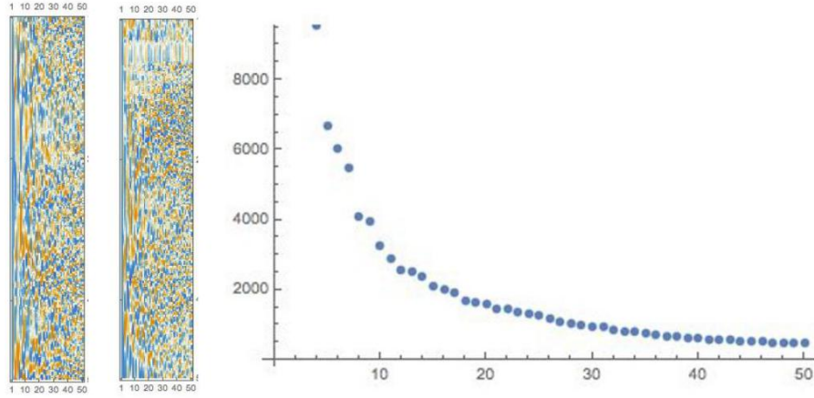
Figure 101: Singular value matrices in the decomposition of Lincoln, for 50 singular values.
