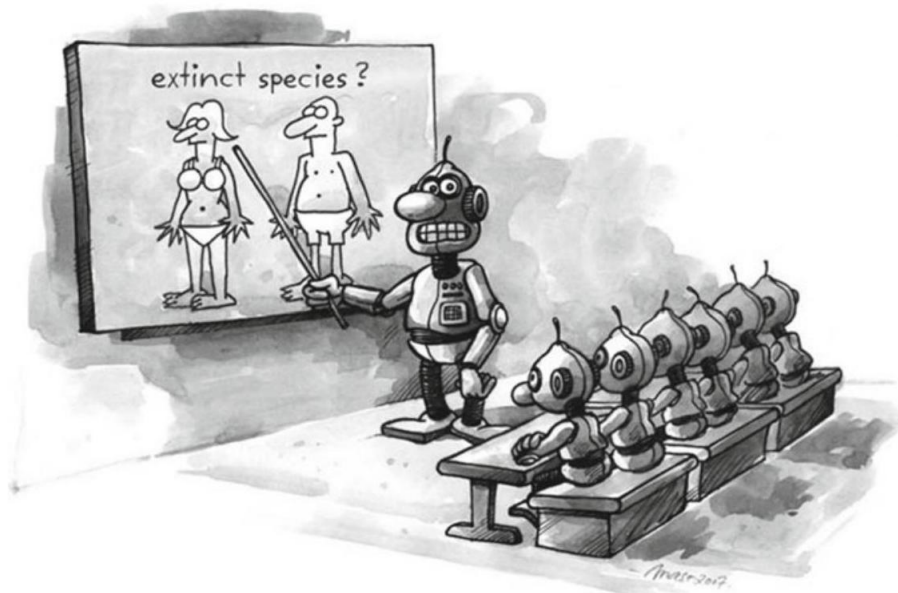
Figure 44: Supervised learning ...
