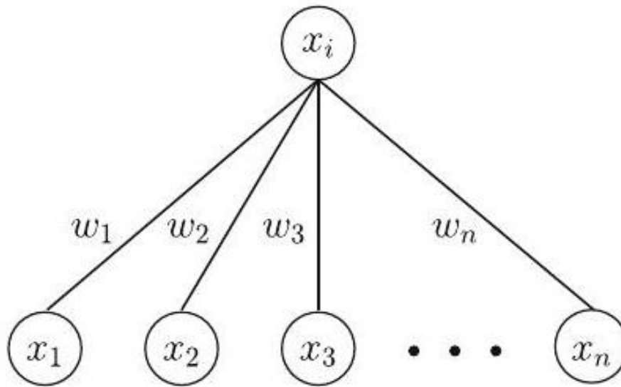
Figure 82: The structure of a formal neuron, which applies the activation function f to the weighted sum of all inputs
