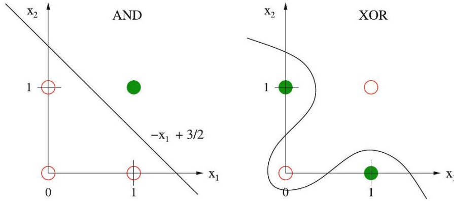
Figure 51: The boolean function AND is linearly separable, but XOR is not ( 0 \hat{=} true, 0 \hat{=} false)
