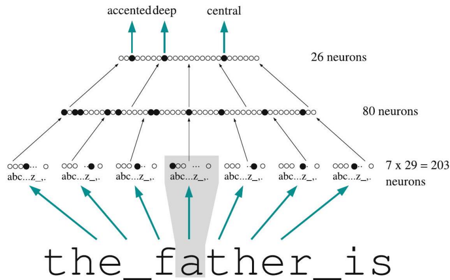
Figure 95: The NETtalk network maps a text to its pronunciation attributes
