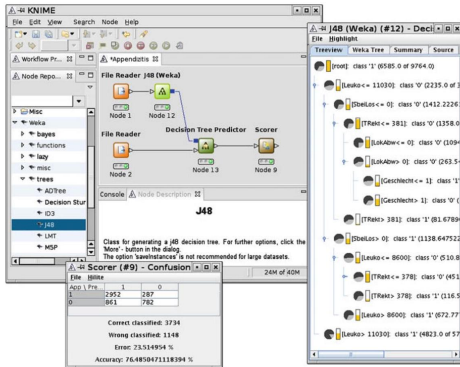
Figure 79: The KNIME user interface with two additional views, which show the decision tree and the confusion matrix
