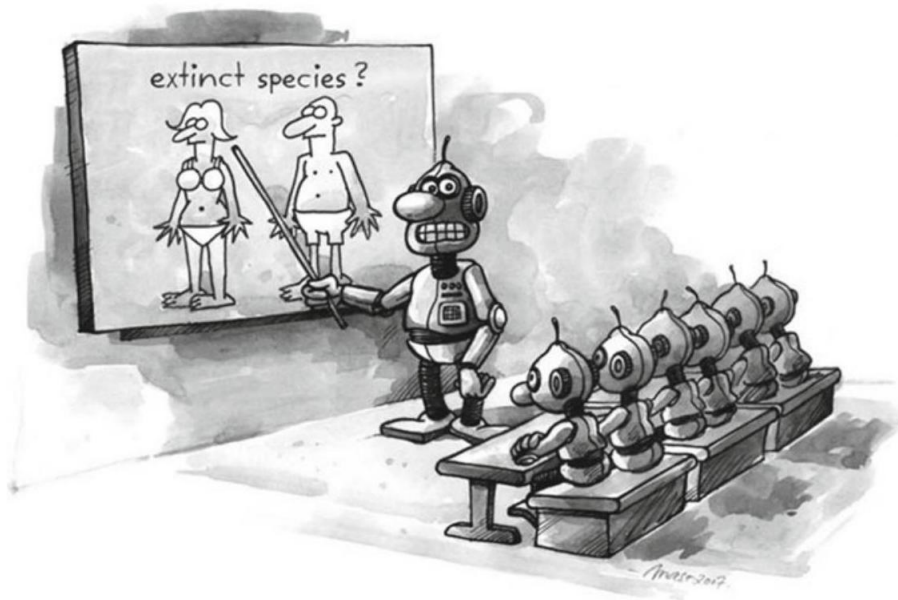
Figure 44: Supervised learning ...
