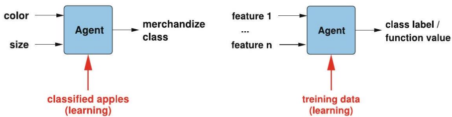
Figure 47: Functional structure of a learning agent for apple sorting (left) and in general (right)
