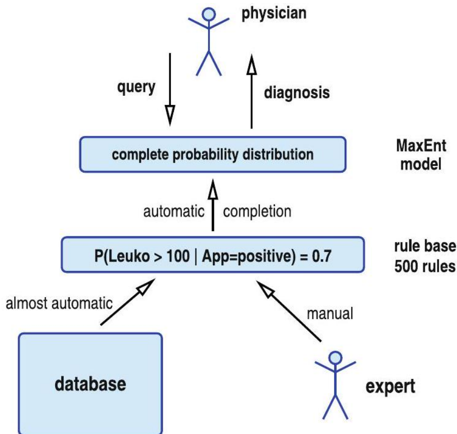
Figure 35: Probabilistic rules are generated from data and expert knowledge, which are integrated in a rule base (knowledge base) and finally made complete using the MaxEnt method
