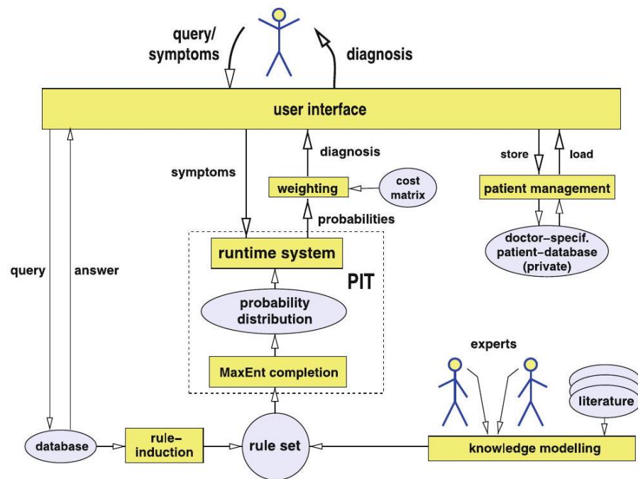
Figure 36: Rules are generated from the database as well as from expert knowledge. From these, MaxEnt creates a complete probability distribution. For a user query, the probability of every possible diagnosis is calculated. Using the cost matrix (see Sect. 7.3.5) a decision is then suggested
