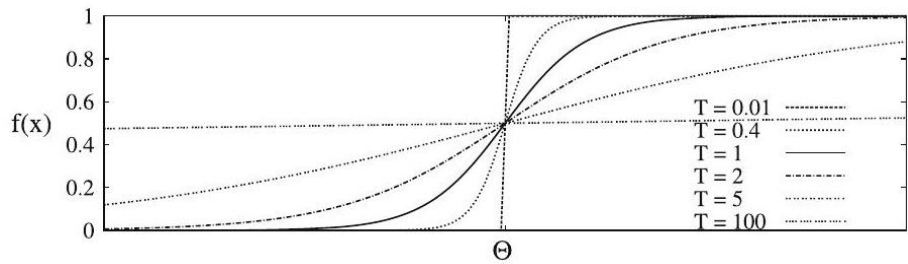
Figure 83: The neuron with a step function works like a perceptron with a threshold
