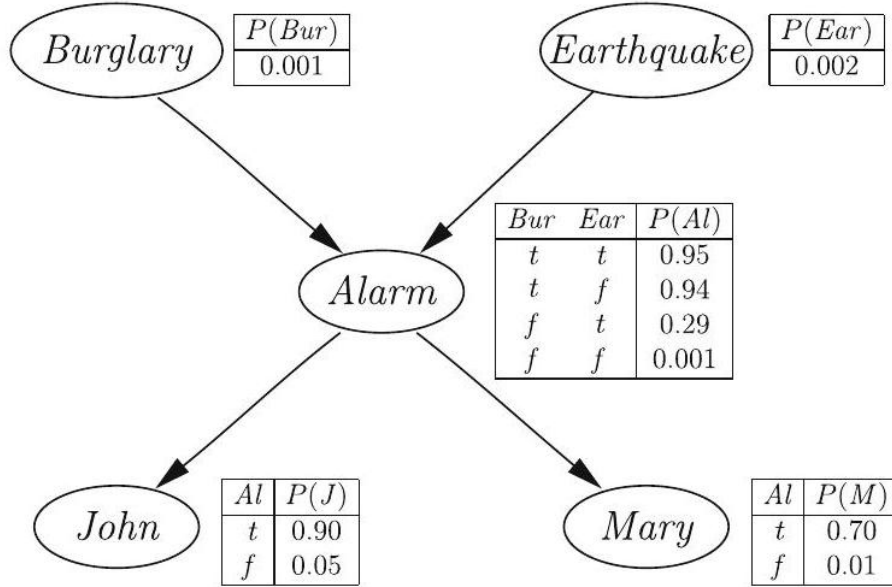
Figure 39: Bayesian network for the alarm example with the associated CPTs
