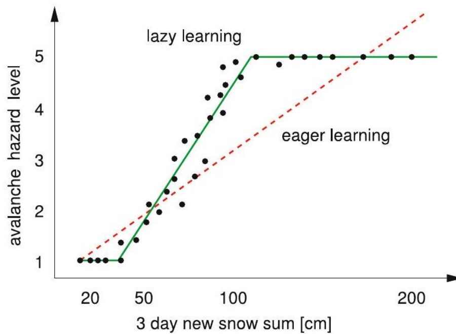
Figure 62: To determine avalanche hazard, a function is approximated from training data. Here for comparison are a local model (solid line), and a global model (dashed line)
