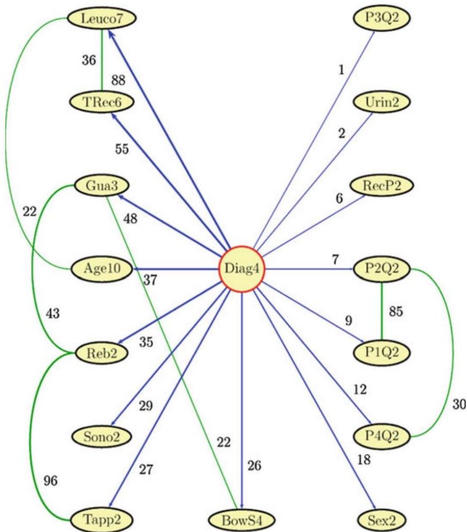
Figure 37: Dependency graph computed from the database
