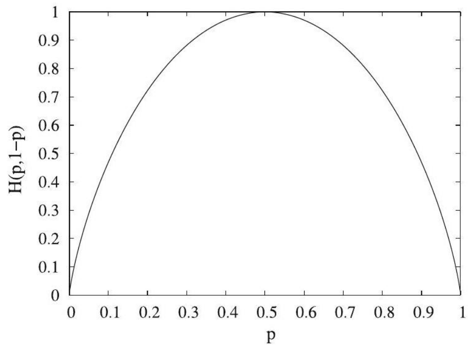
Figure 65: The entropy function for the case of two classes. We see the maximum at p = 1/2 and the symmetry with respect to swapping p and 1 - p
