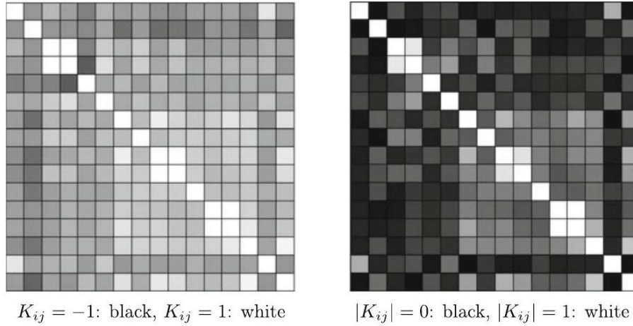
Figure 49: The correlation matrix as a frequency graph. In the left diagram, dark stands for negative and light for positive. In the right image the absolute values were listed. Here black means K_{ij} \approx 0 (uncorrelated) and white |K_{ij}| \approx 1 (strongly correlated)
