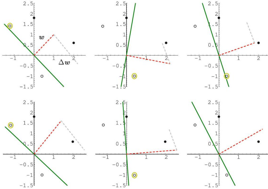
Figure 53: Application of the perceptron learning rule to two positive ( \cdot ) and two negative ( \circ ) data points. The solid line shows the current dividing line w\mathbf{x} = 0 . The orthogonal dashed line is the weight vector w and the second dashed line the change vector \Delta w = \mathbf{x} or \Delta w = -\mathbf{x} to be added, which is calculated from the currently active data point surrounded in light green
