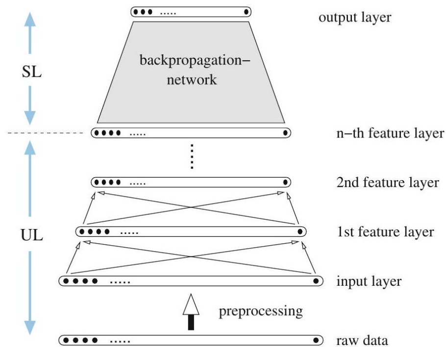
Figure 100: Simplified architecture of a deep learning network. It is composed of a preprocessor, several layers (in this case two) for unsupervised feature detection and then one classical neural network, which, in this example, is trained by backpropagation
