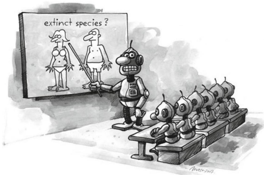
Figure 44: Supervised learning ...
