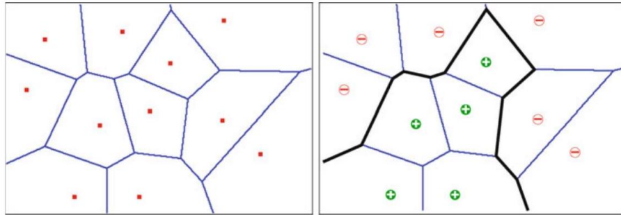
Figure 57: A set of points together with their Voronoi-Diagram (left) and the dividing line generated for the two classes M_+ and M_-
