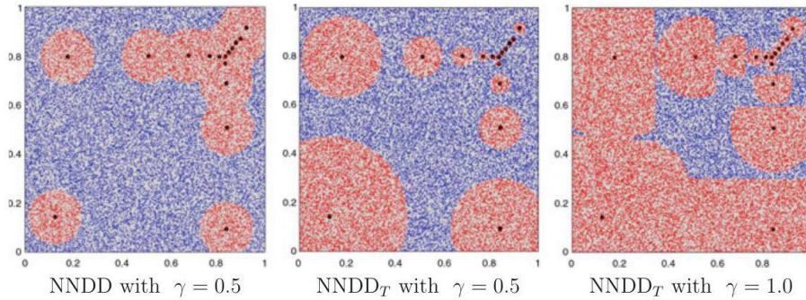
Figure 72: \text{NNDD}_{\text{and}} \text{NNDD}_T applied to a set of 16 selected two-dimensional data points (black points). In each case, class membership has been determined for 10,000 randomly selected points. The points marked in red were classified as positive, i.e. assigned the training set's class, while the blue points are classified as negative
