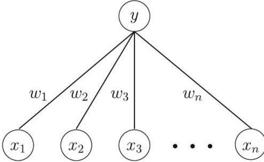
Figure 90: A two-layer network with an output neuron
