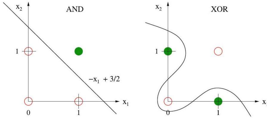
Figure 51: The boolean function AND is linearly separable, but XOR is not ( 0 \triangleq true, 0 \triangleq false)
