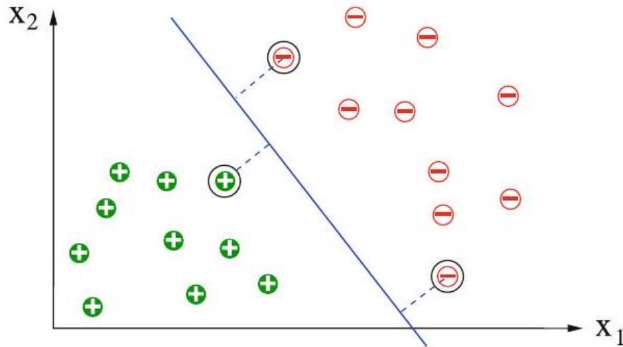
Figure 99: Two classes with the maximally dividing line. The circled points are the support vectors
