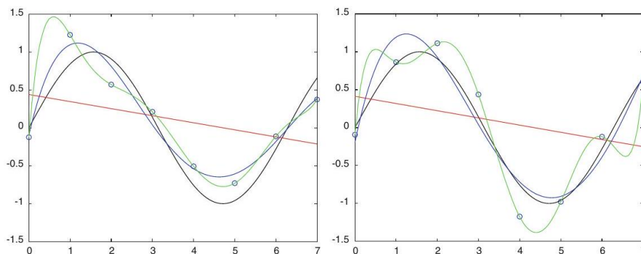
Figure 68: Two different data sets approximated by polynomials of degree 1, 4 and 7. The bias variance tradeoff is clearly visible
