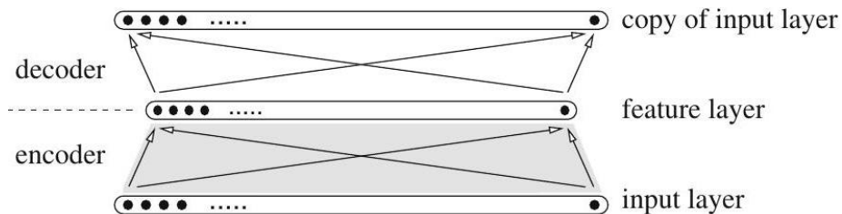
Figure 101: Autoencoder for learning the weights of a feature layer. A classical backpropagation network can be used here to learn the identity mapping from the current input layer onto itself. Features form in the hidden layer during learning
