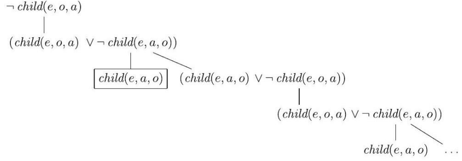
Figure 14: PROLOG search tree for child (eve, oscar, anne)
