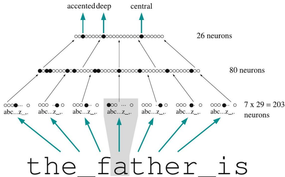
Figure 95: The NETtalk network maps a text to its pronunciation attributes
