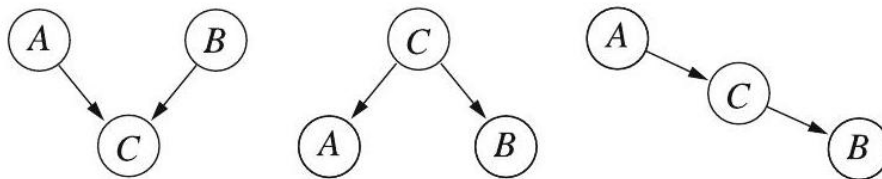
Figure 43: Stepwise construction of the alarm network considering causality conditionally independent (middle, right)
