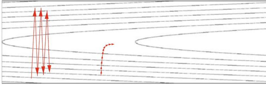
Figure 92: Gradient descent for a large \eta (left) and a very small \eta (right) into a valley descending flatly to the right. For a large \eta there are oscillations around the valley. For a \eta which is too small, in contrast, convergence in the flat valley happens very slowly
