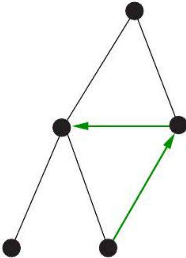
Figure 58: The possible edge cases for graph traversal. Forward edges and cross edges can occur in DFS only on directed graphs.
