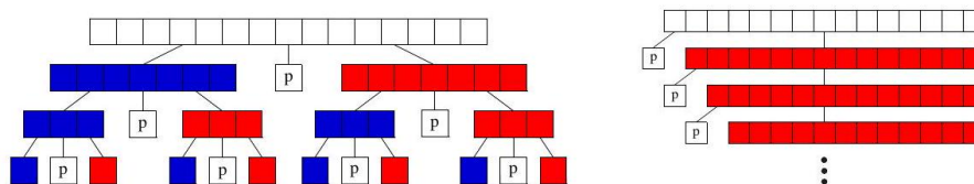
Figure 29: The best-case (left) and worst-case (right) recursion trees for quicksort. The left partition is in blue and the right partition in red.
