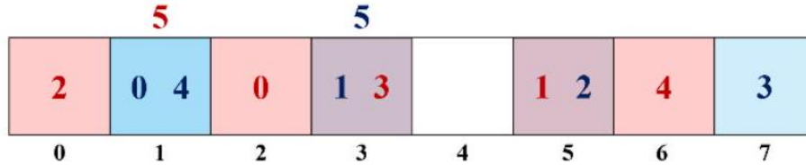
Figure 42: Hashing the integers 0, 1, 2, 3, and 4 into an n = 8 bit Bloom filter, using hash functions h_1(x) = 2x + 1 (blue) and h_2(x) = 3x + 2 (red). Searching for x = 5 would yield a false positive, since the two corresponding bits have been set by other elements.
