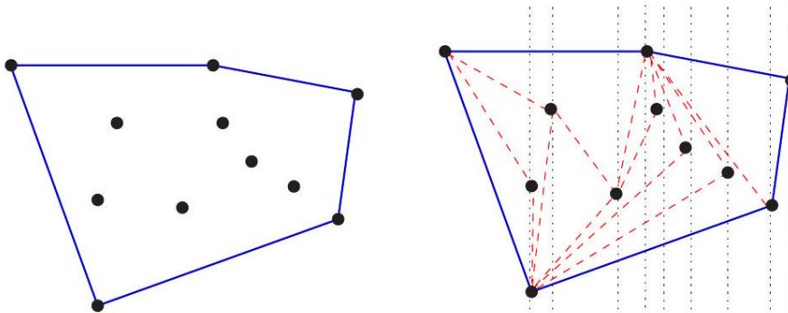
Figure 25: The convex hull of a set of points (left), constructed by left-to-right insertion (right).
