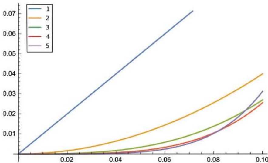
Figure 43: Bloom filter error probability as a function of load (m/n) for k from 1 to 5. By selecting the right k for the given load, we can dramatically reduce false positive error rate with no increase in table space.
