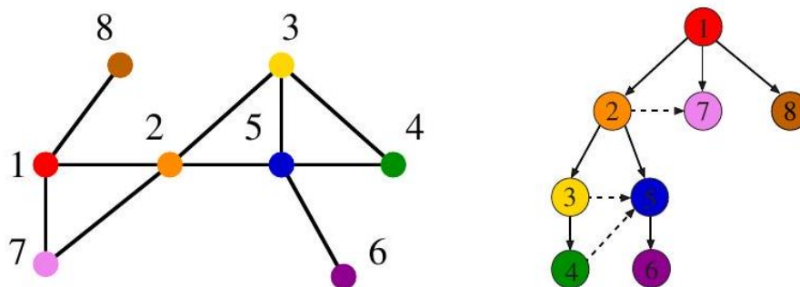
Figure 53: An undirected graph and its breadth-first search tree. Dashed lines, which are not part of the tree, show graph edges that go to discovered or processed vertices.
