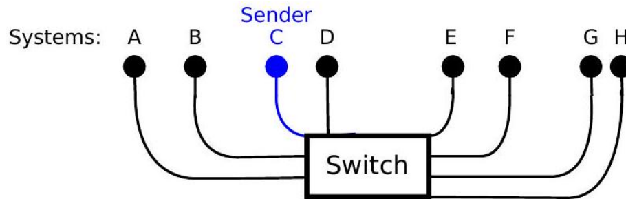
Fig. 60: Communication in Ethernet
