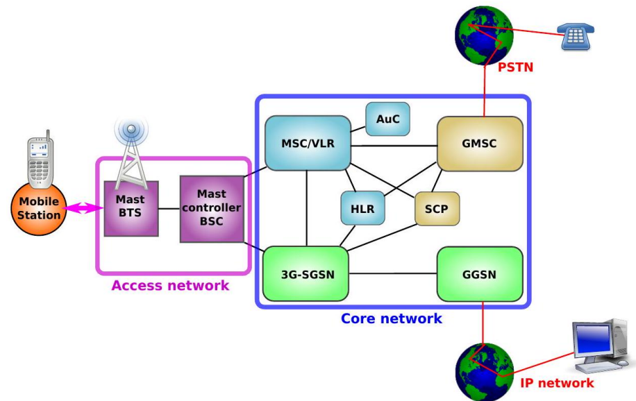
Fig. 63: The architecture of a telephone network based on GSM
