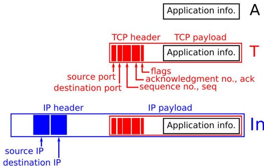
Fig. 54: Encapsulation in TCP and IP
