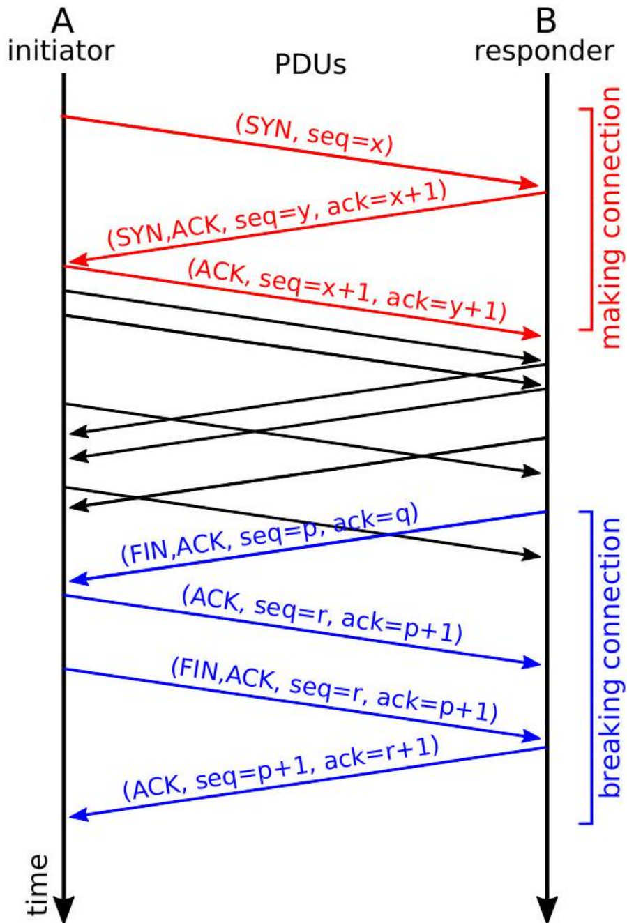
Fig. 55: Exchange of PDUs via a TCP connection
