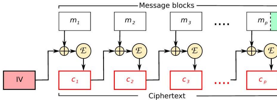
Fig. 31: Operation of DES in CBC mode
