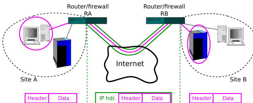
Fig. 76: Site-to-site tunneling
