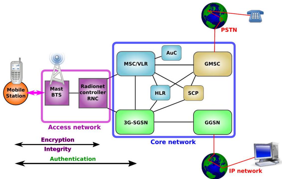
Fig. 91: The architecture of a telephone network based on UMTS
