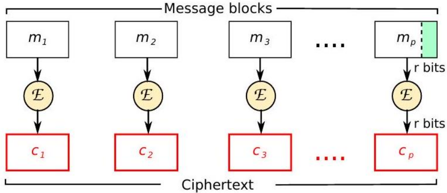
Fig. 30: Operation of DES in ECB mode
