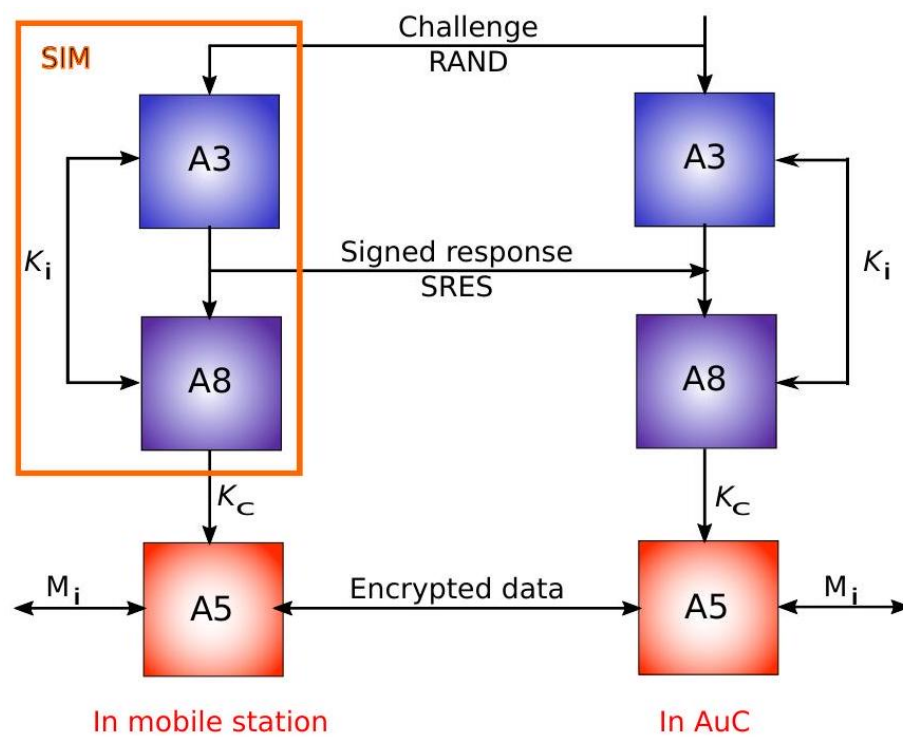
Fig. 90: Cryptographic functions in GSM
