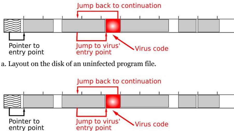
Fig. 124: Placement of virus code in an executable file.
