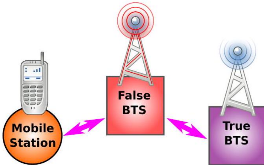
Fig. 92: A false BTS can take over the traffic from a mobile station
