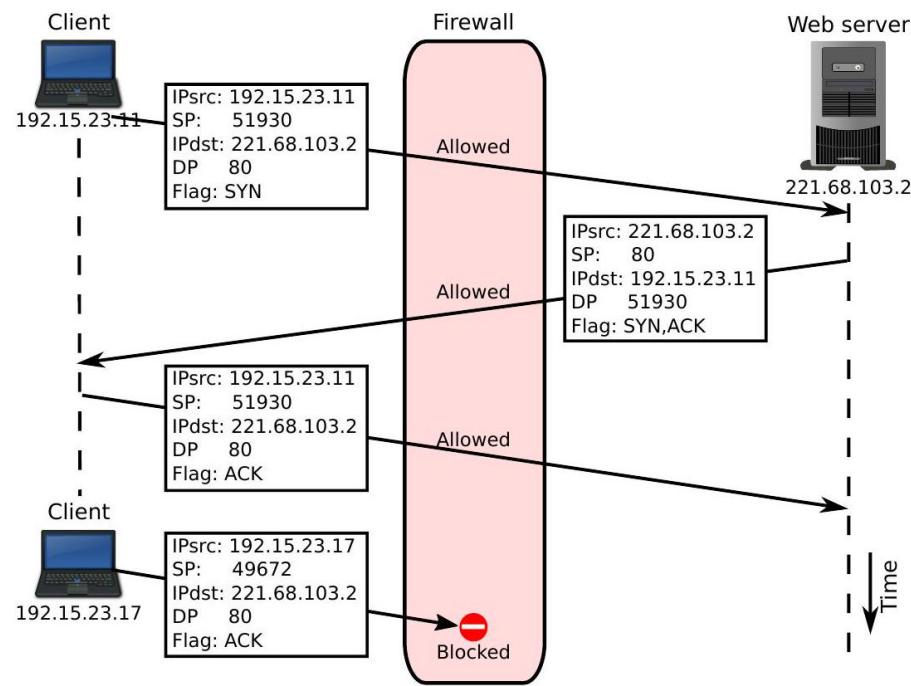
Fig. 82: An SPI firewall
