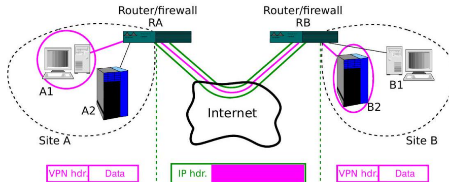
Fig. 77: Secure site-to-site tunneling in a VPN
