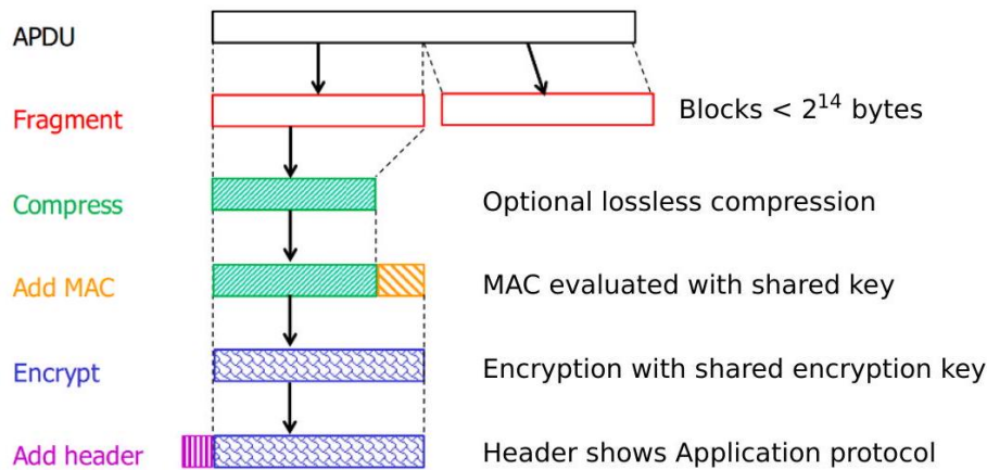
Fig. 80: Treatment of APDUs in SSL/TLS's Record protocol
