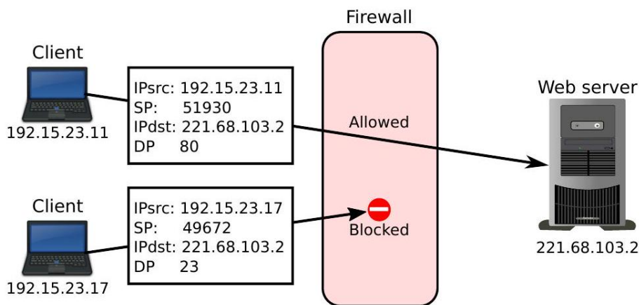
Fig. 81: A PF firewall
