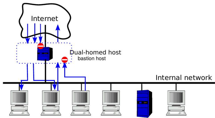
Fig. 85: A dual-homed host setup
