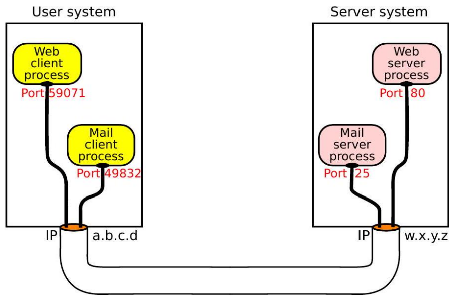
Fig. 53: Ports for use by TCP and UDP
