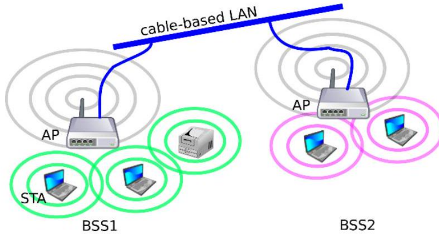
Fig. 61: An ESS with two BSSs
