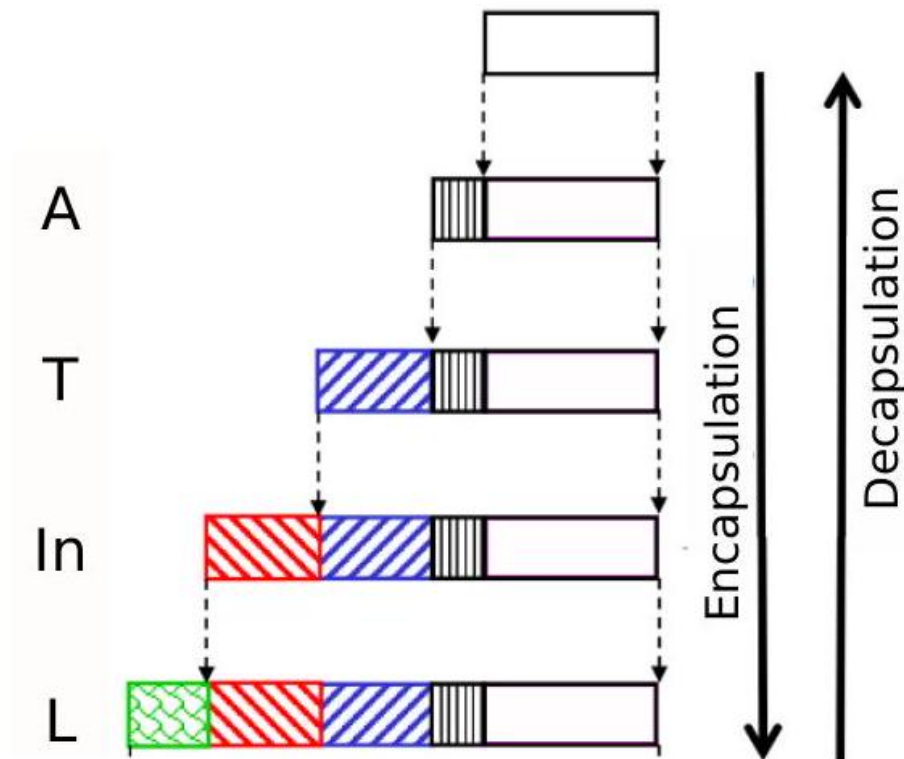
Fig. 69: Embedding of PDUs in a layered architecture
