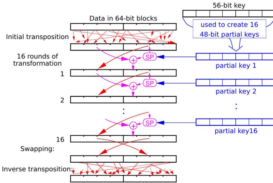
Fig. 29: Operation of the Digital Encryption Standard (DES)
