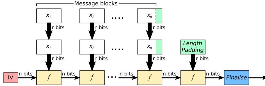
Fig. 37: Principle of operation of a cryptographic hash function based on the Merkle-Damgaard construction
