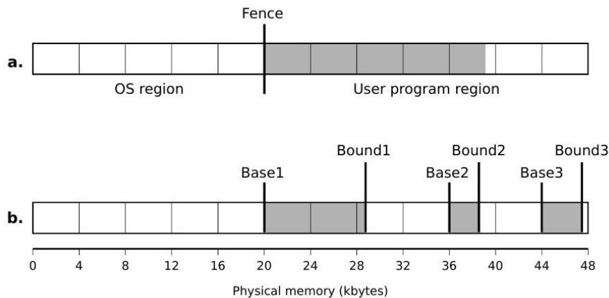
Fig. 113: Two simple techniques for memory protection
