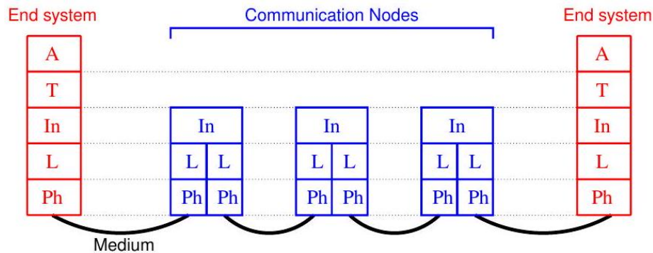
Fig. 56: End systems and communication nodes
