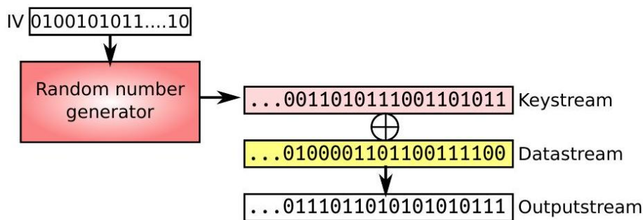
Fig. 33: Operation of a stream cipher.
