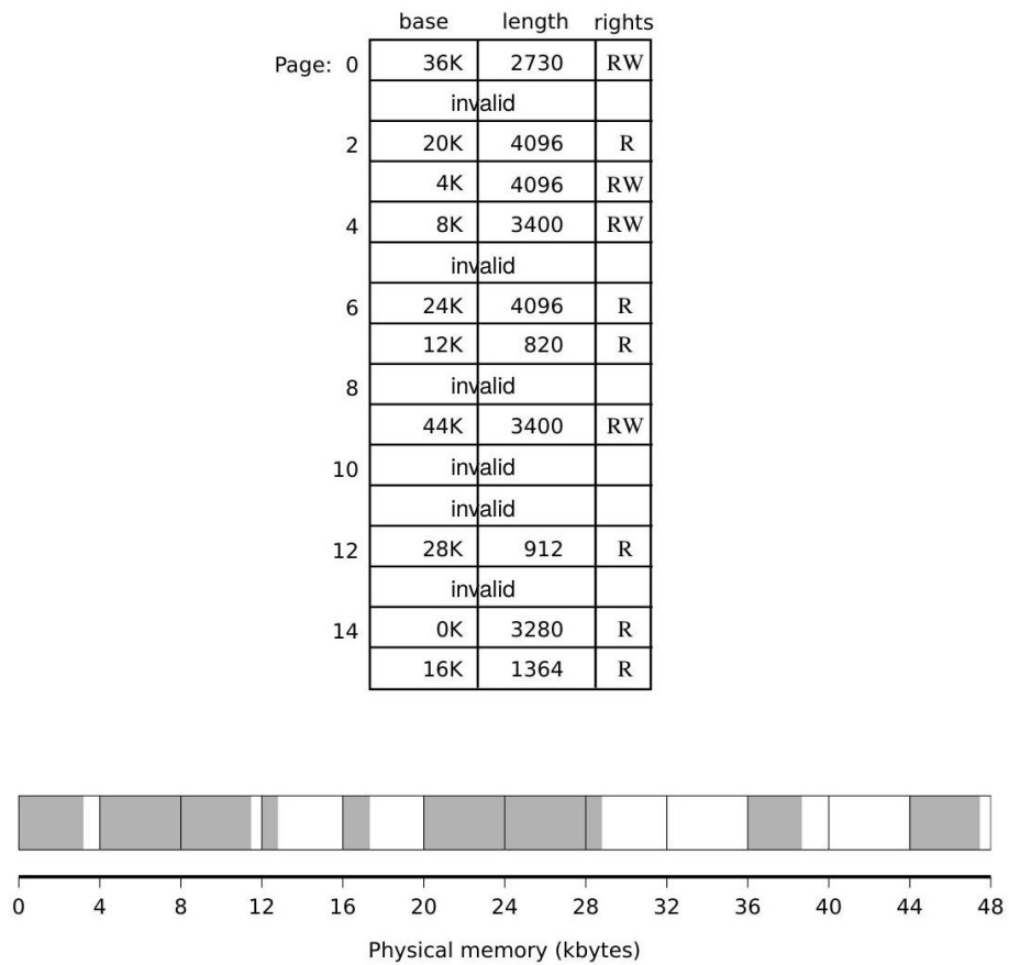
Fig. 115: A page table and the allocation of space in the memory which it corresponds to
