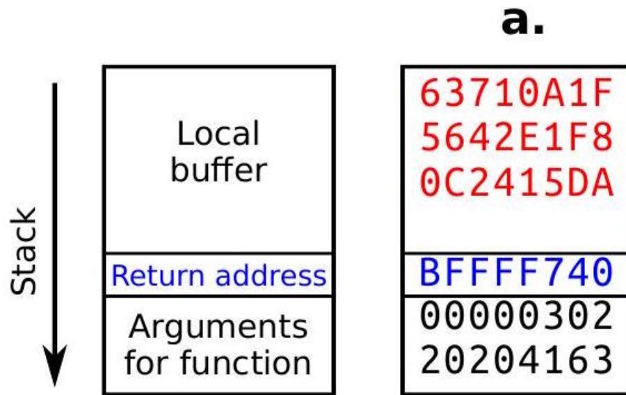
Fig. 120: Buffer Overflow
