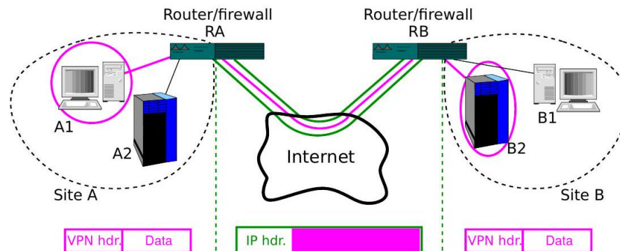
Fig. 77: Secure site-to-site tunneling in a VPN
