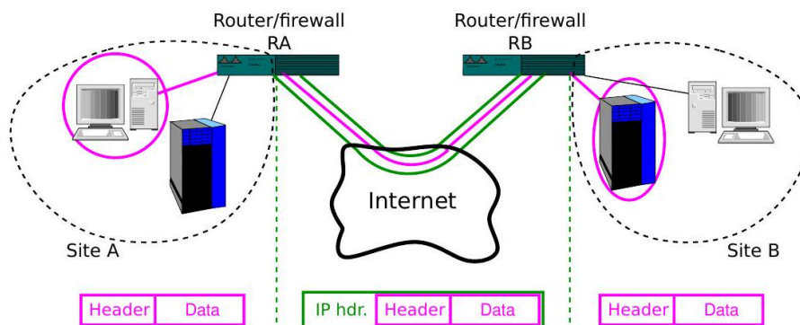
Fig. 76: Site-to-site tunneling
