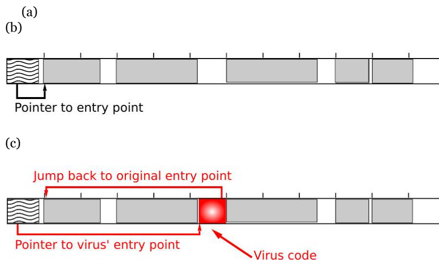
Fig. 123: Placement of virus code in an executable file.
