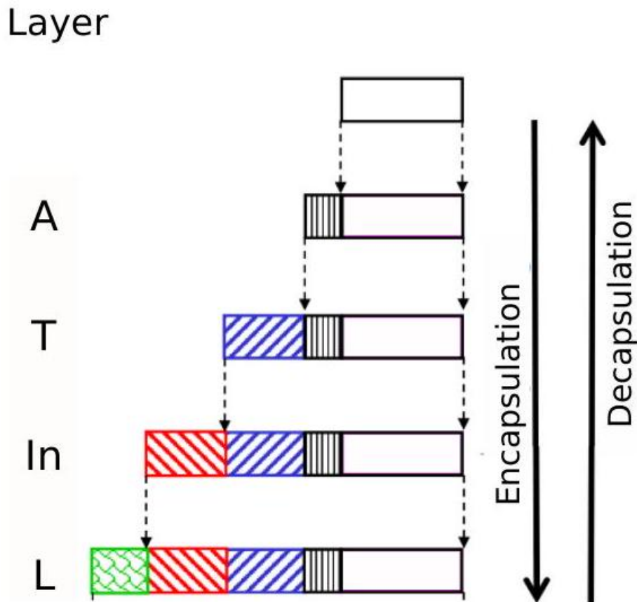
Fig. 69: Embedding of PDUs in a layered architecture
