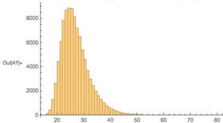
Figure 49: The distribution of longest hitting streaks, over 100,000 simulated careers. DiMaggio's actual 56 -game hitting streak stands at the very tail of this distribution, thus demonstrating the difficulty of this feat.
