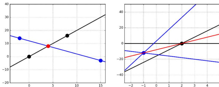
Figure 105: Points are equivalent to lines under a duality transform. The point (4, 8) in red (left) maps to the red line y = 4x - 8 on right. Both sets of three collinear points on the left correspond to three lines passing through the same point on right.
