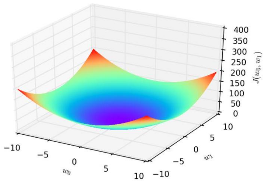
Figure 110: Linear regression defines a convex parameter space, where each point represents a possible line, and the minimum point defines the best fitting line.
