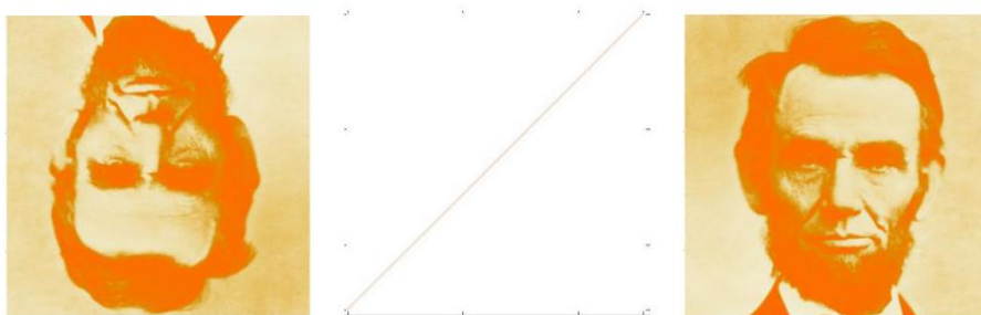
Figure 95: Multiplying a matrix by a permutation matrix rearranges its rows and columns.
