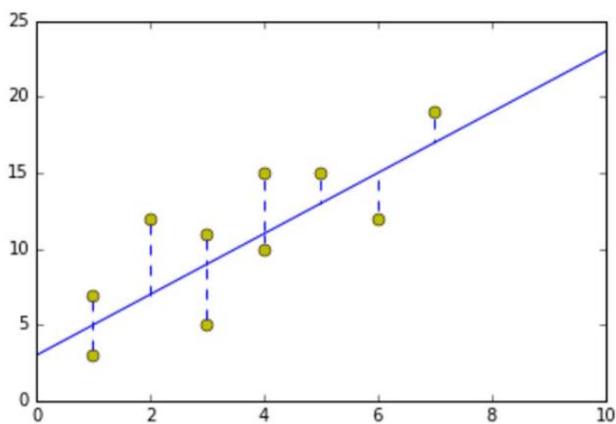
Figure 106: The residual error in least squares is the projection of y_i - f(X) down to X , not the shortest distance between the line and the point.
