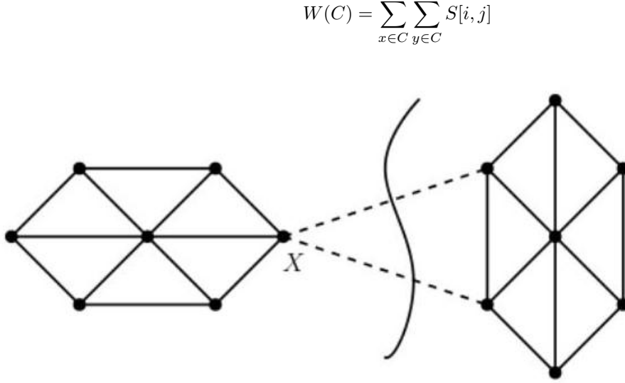
Figure 142: Low weight cuts in similarity graphs identify natural clusters.
