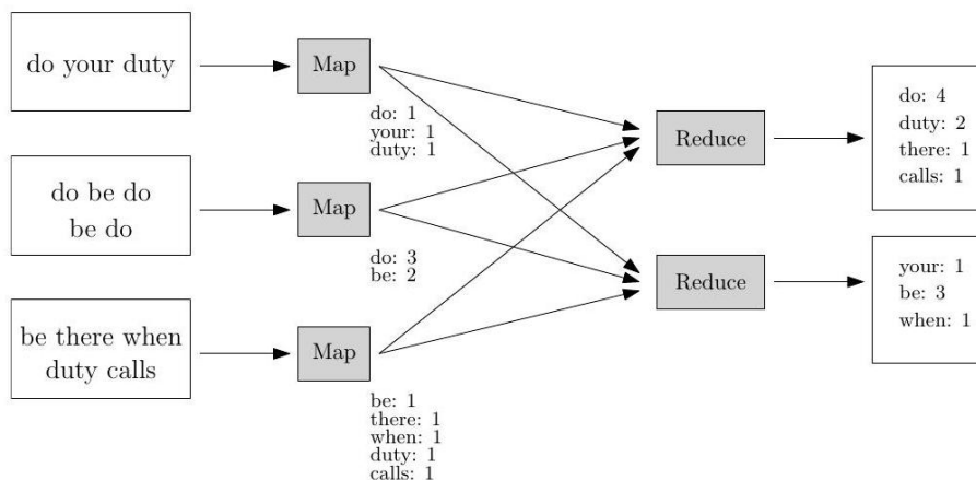
Figure 155: Word count in action. Count combination has been performed before mapping to reduce the size of the map files.
