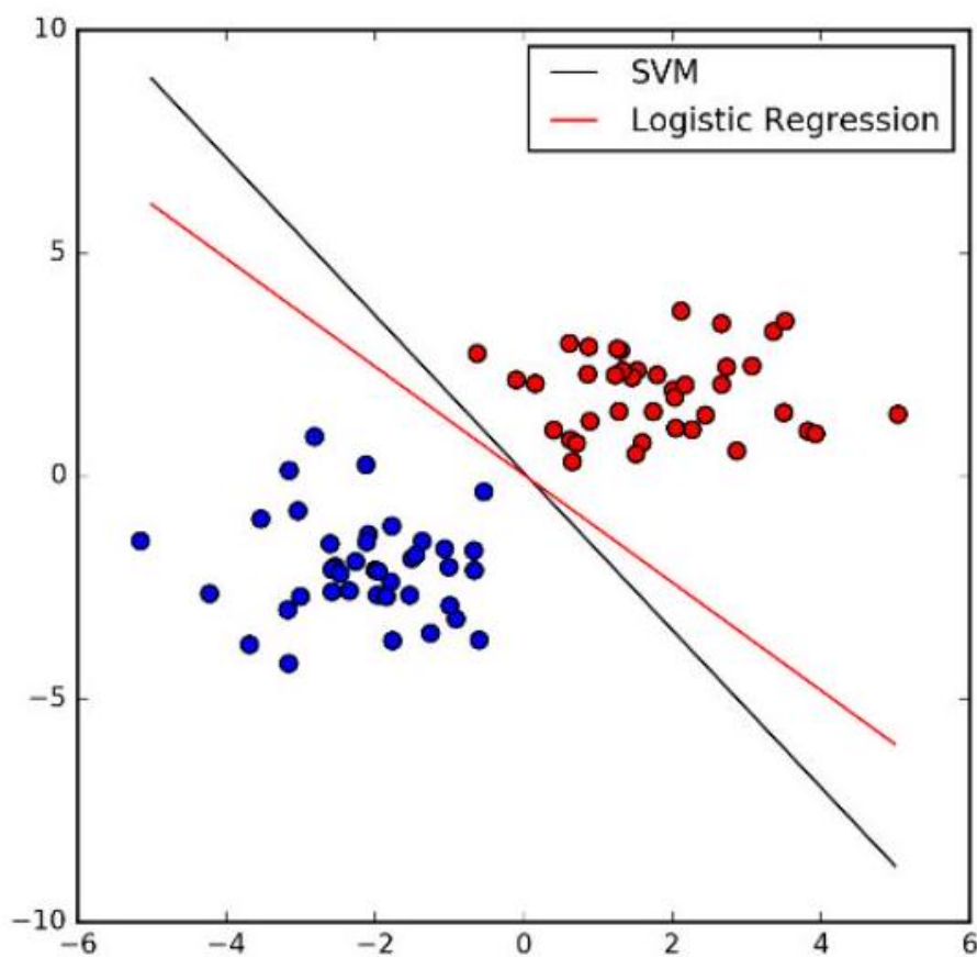
Figure 147: Both logistic regression and SVMs produce separating lines between point sets, but optimized for different criteria.
