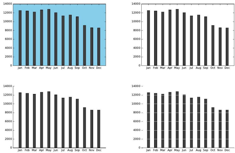
Figure 57: Four successive simplifications of Figure 6.7 by removing extraneous non-data elements.
