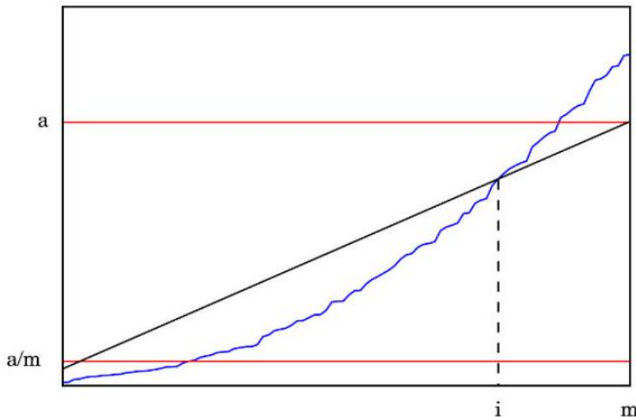
Figure 45: The Benjamini-Hochberg procedure minimizes false discovery rate, by accepting p -values only when p_i \leq \alpha i/m . The blue curve shows the sorted p values, and the diagonal defines the cutoff for when such a p -value is significant.
