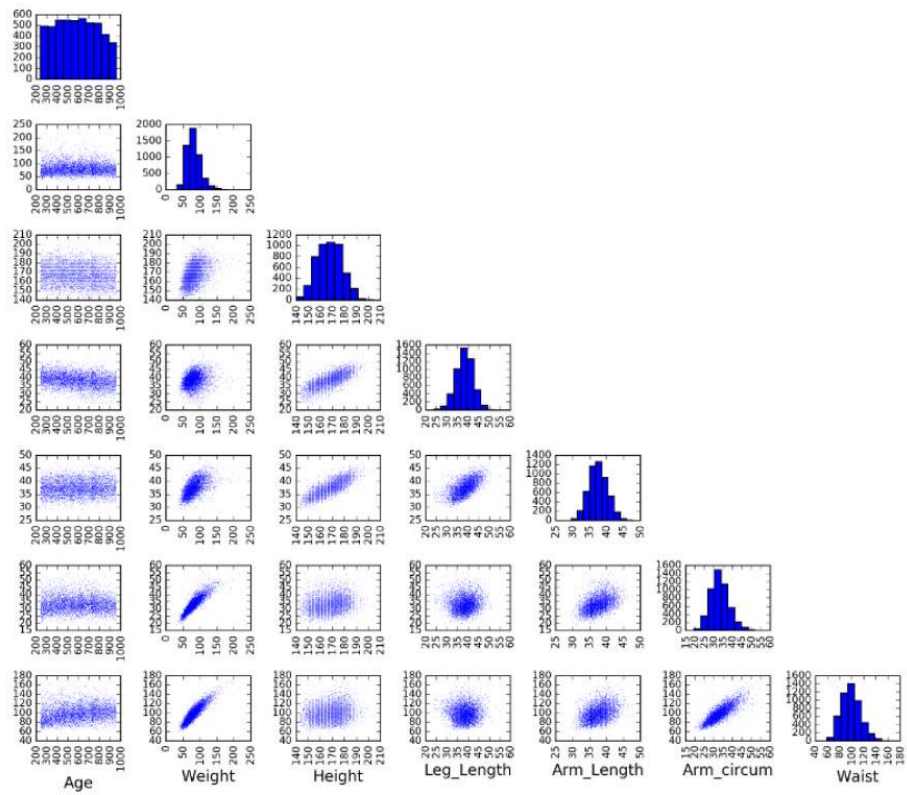
Figure 51: The array of dot plots of variable pairs provides quick insight into the distributions of data values and their correlations.
