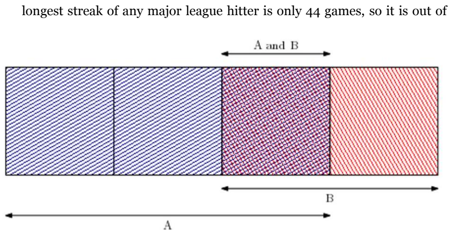
Figure 50: Bayes' Theorem in action.
