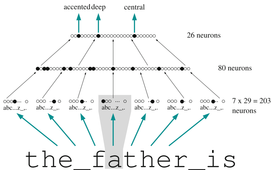
Fig. 9.21 The NETalk network maps a text to its pronunciation attributes
