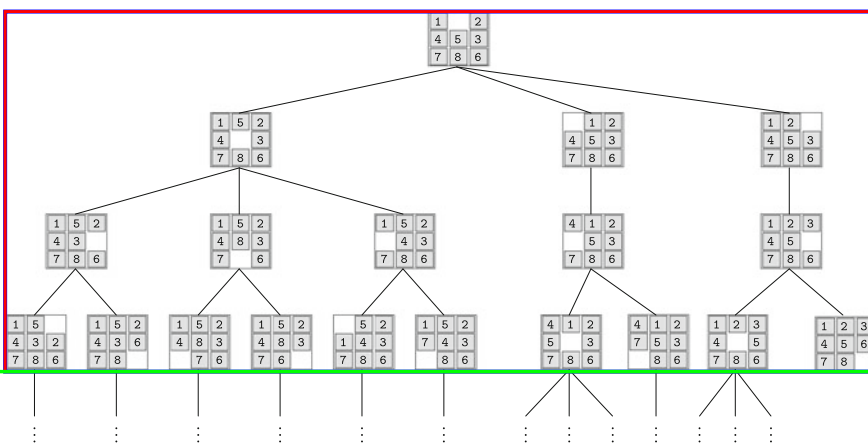
Fig. 6.4 Search tree for an 8-puzzle without cycles of length 2
