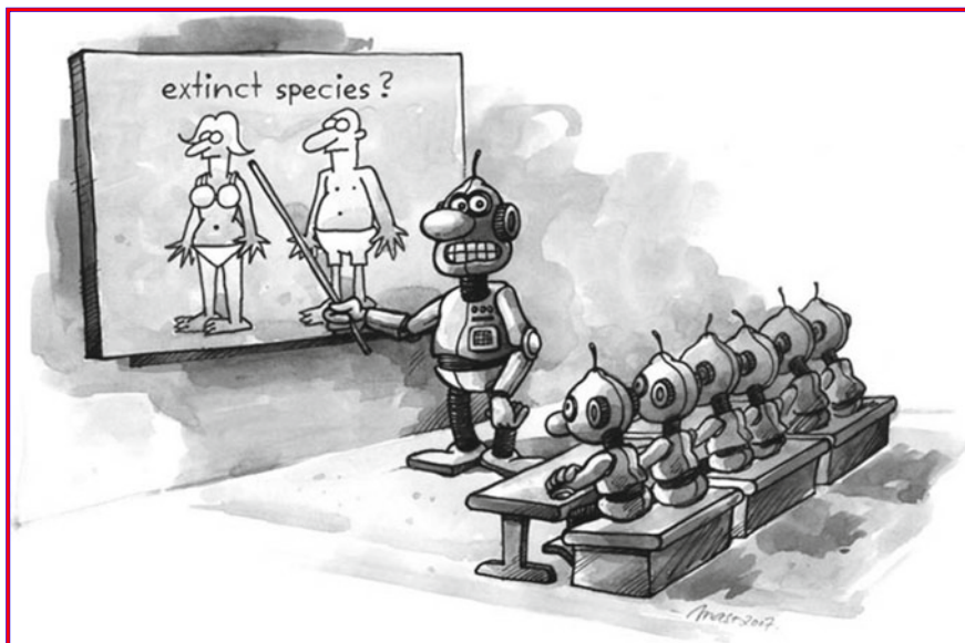
Fig. 8.1 Supervised learning ...
